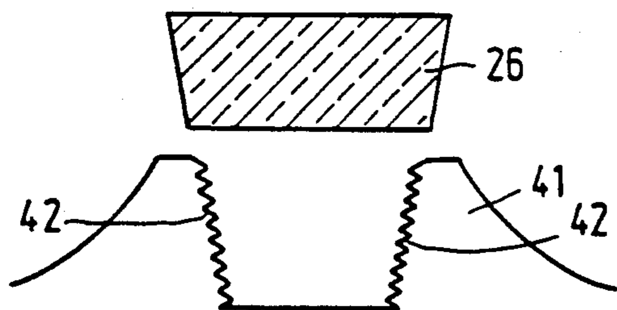
FIG. 3 PRIOR ART
