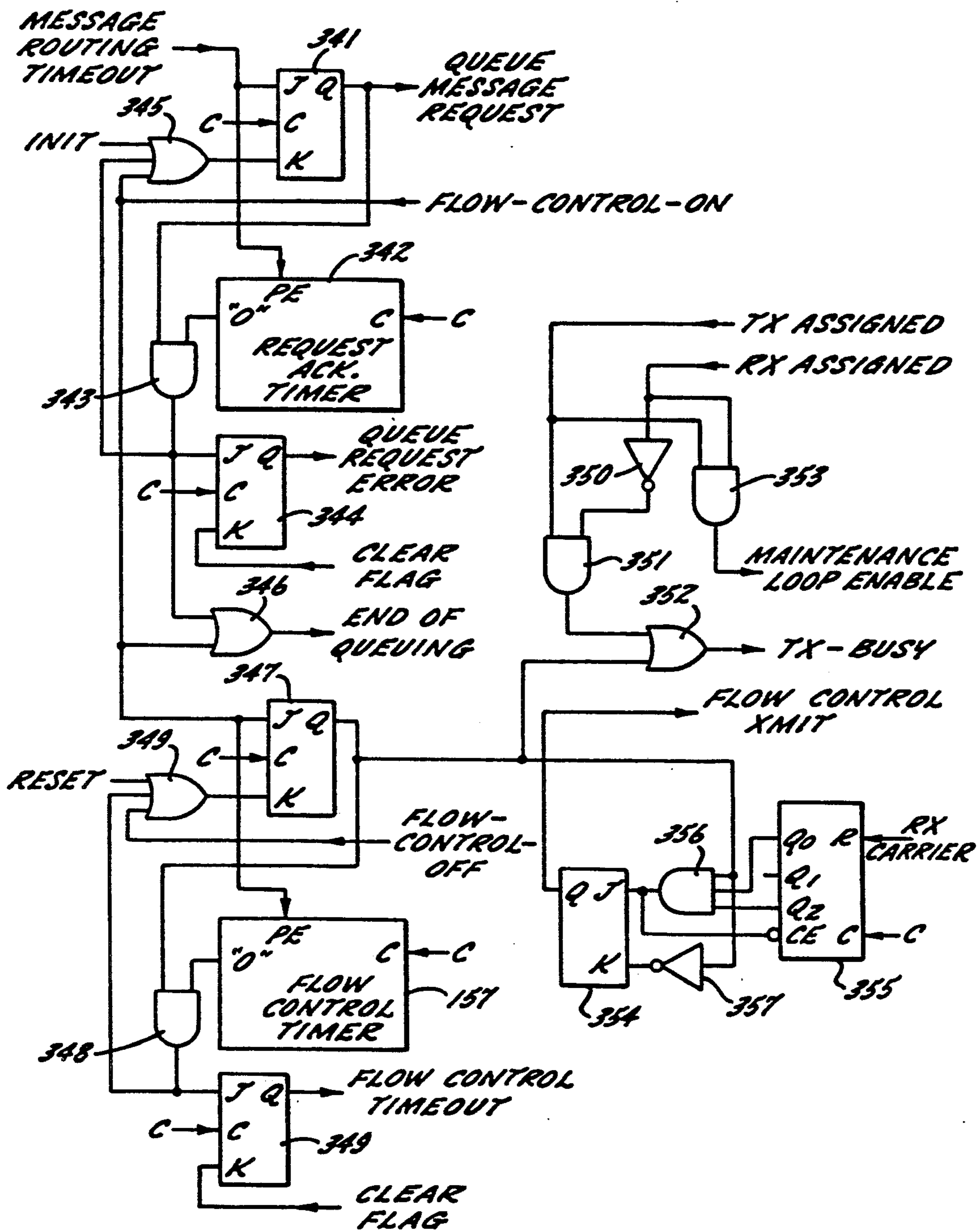
RX AND TX LOGIC FOR MESSAGE QUEUING
