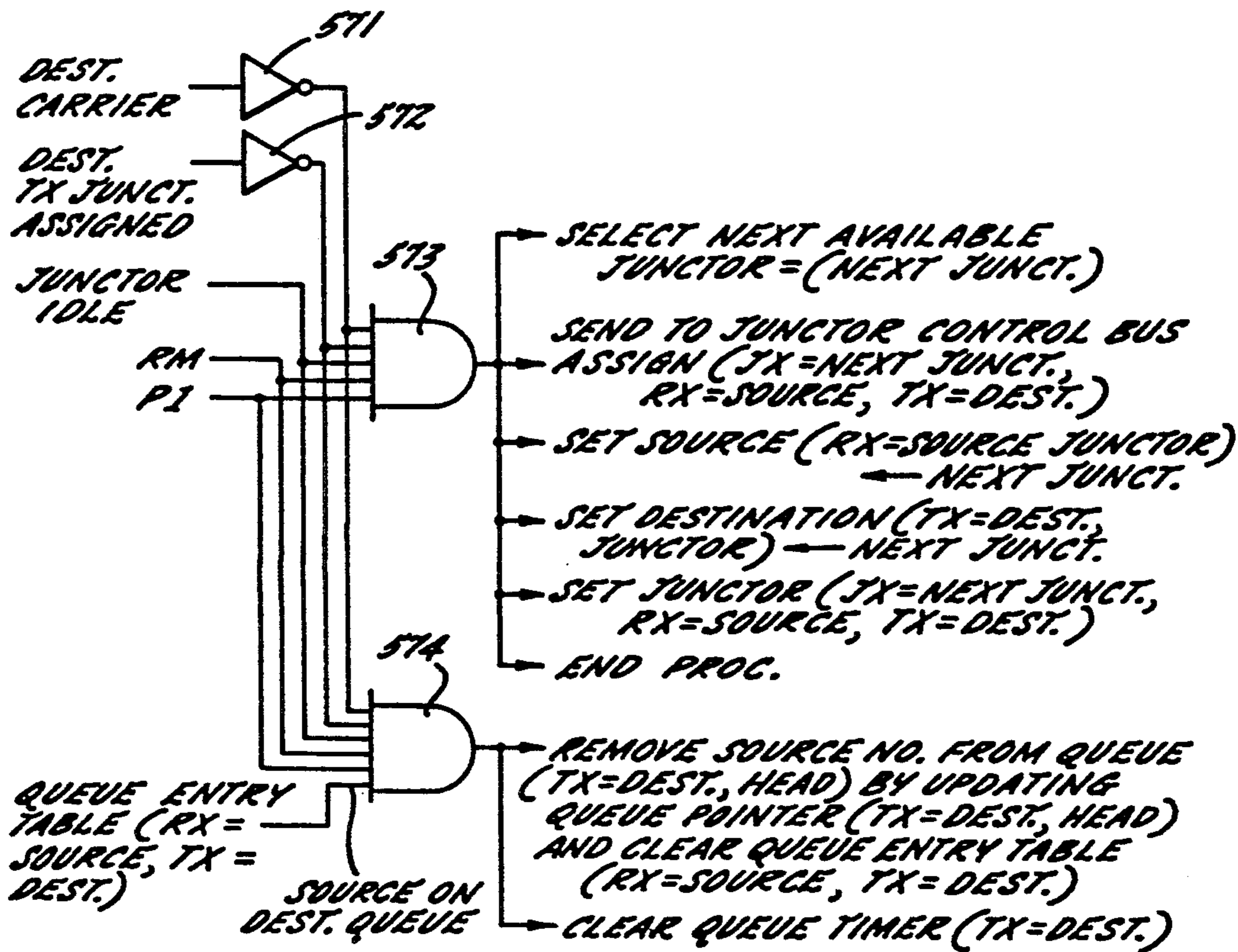
COMBINATIONAL LOGIC FOR ROUTING MESSAGE
