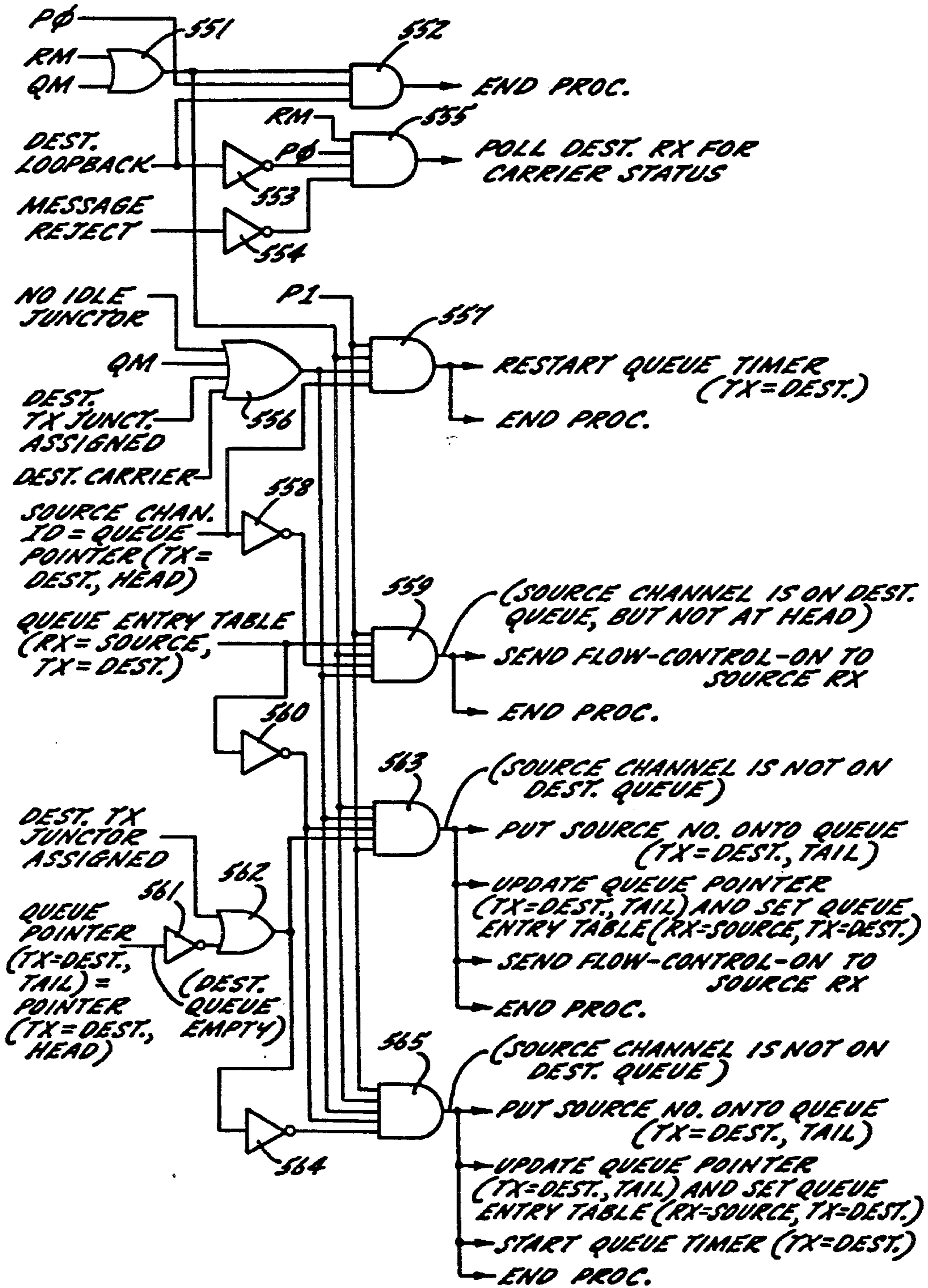
COMBINATIONAL LOGIC FOR MESSAGE QUEUING
