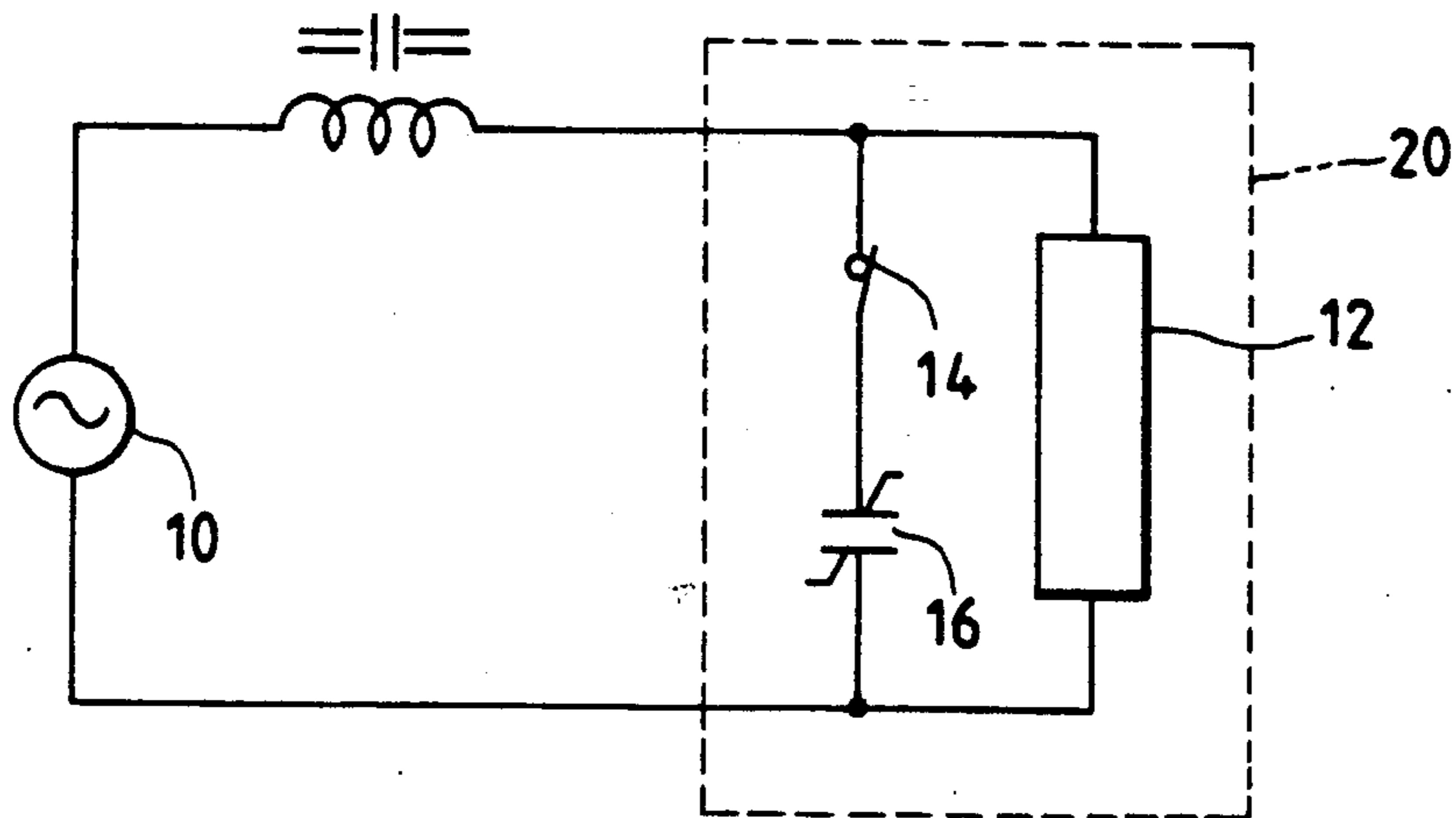
FIG. 1 PRIOR ART
