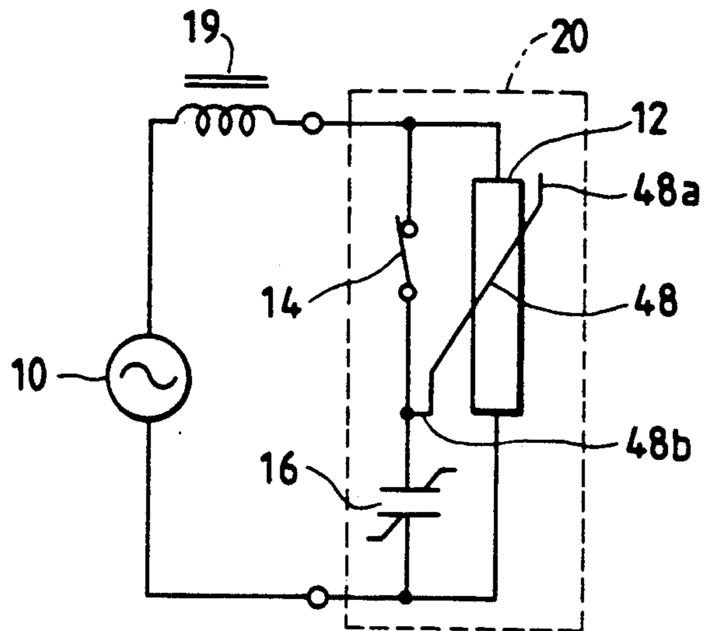
FIG. 3 PRIOR ART
