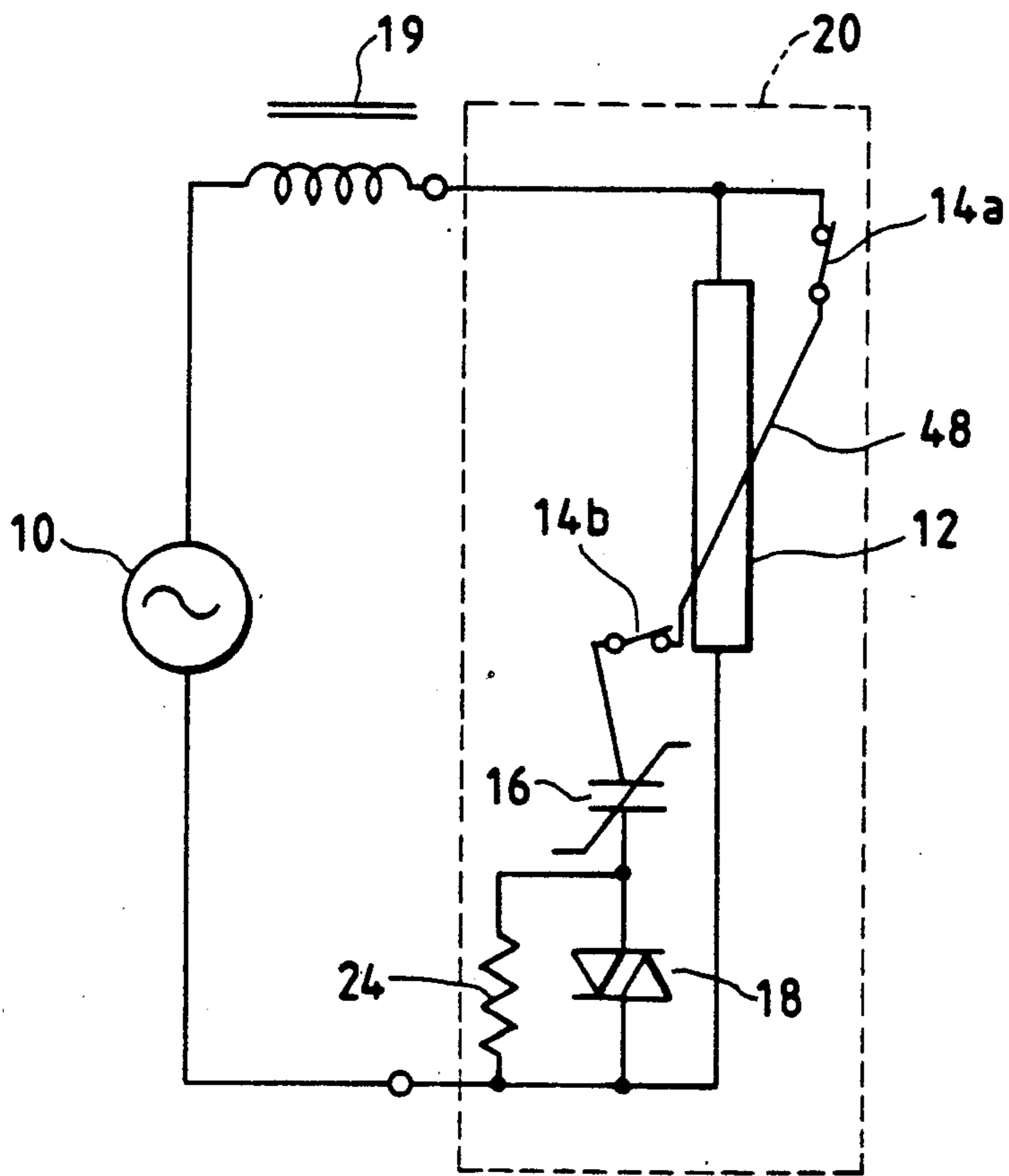
FIG. 4 PRIOR ART
