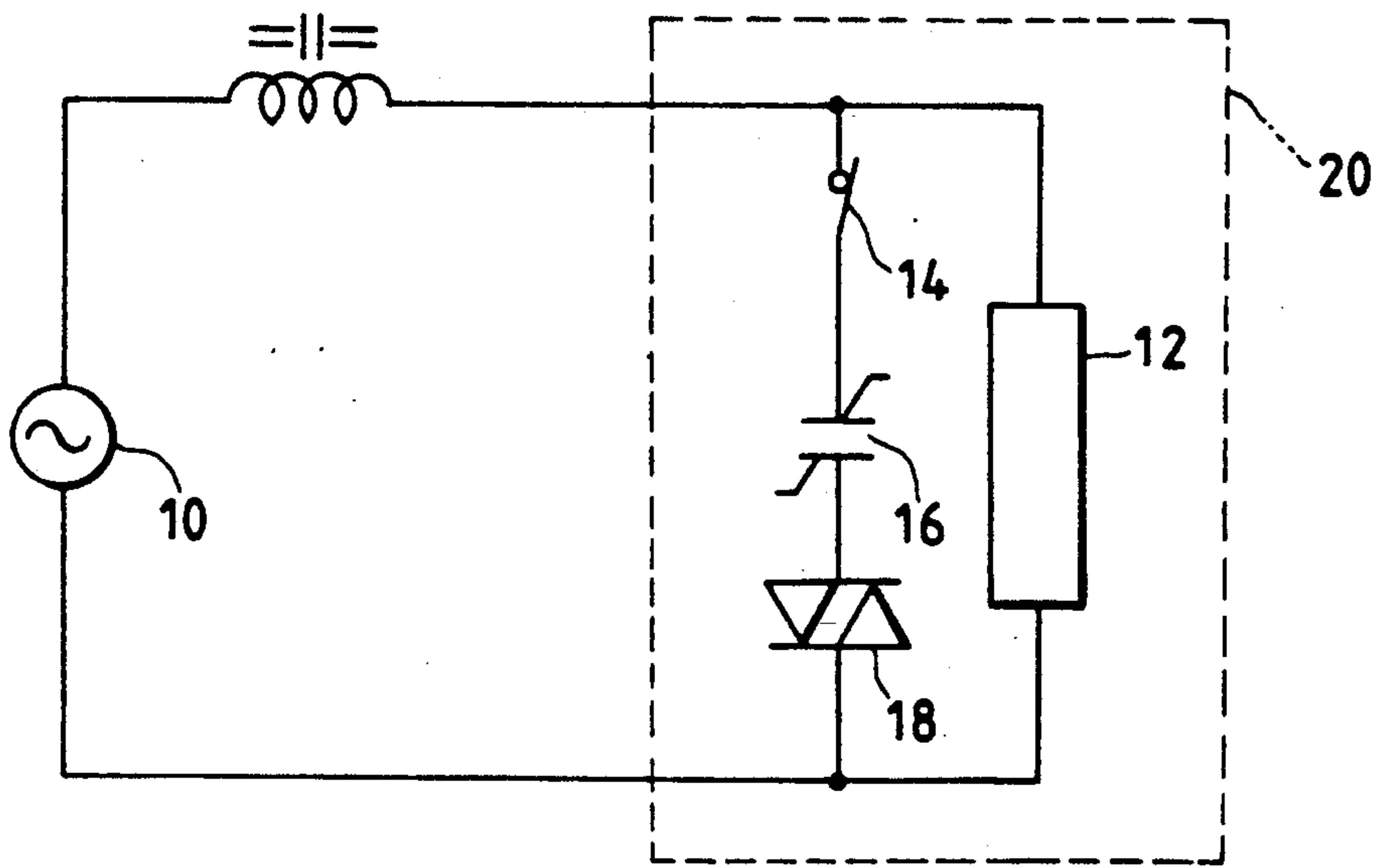
FIG. 2 PRIOR ART
