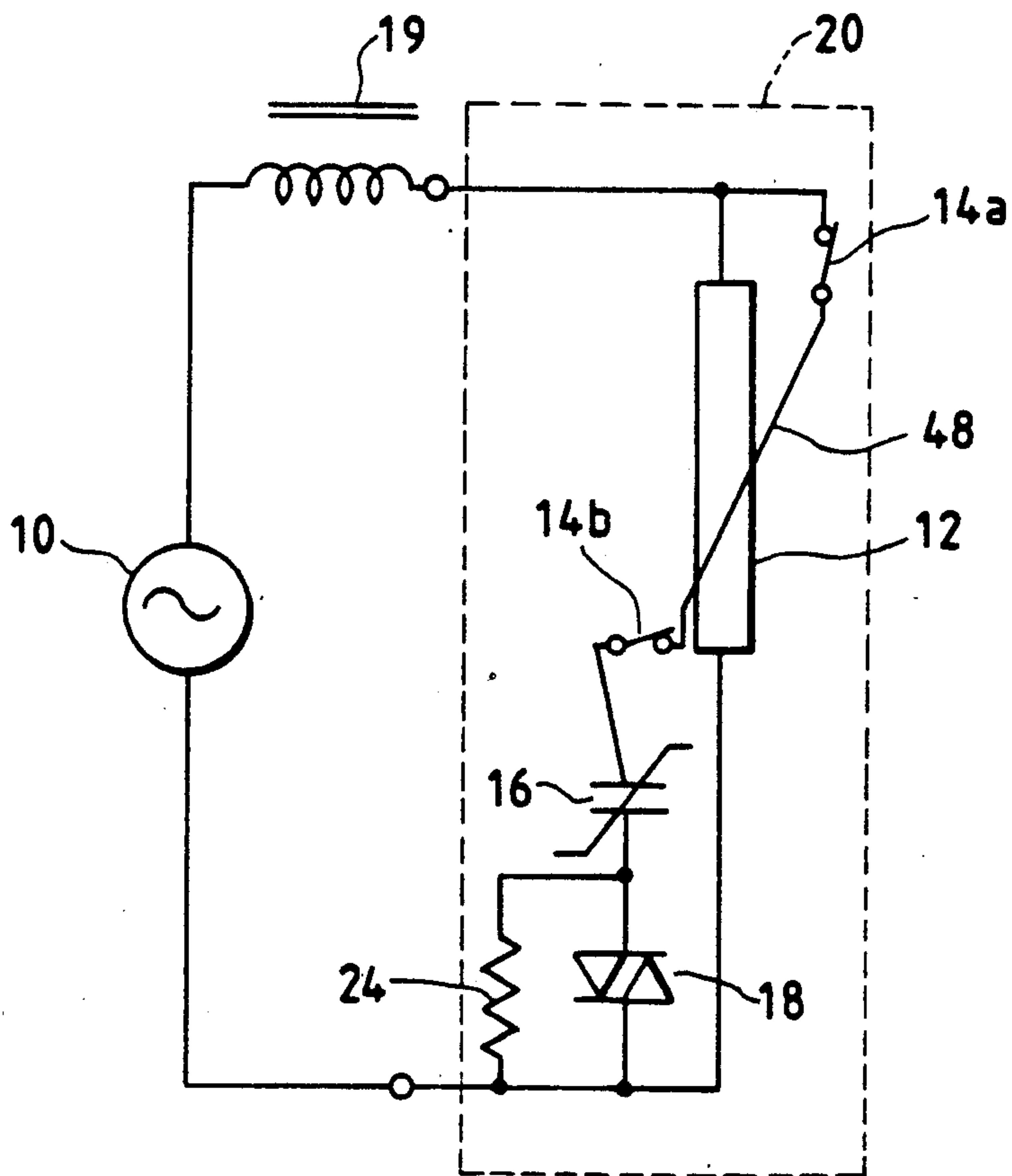
FIG. 4 PRIOR ART
