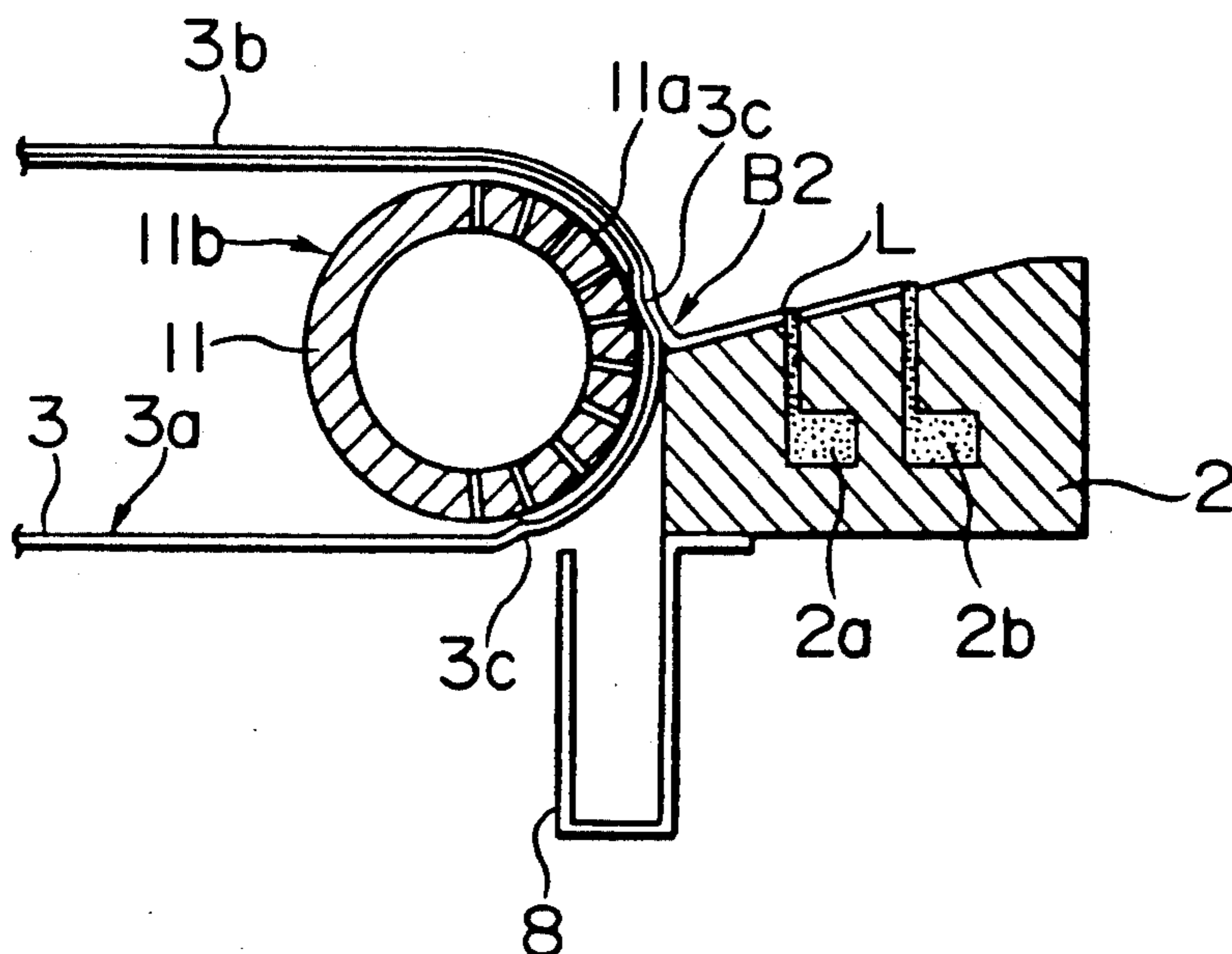
FIG. 8 PRIOR ART
