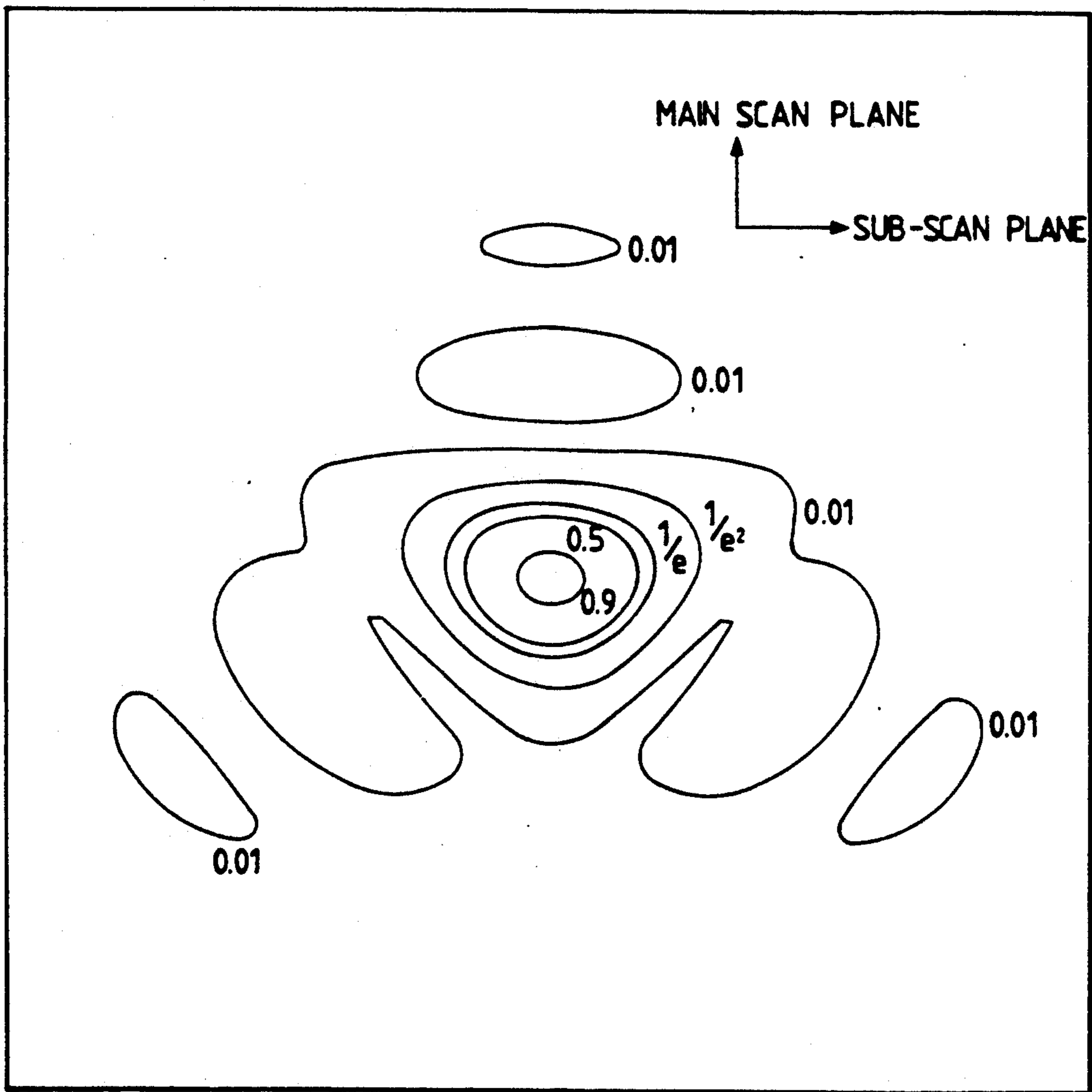
FIG. 4 PRIOR ART
