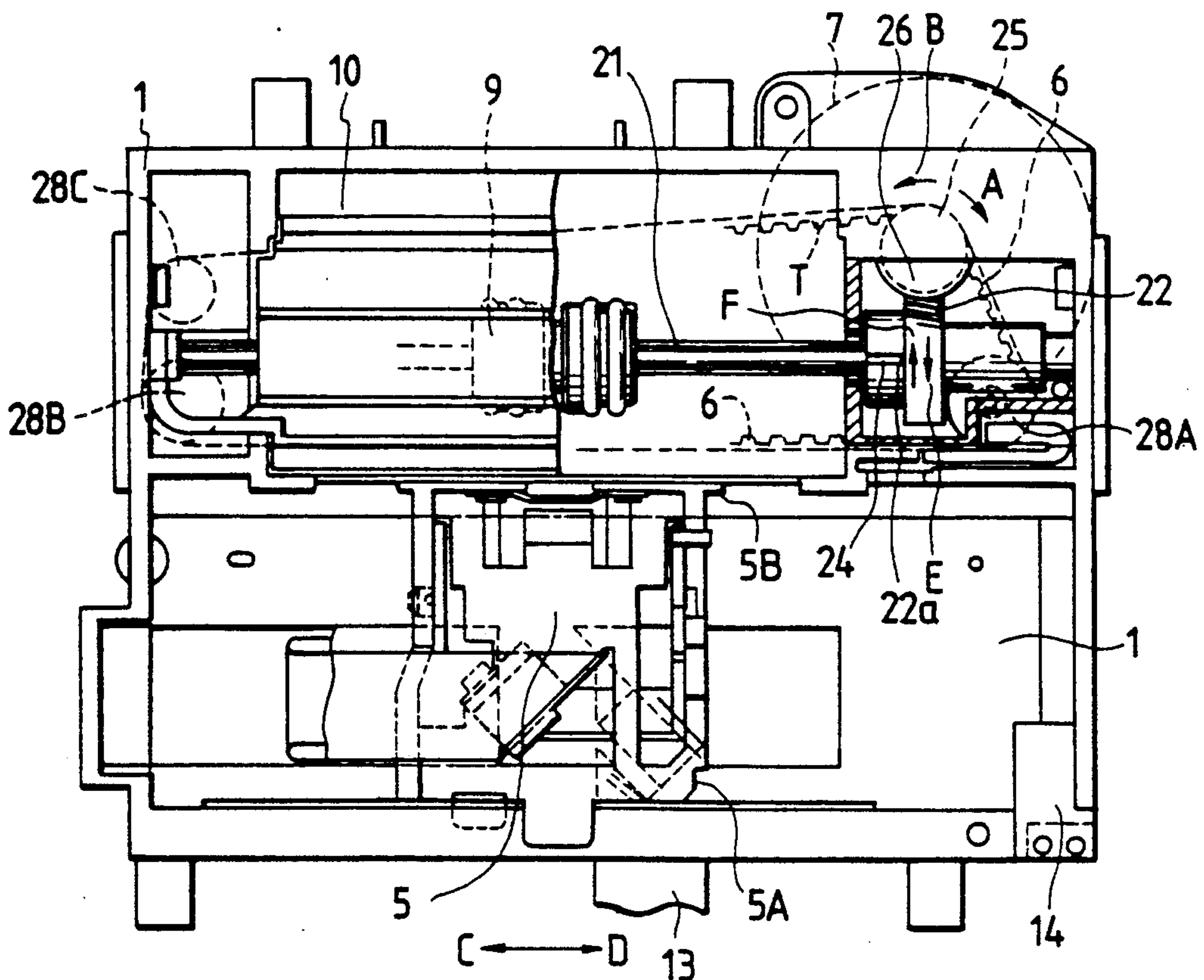
FIG. 4 PRIOR ART
