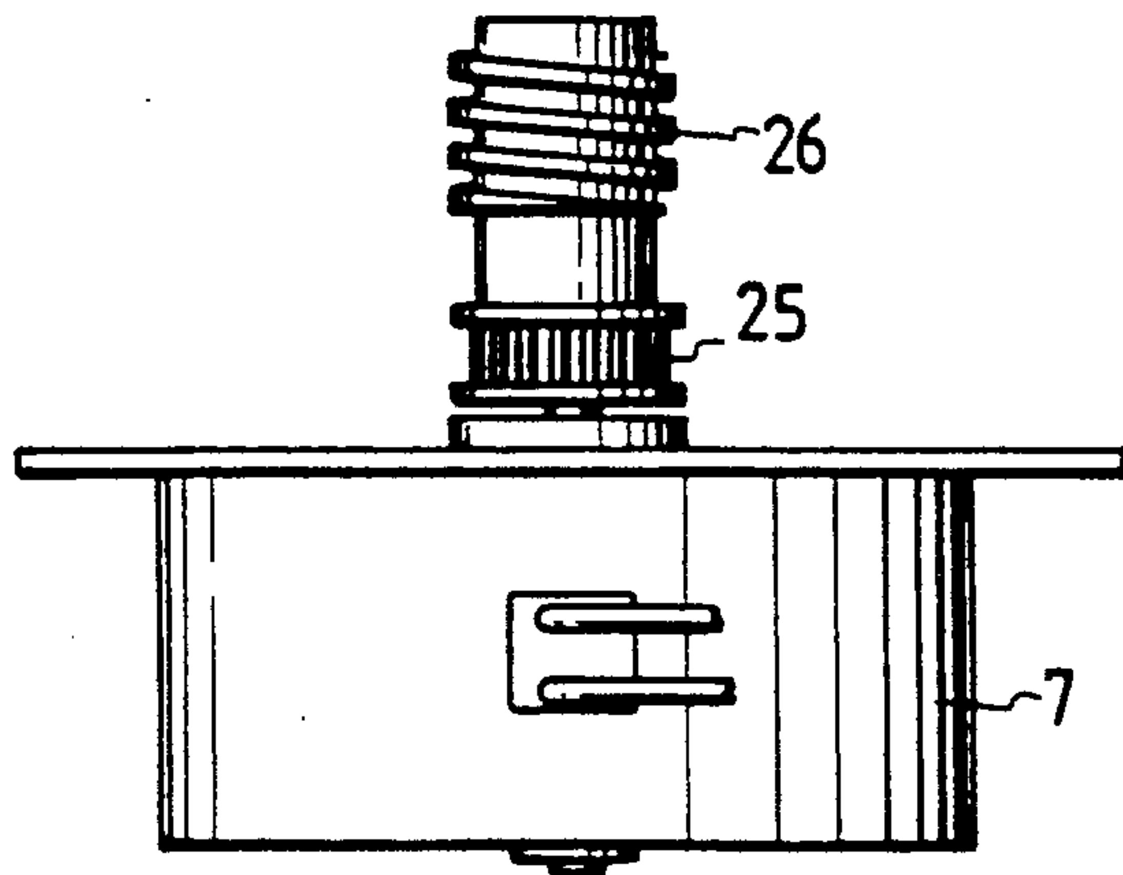
FIG. 6 PRIOR ART
