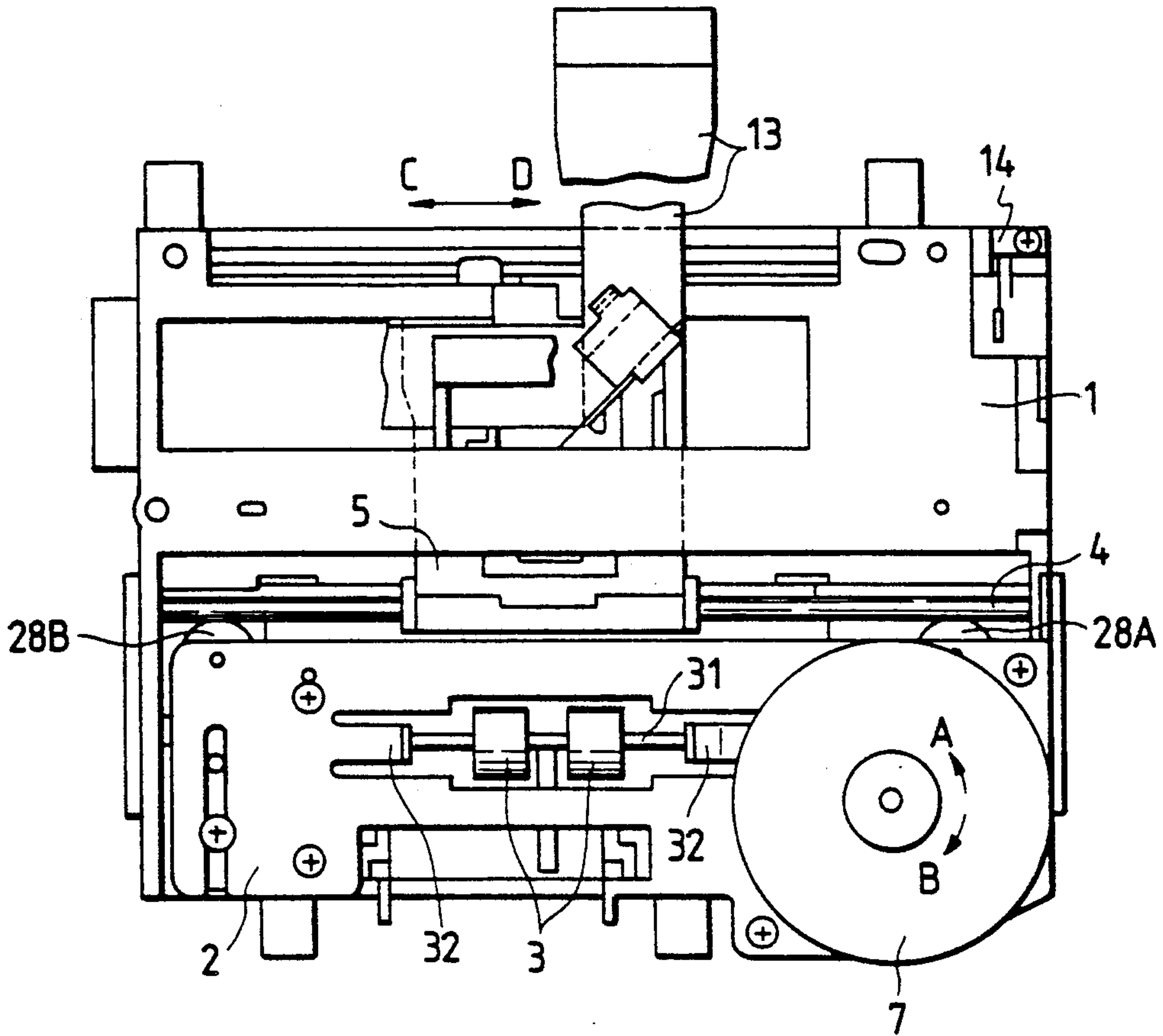
FIG. 5 PRIOR ART
