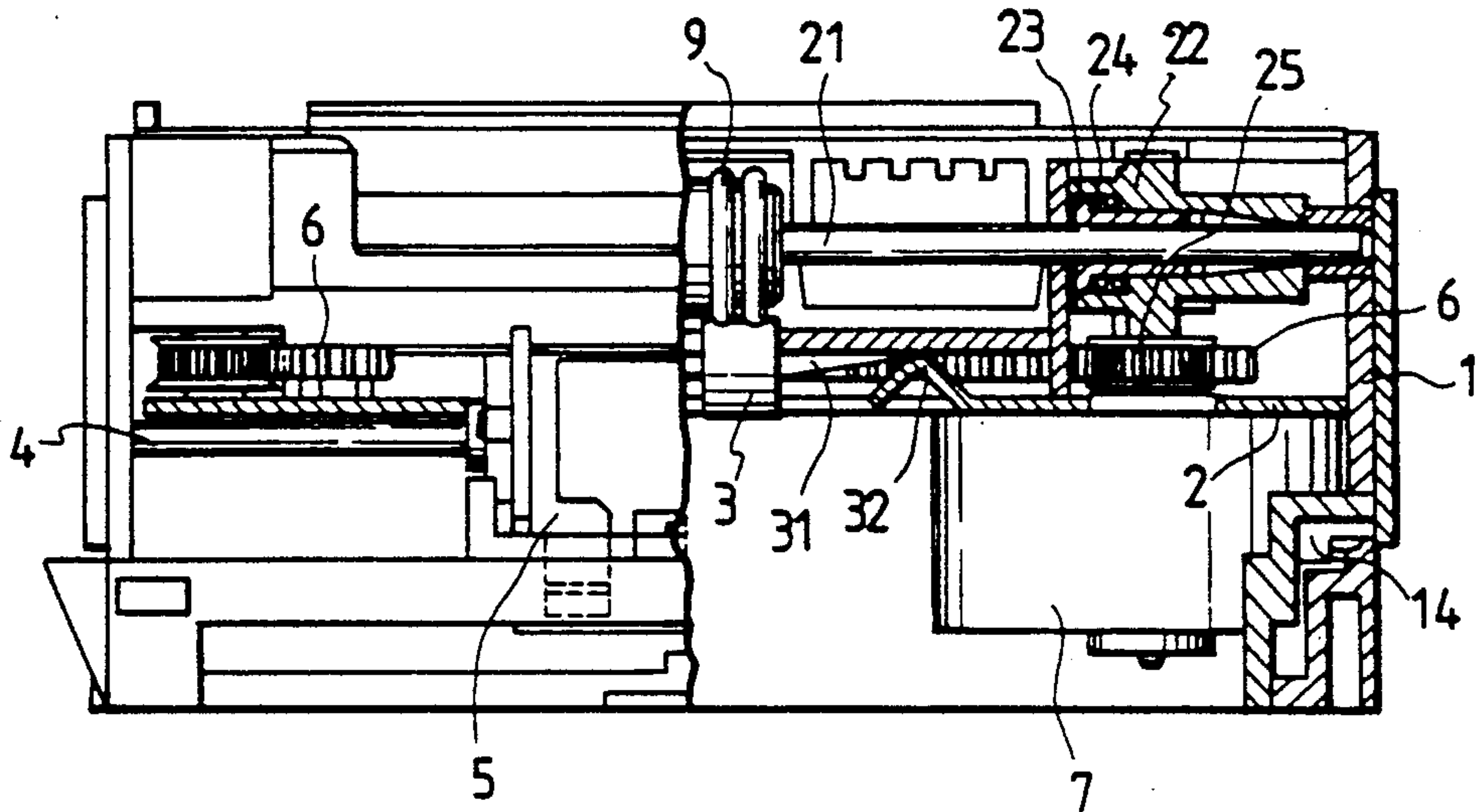
FIG. 3 PRIOR ART
