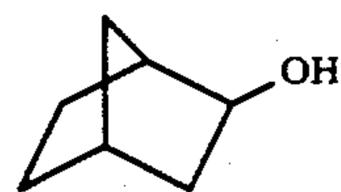
exo-norborneol
