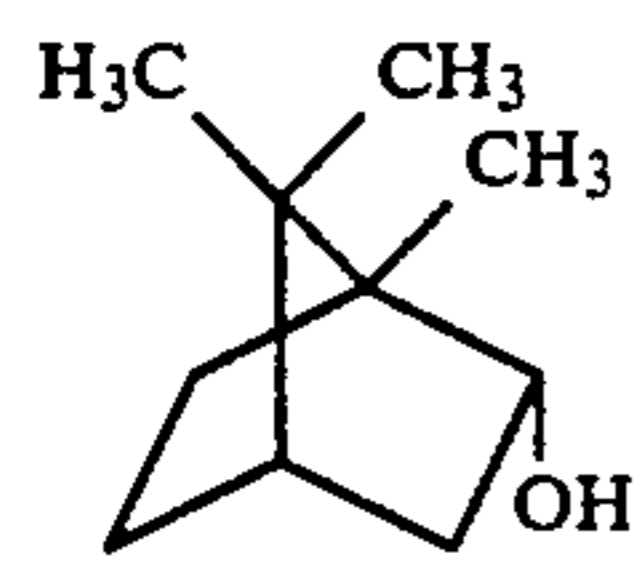
[(1S)-endo]-(-)-borneol
