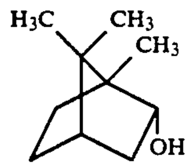
[(1S)-endo]-(-)-borneol
