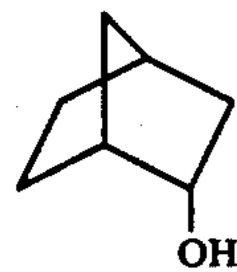
endo-norborneol
