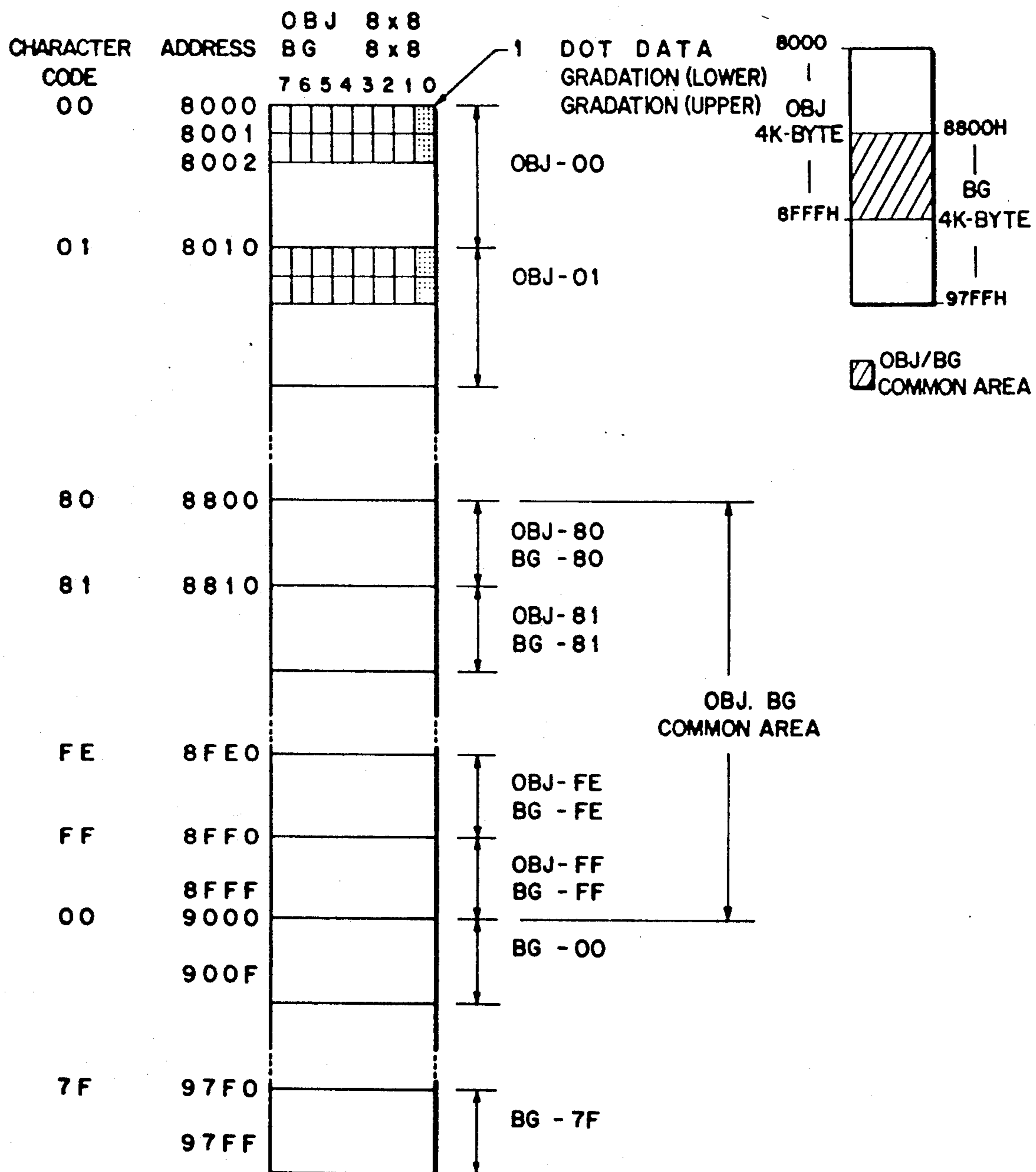
FIG. 13 CHARACTER RAM
