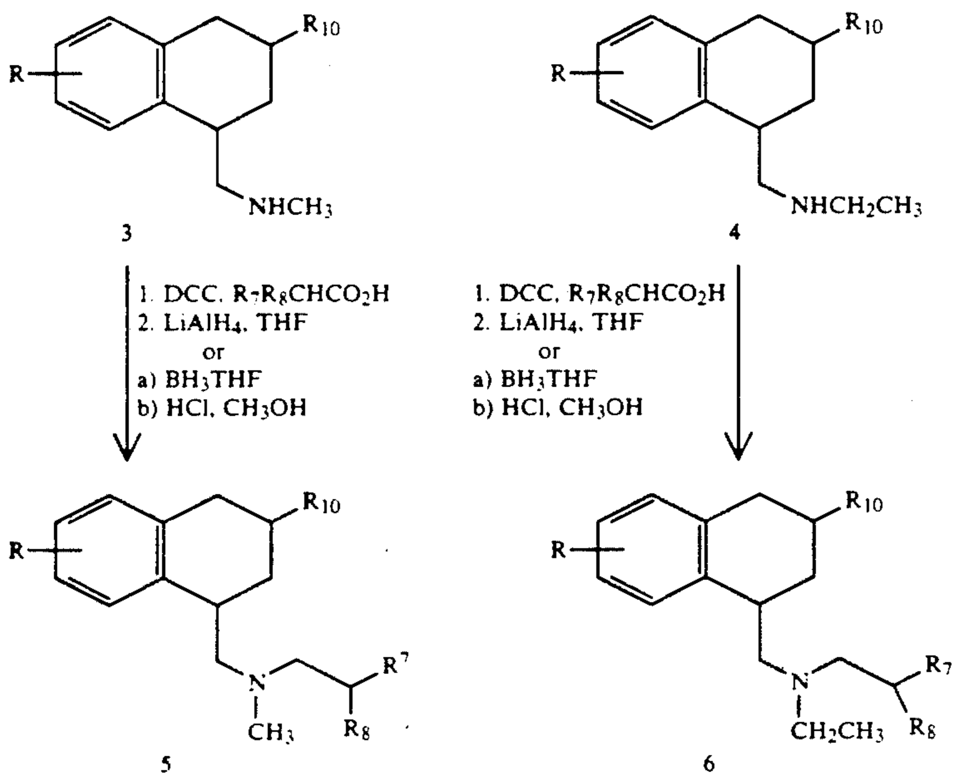
Scheme 2
