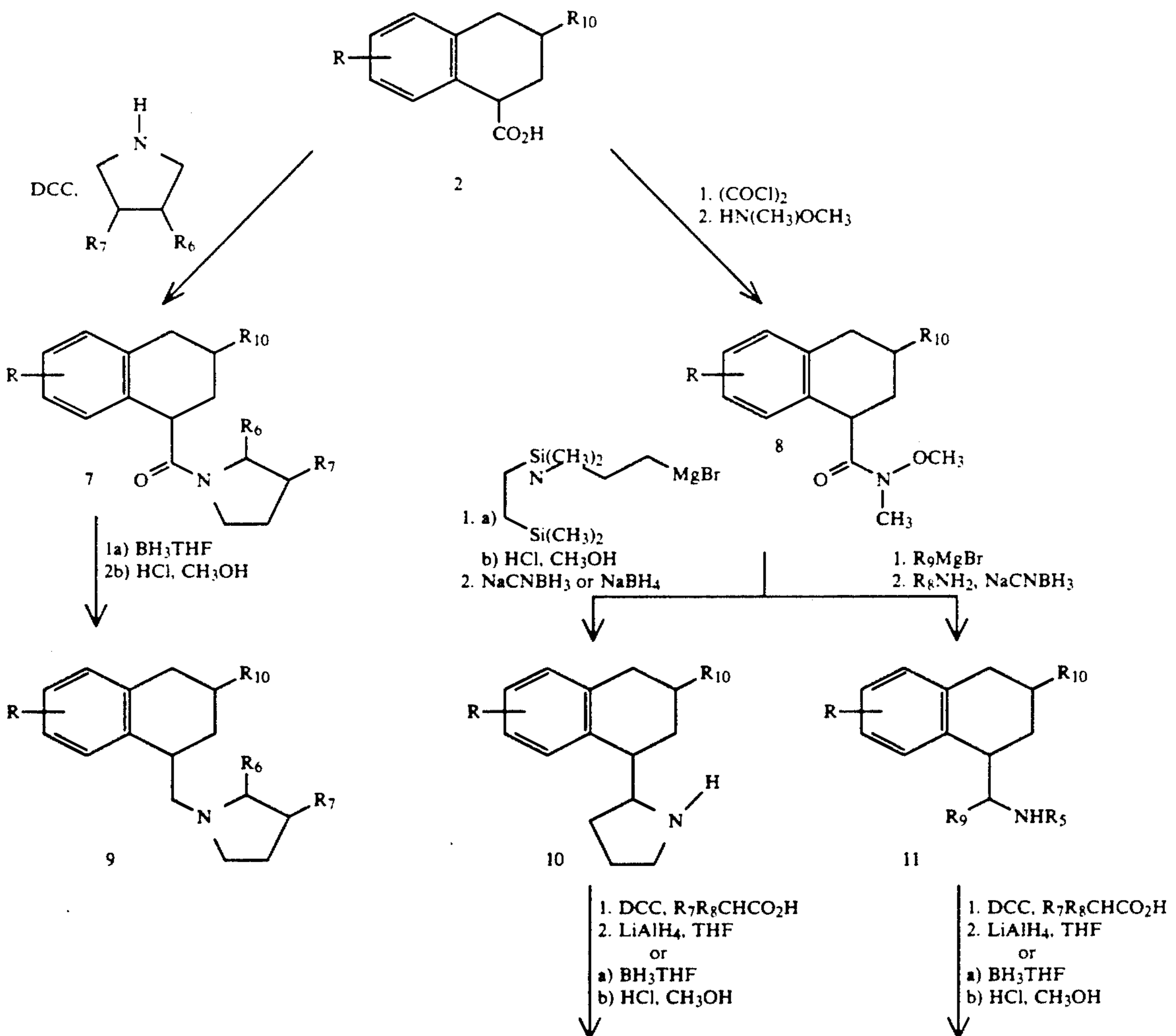
Scheme 3
