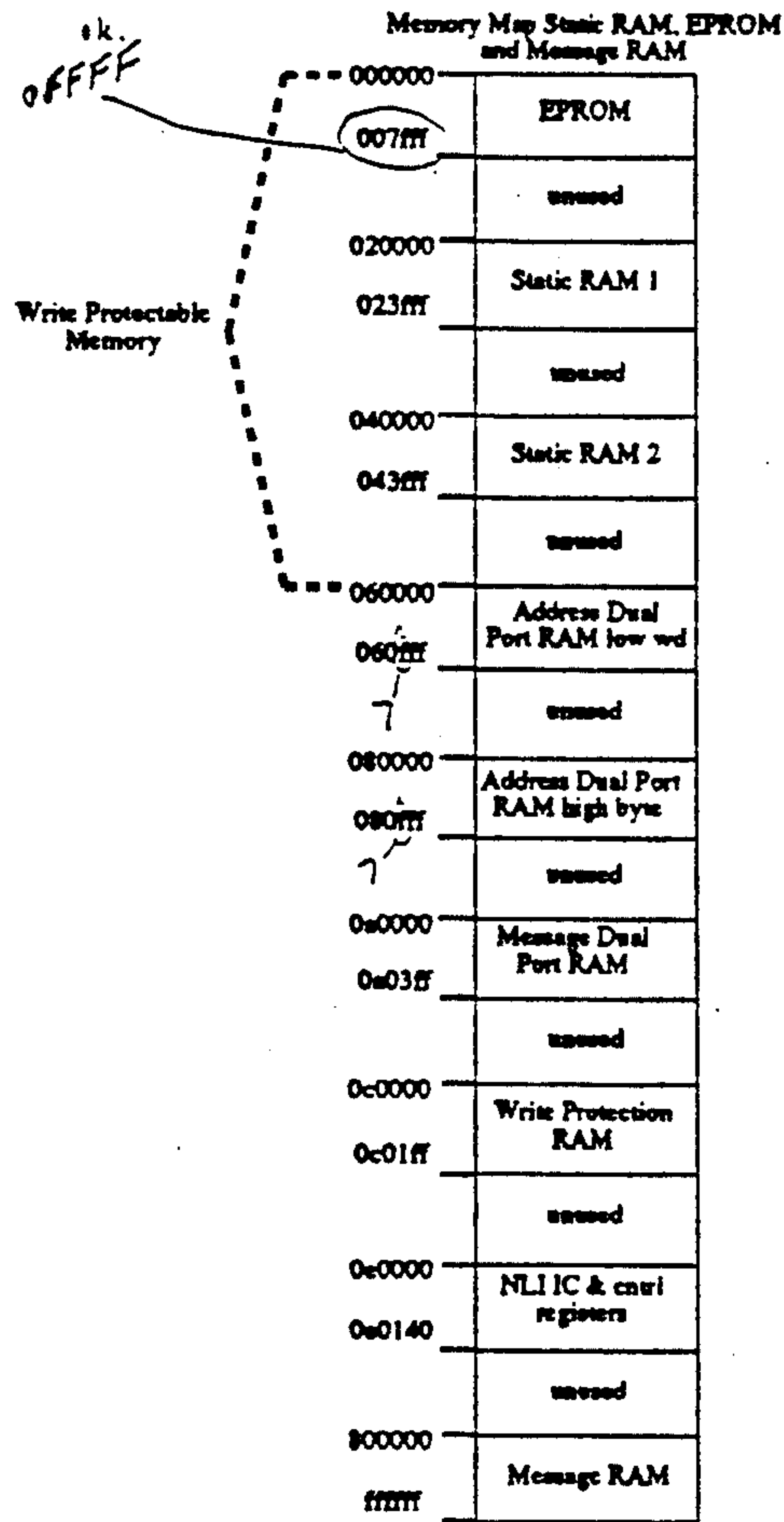
Figure 10. Memory Map for DAS
