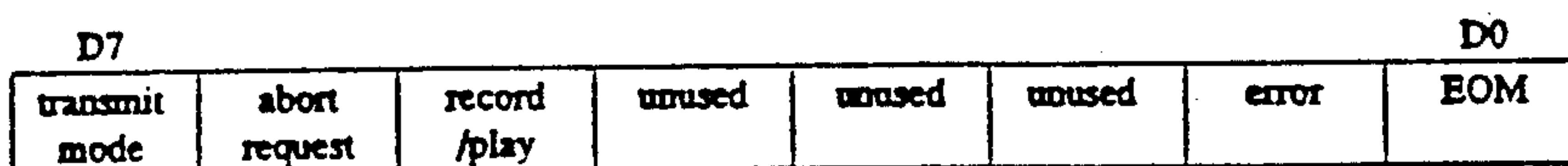
Figure 16. Channel Control Table Layout
