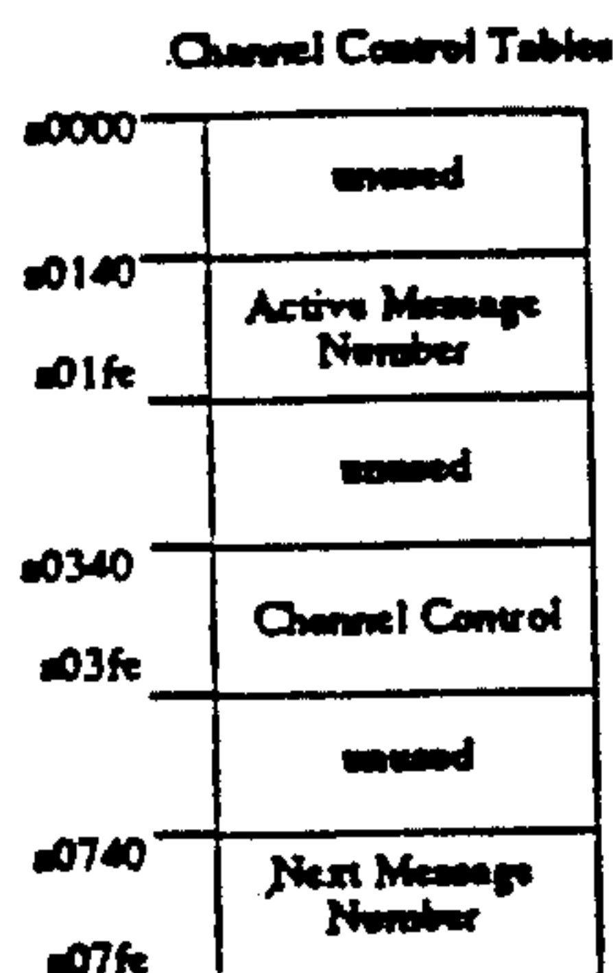
Figure 16. Channel Control Table Layout
