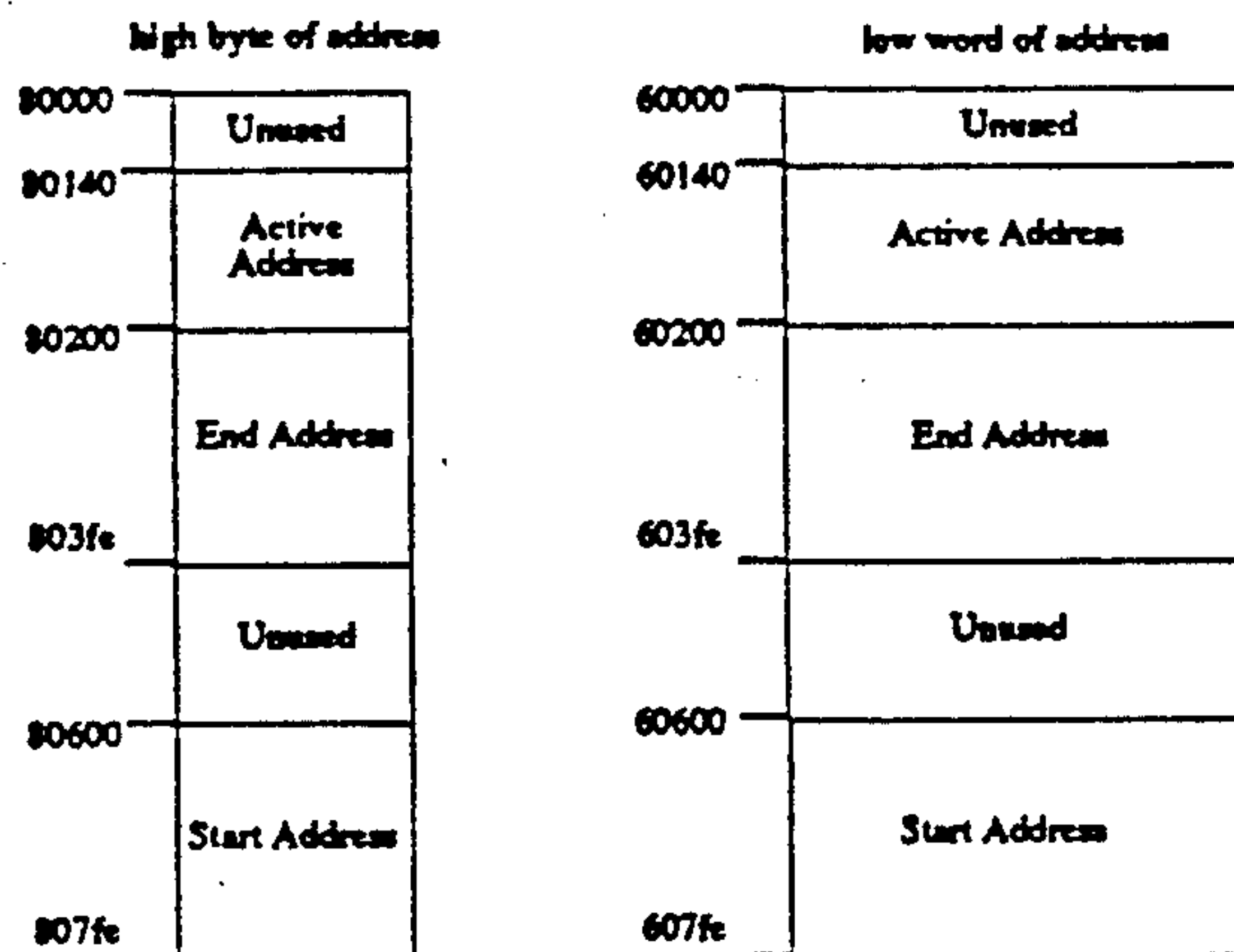
Figure 13. Message Address Pointer Table Layout
