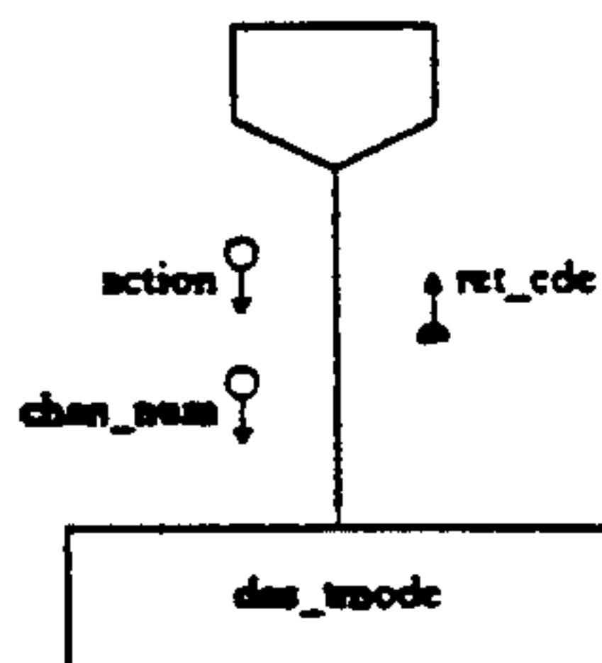
Figure 21. Set Transmit Mode Primitive
