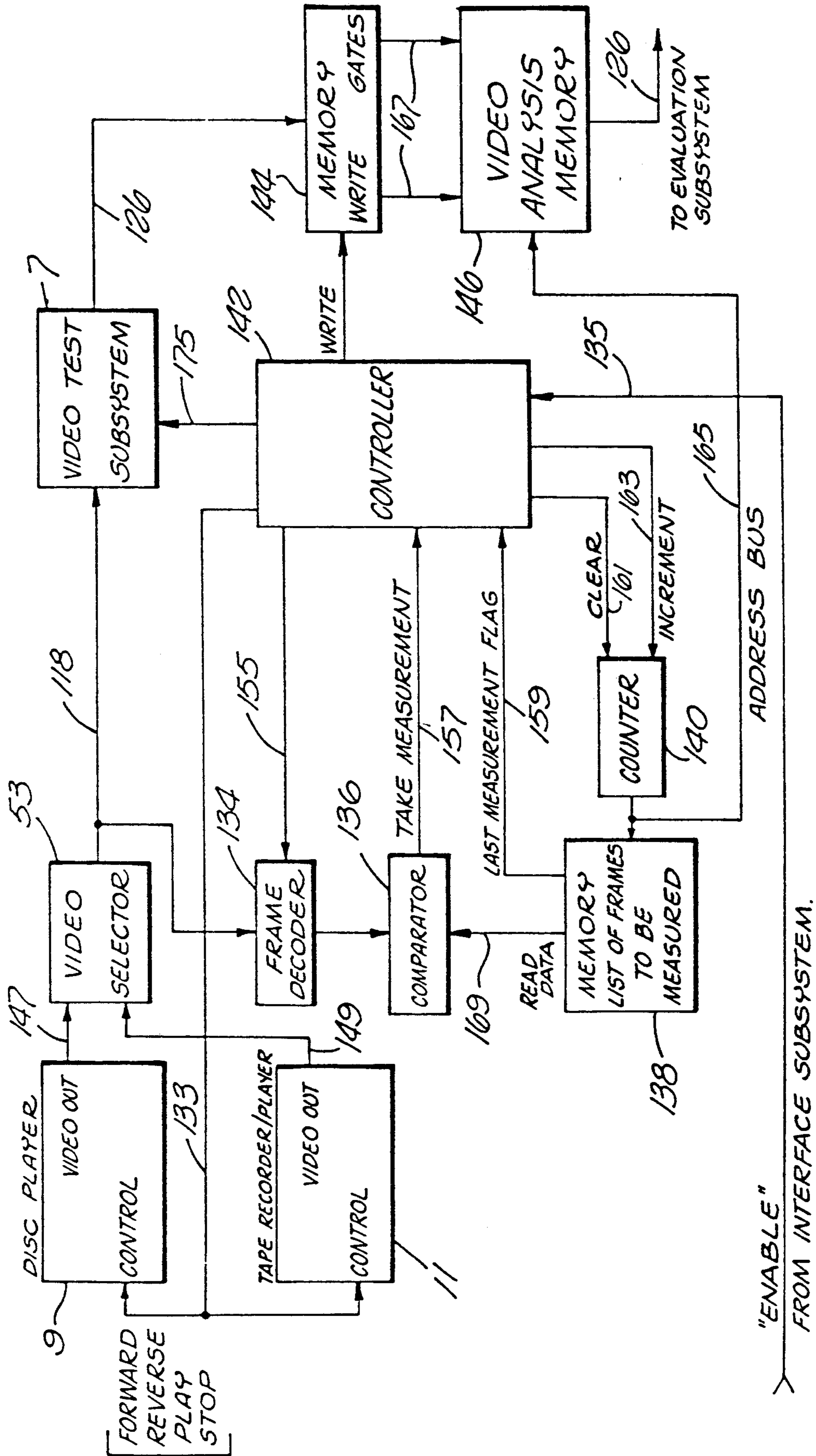
FIG. 22 VIDEO ANALYSIS LOGIC
