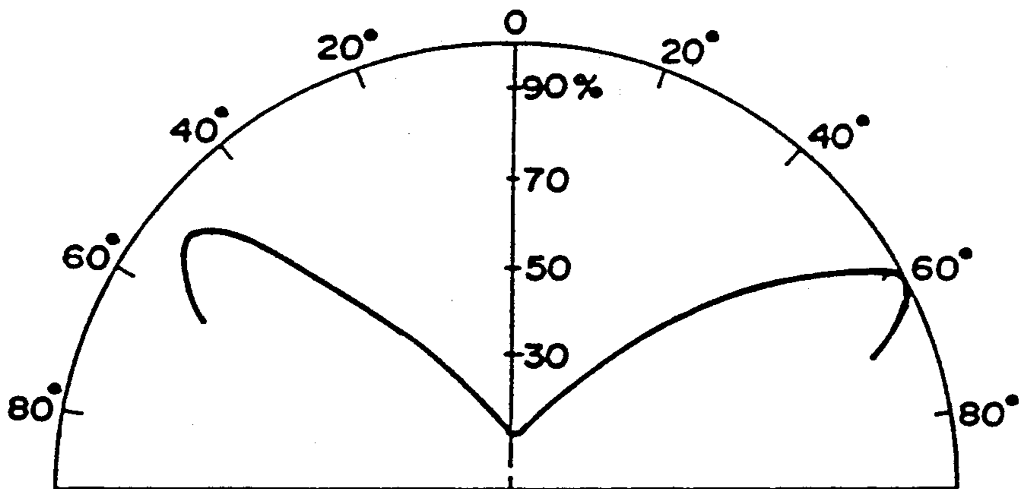
Anisotropic Lenticular Lens A
