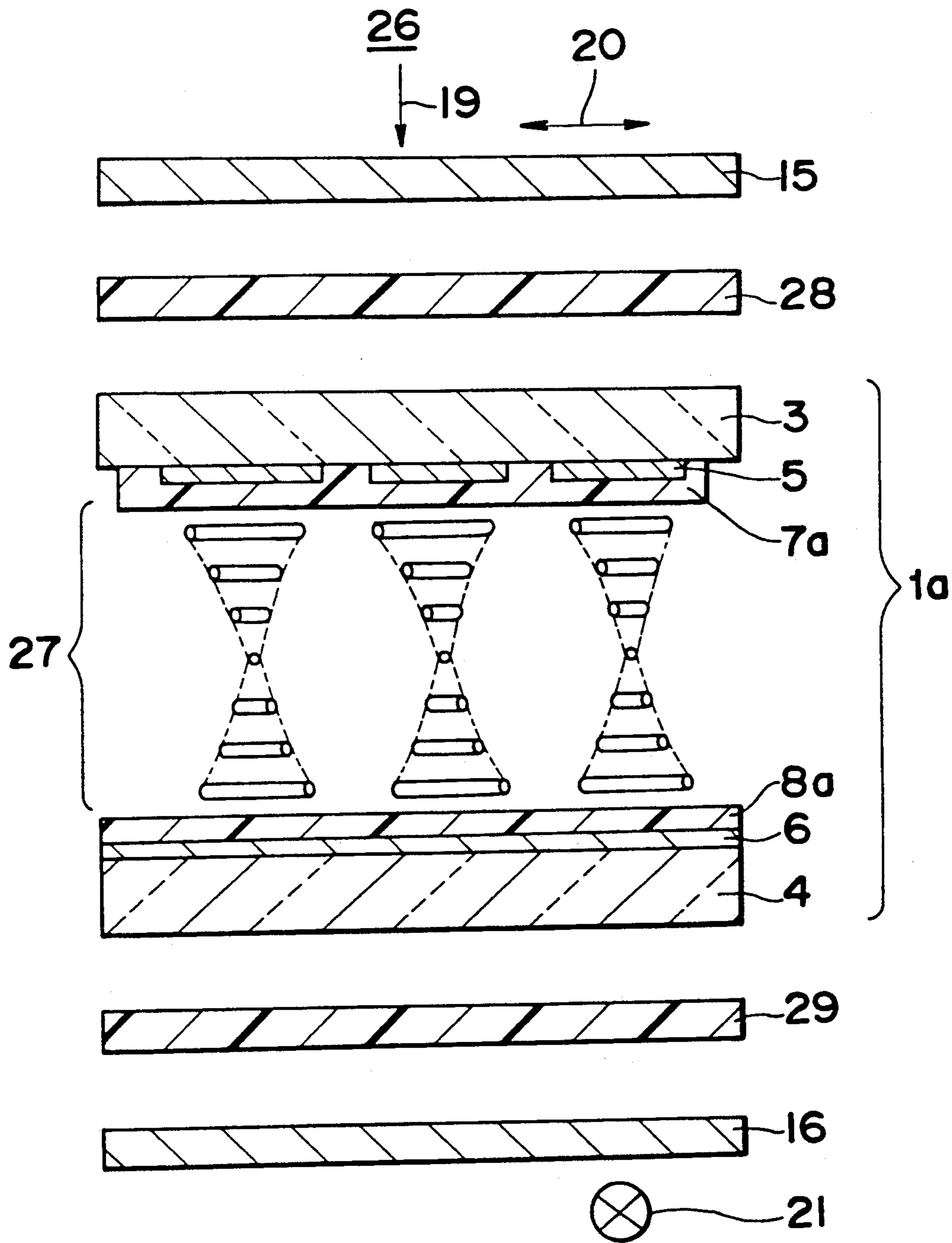
Fig. 6 PRIOR ART
