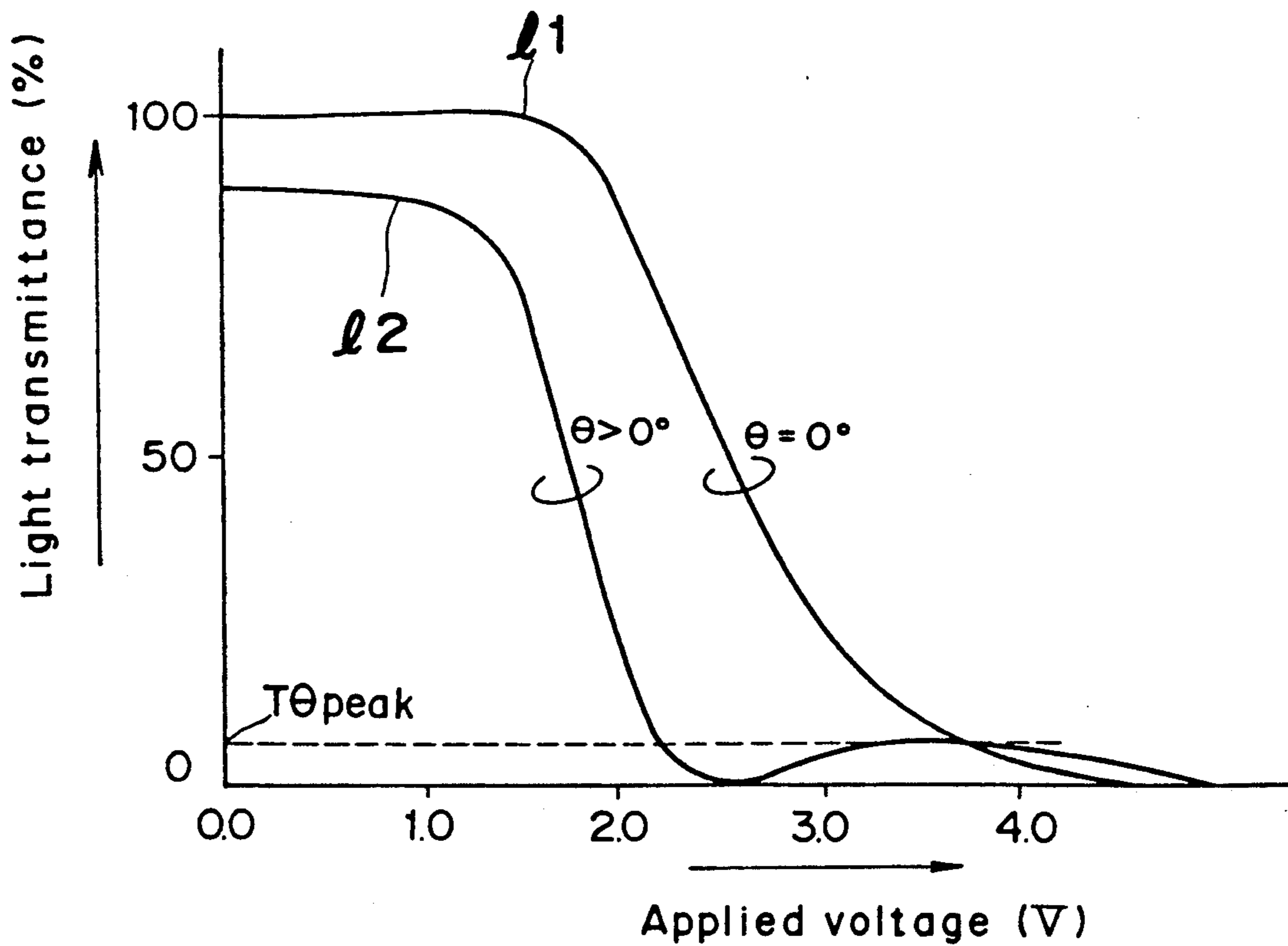
Fig. 3 PRIOR ART
