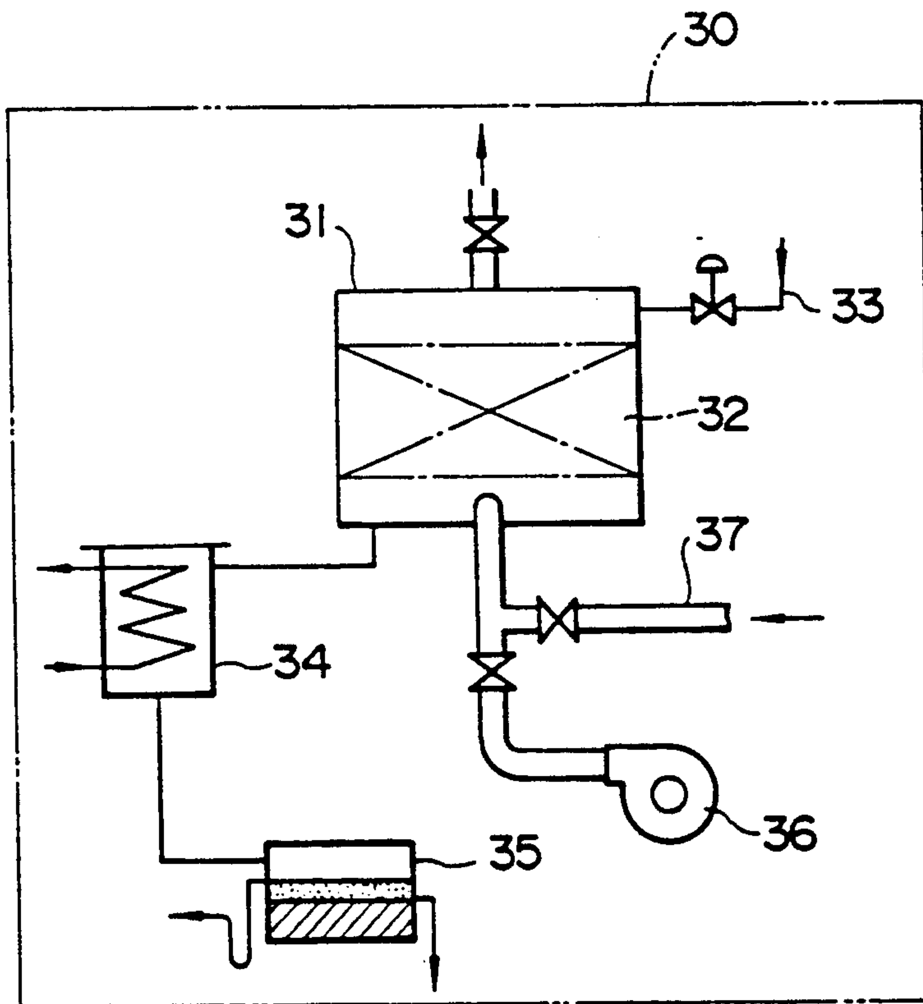
FIG. 10 (PRIOR ART)
