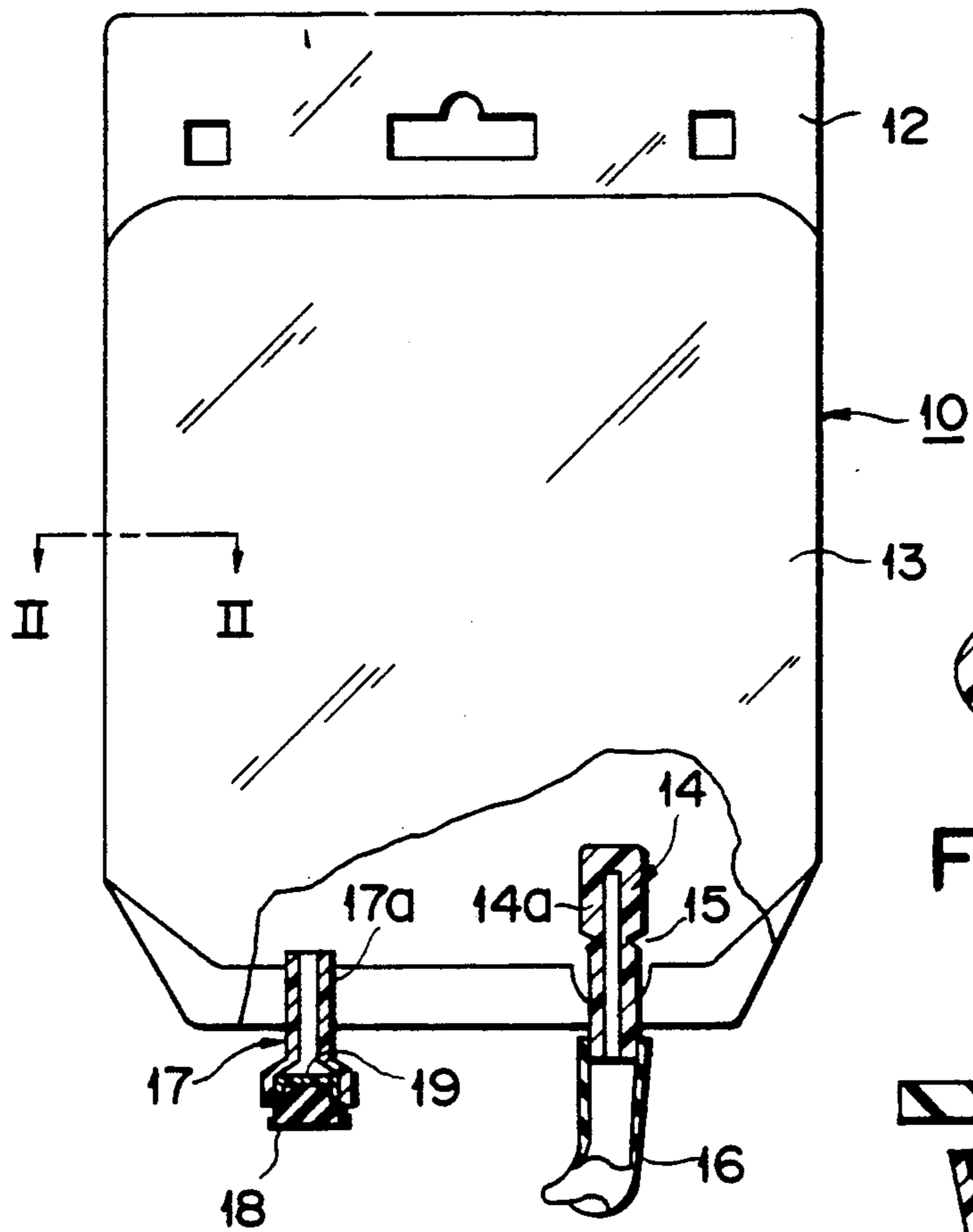
FIG. 1 (PRIOR ART)
