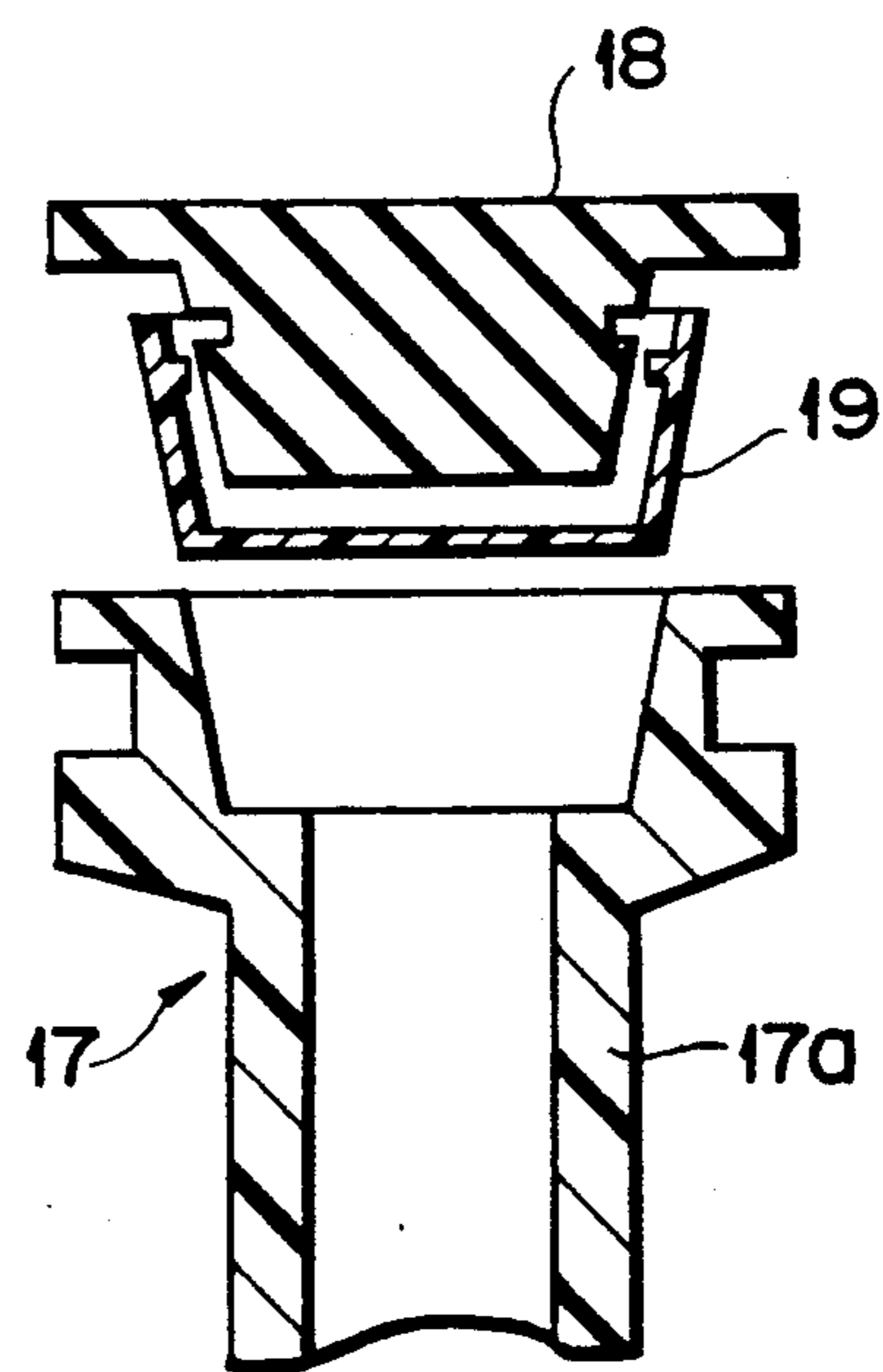
FIG. 2 (PRIOR ART)
