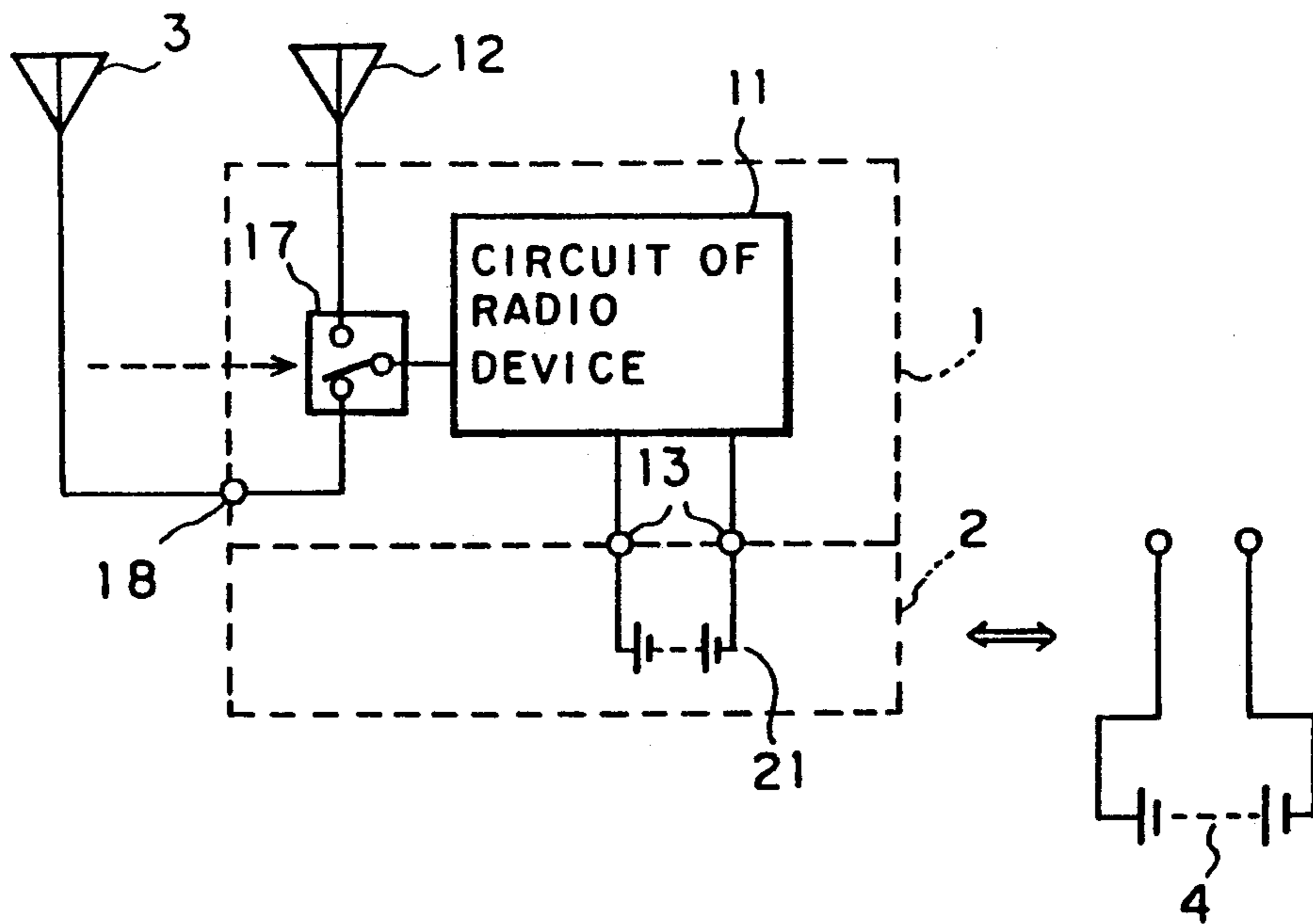
FIG. 2 (PRIOR ART)
