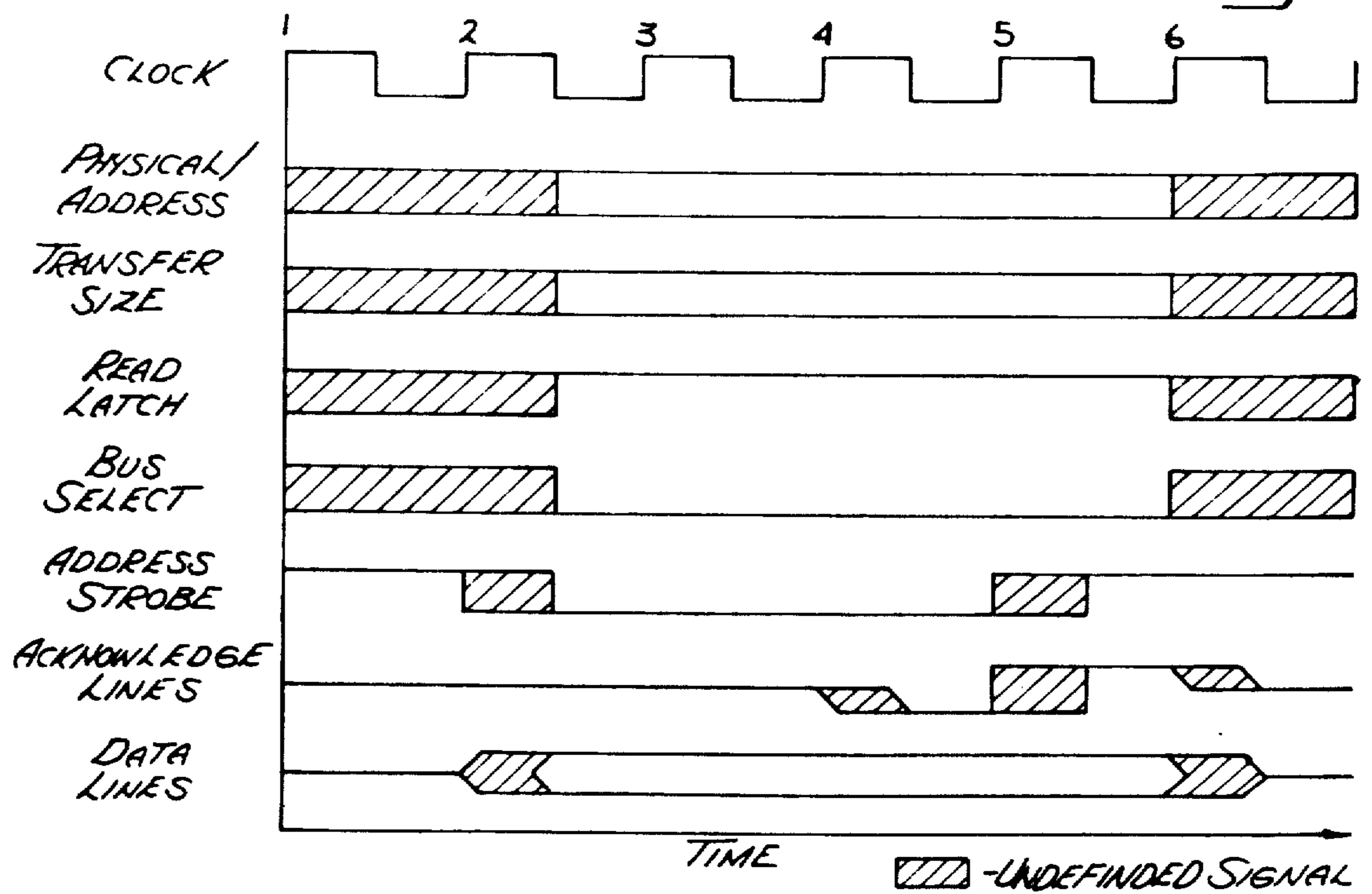
WRITE CYCLE
