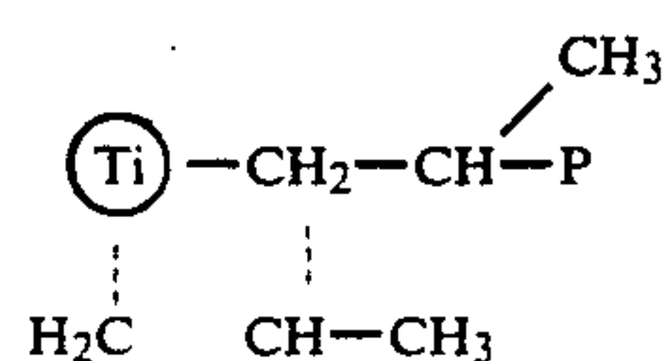
Primary Addition 1-2 Cis Insertion
