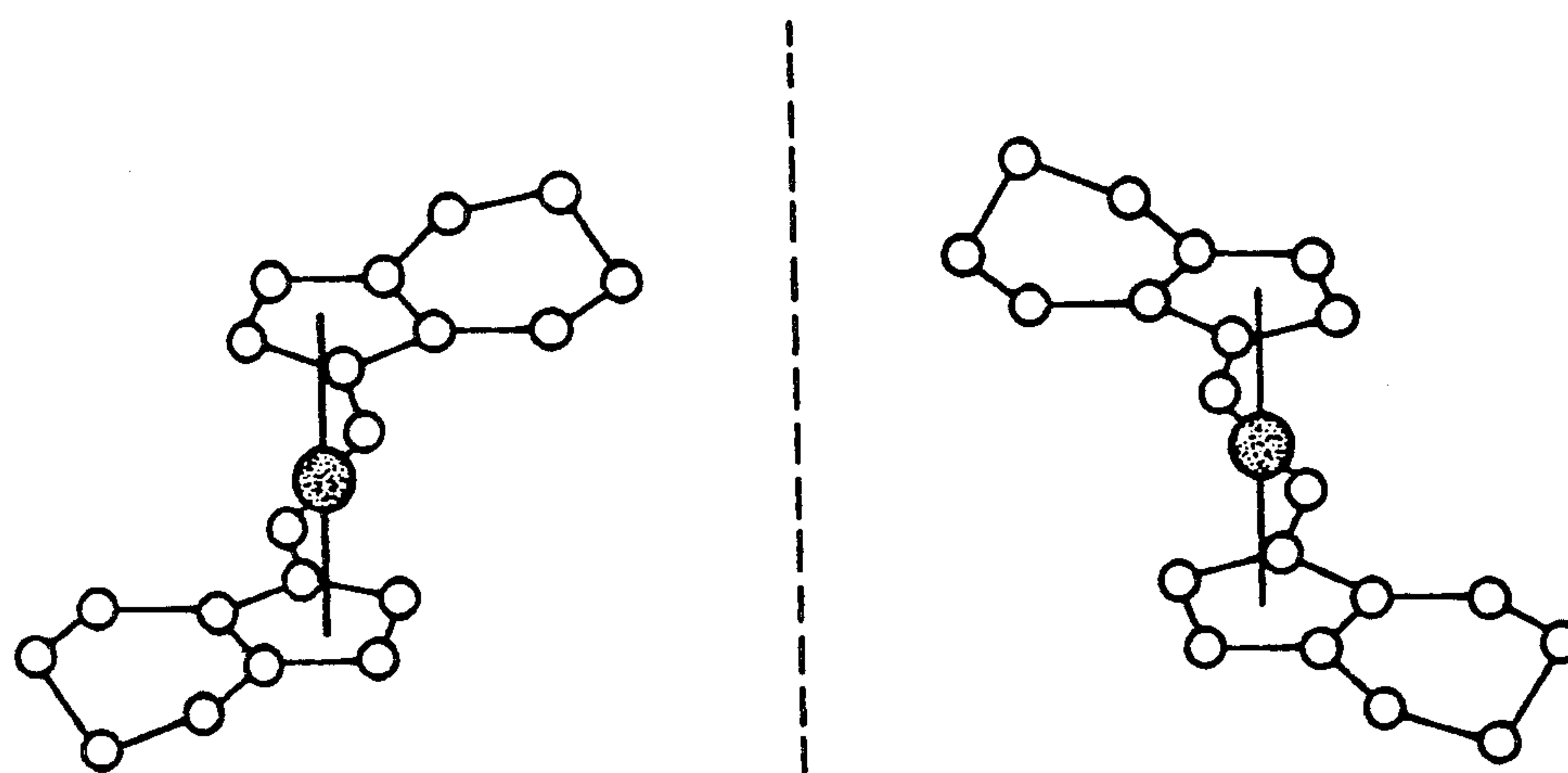
MIRROR IMAGE RACEMIC FORMS
