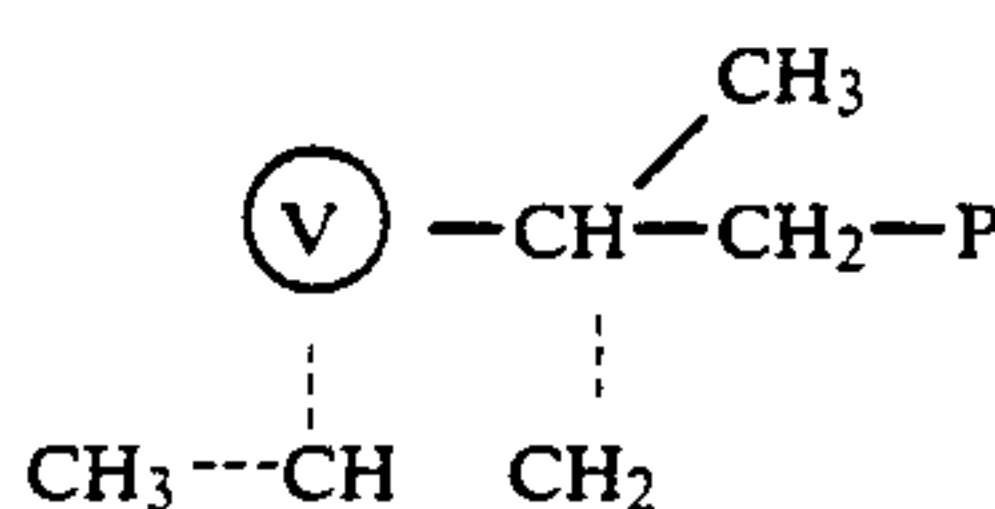
Secondary Addition 2-1 Cis Insertion
