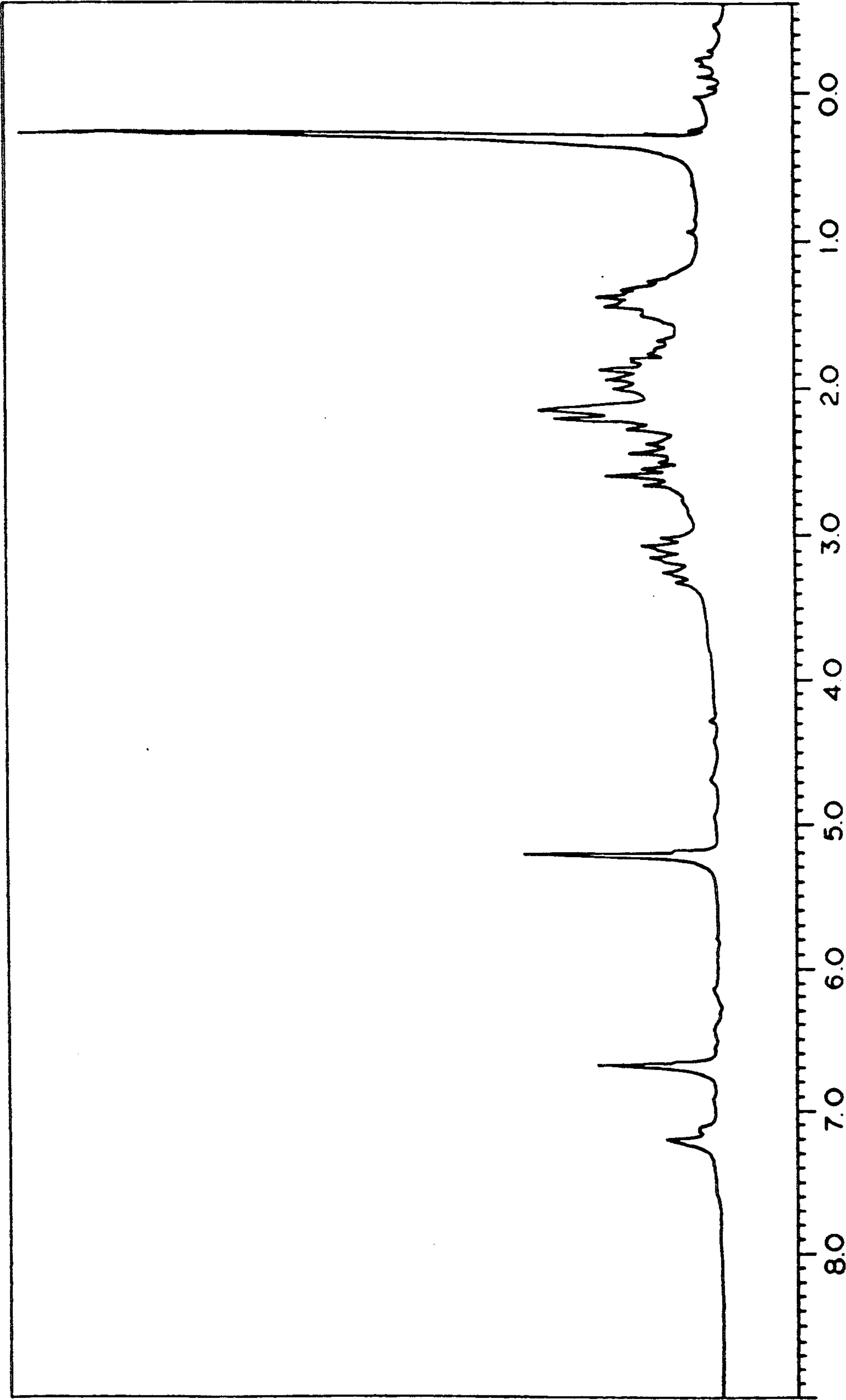
FIG. 9 \delta , ppm (REFERENCE TOLUENE, 7.2 ppm)
