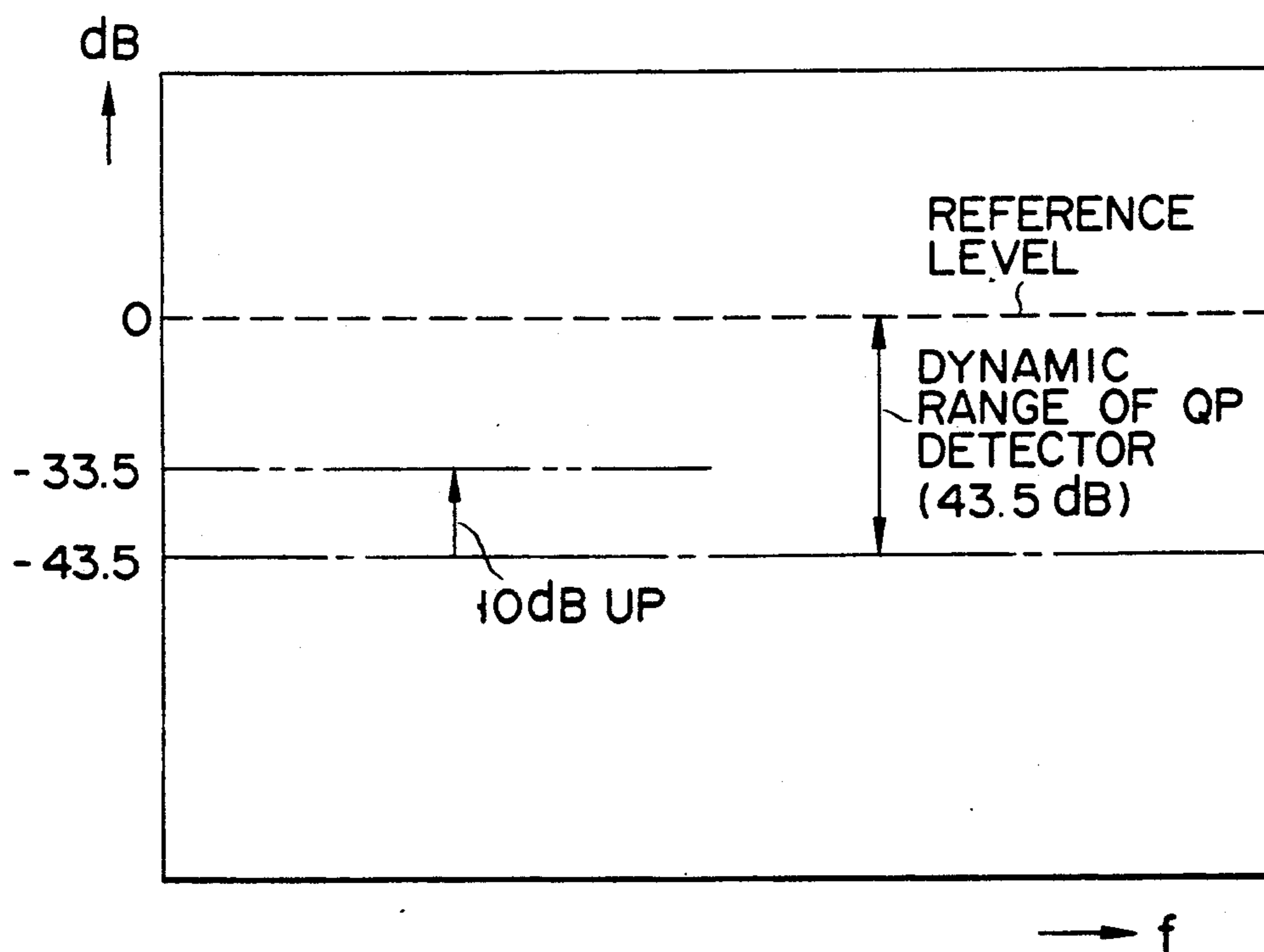
FIG. 9 PRIOR ART
