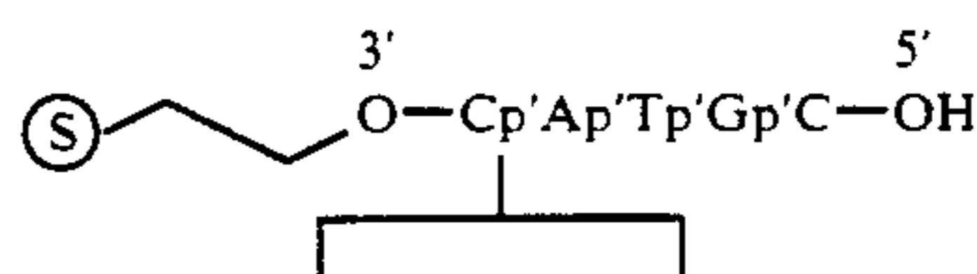
Reaction Scheme for Example 14
