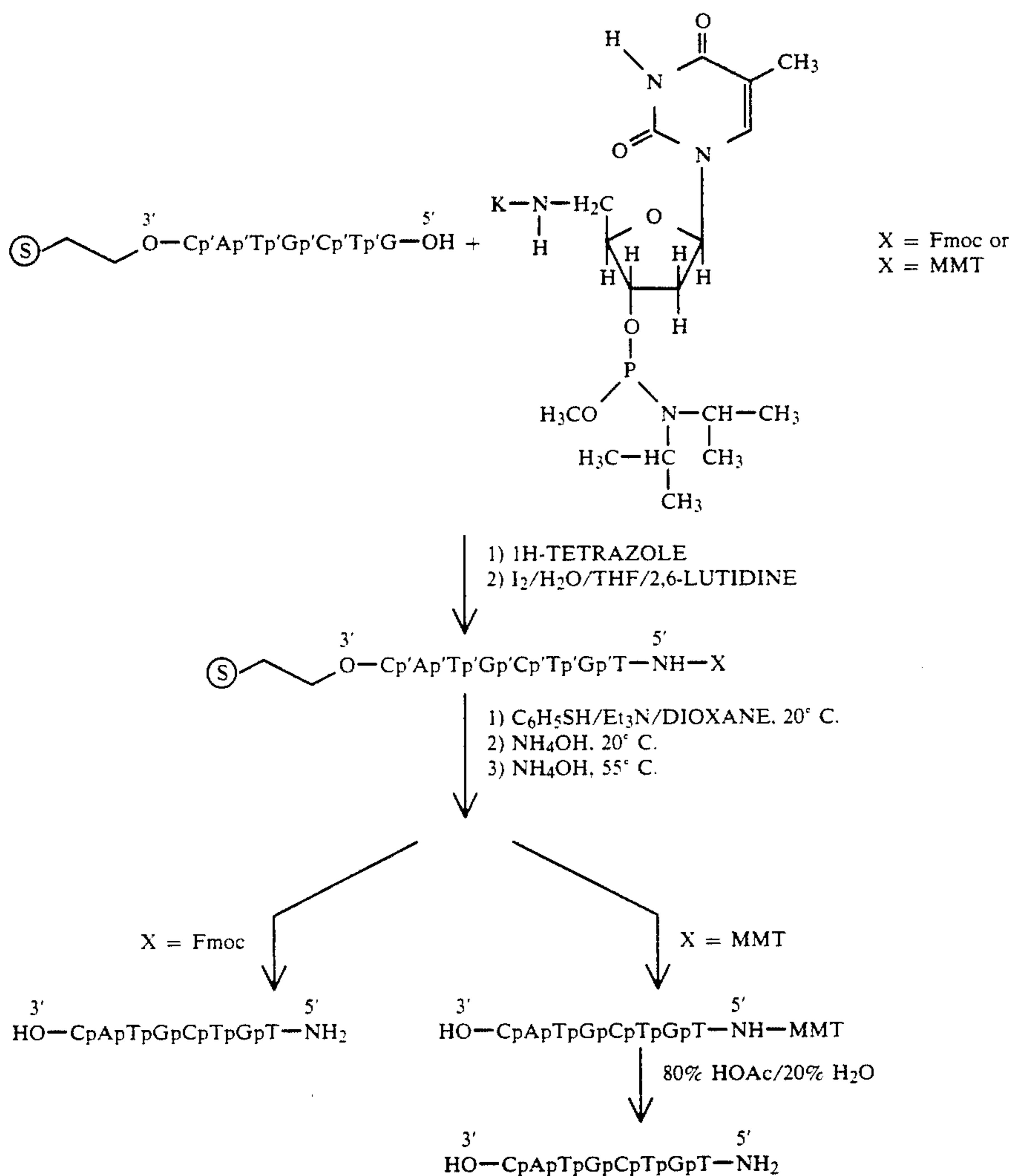
Reaction Scheme for Example 11
