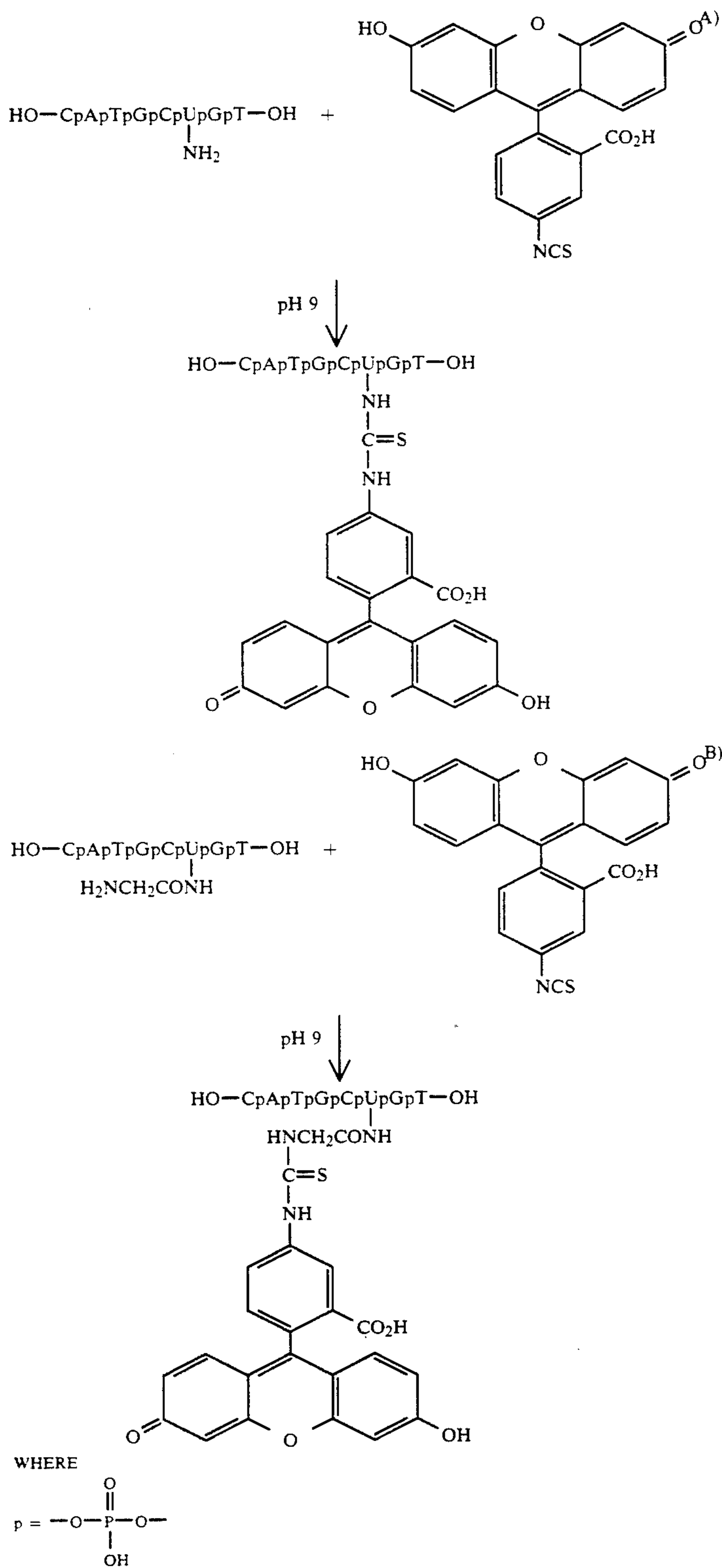
Reaction Scheme for Example 15
