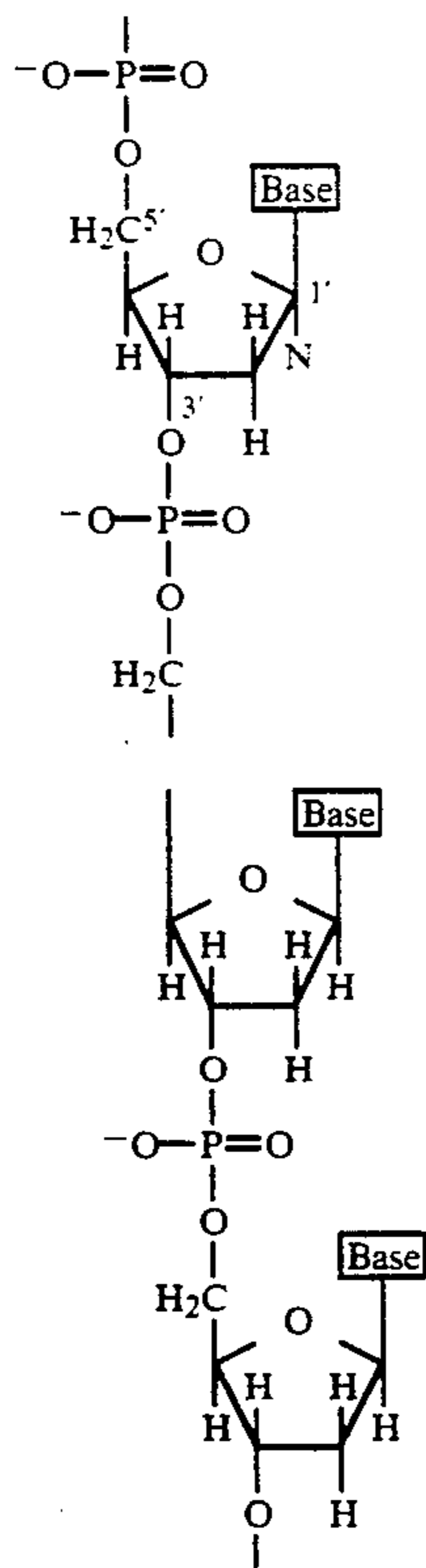
Structure of part of a DNA chain.
