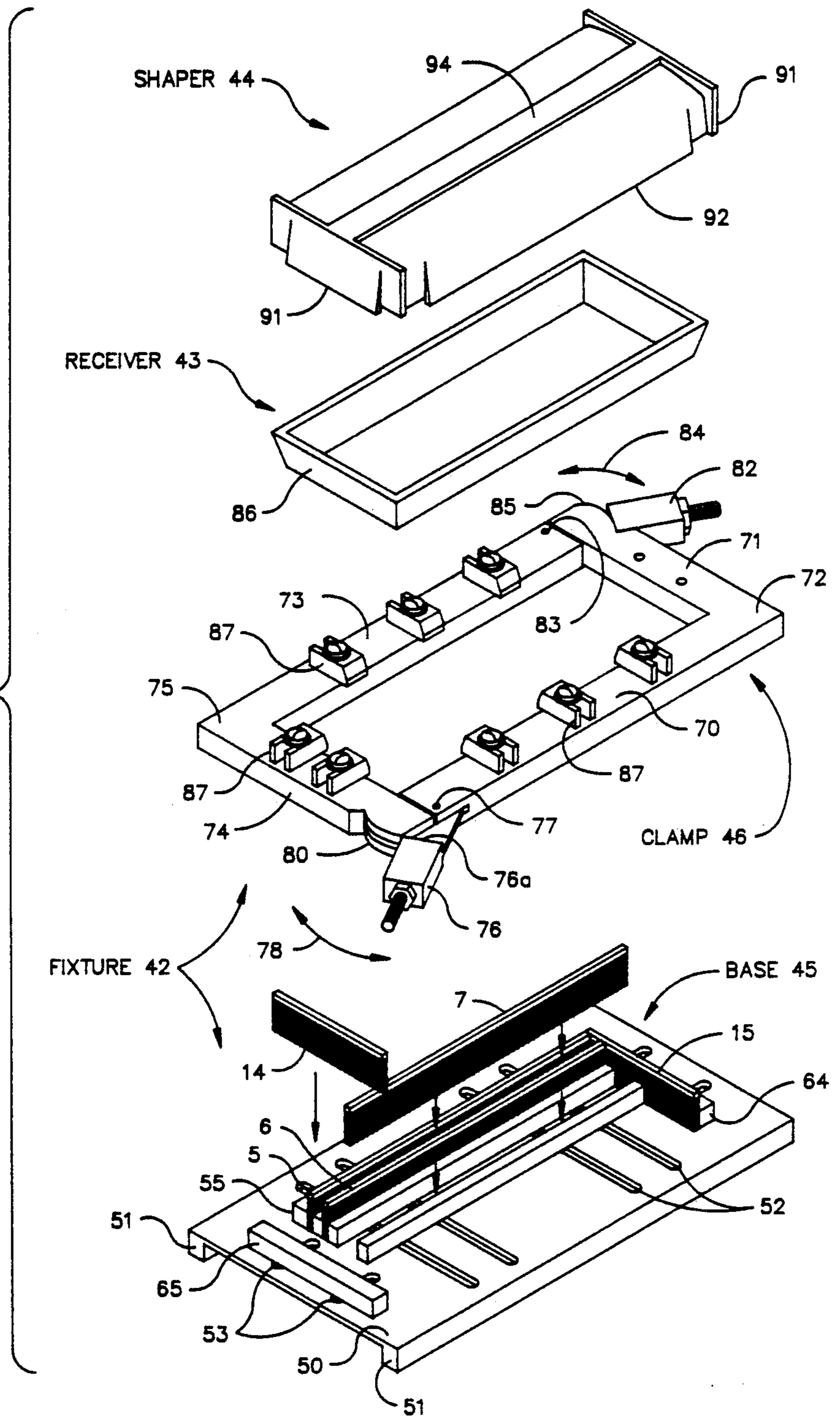
FIG 8 CAVITY FORMER 40
