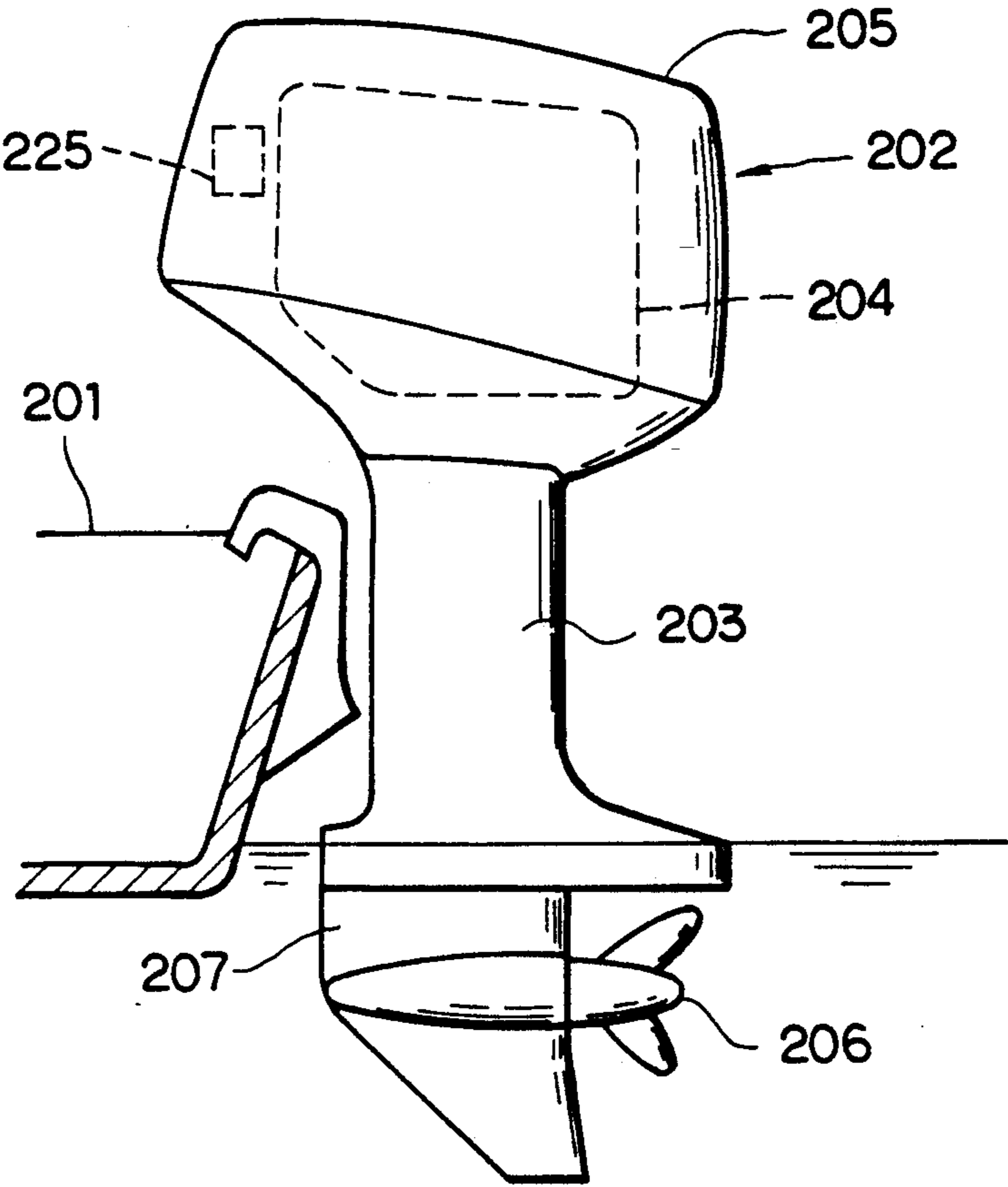
FIG. 8 PRIOR ART
