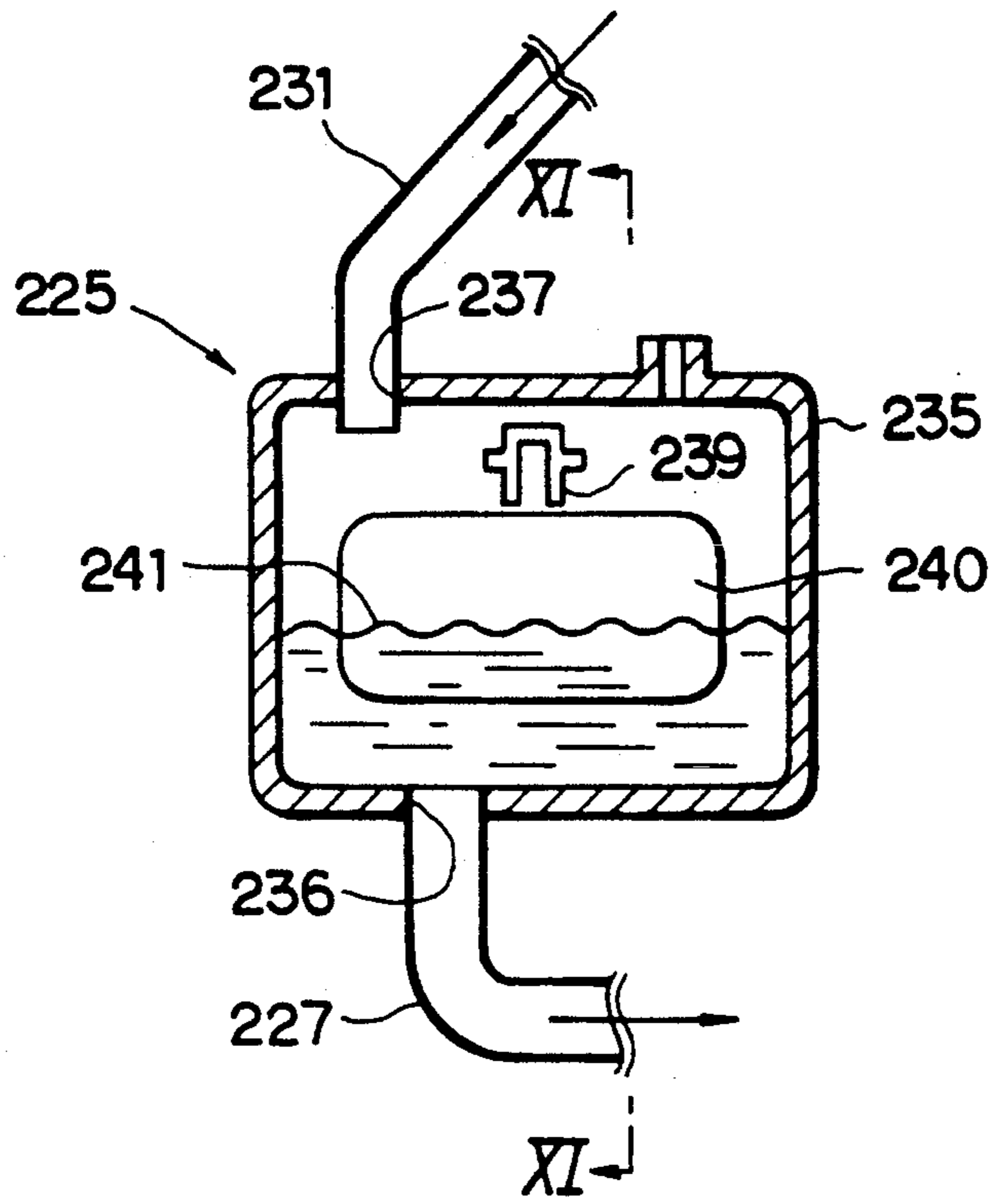
FIG. 10 PRIOR ART
