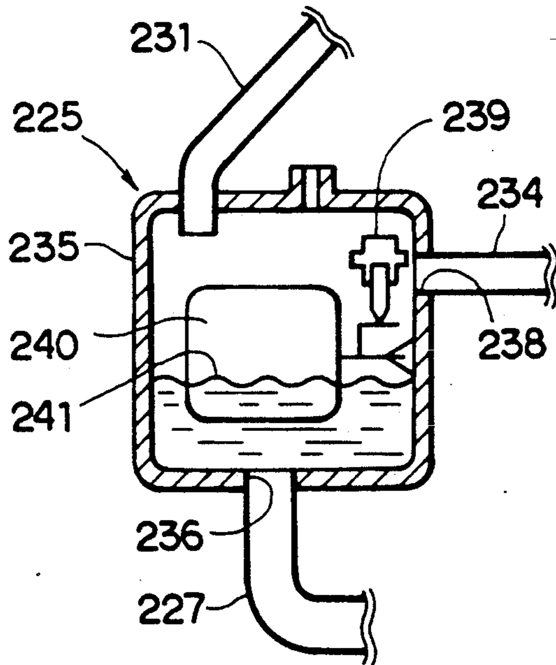
FIG. 11 PRIOR ART
