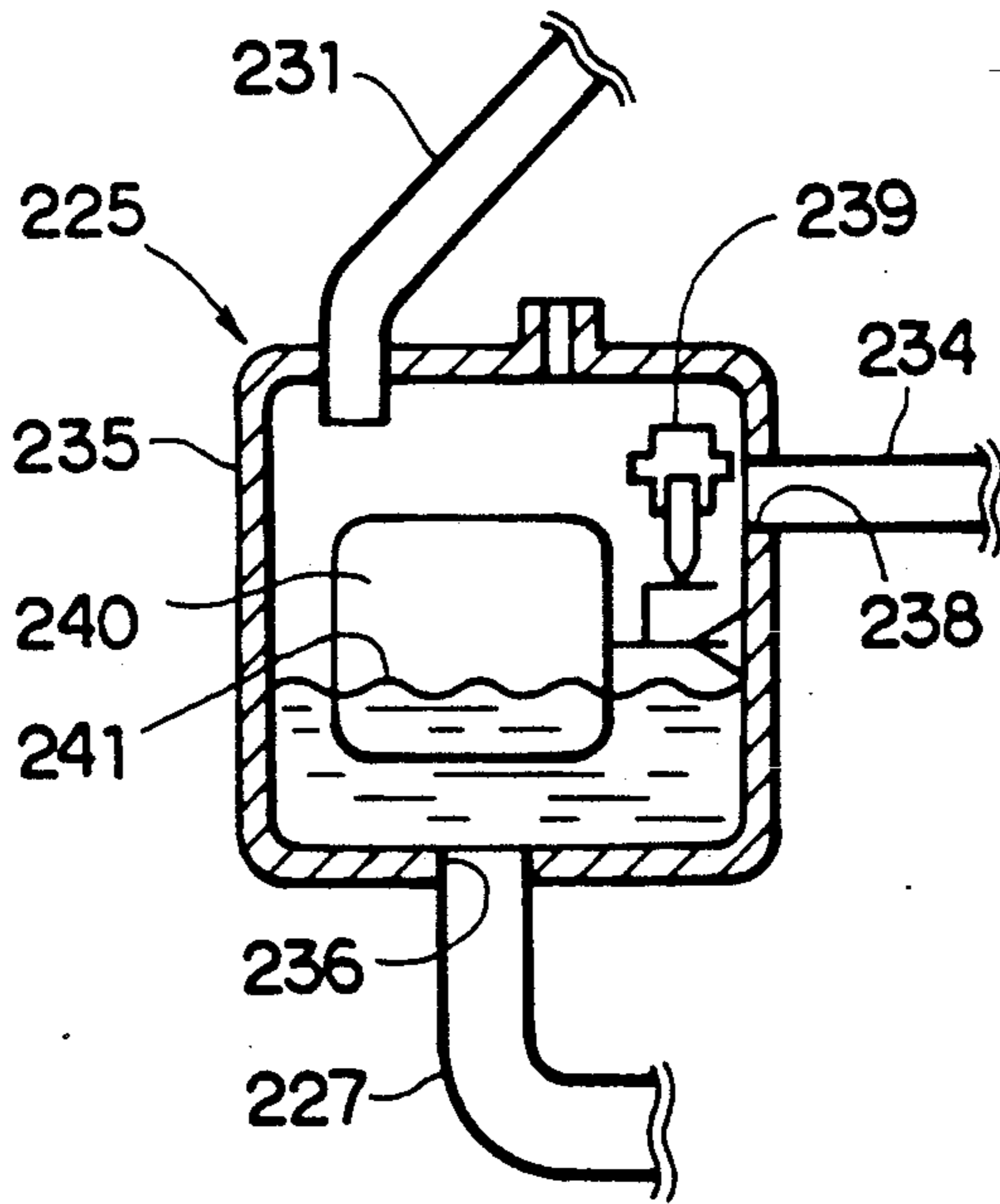
FIG. 11 PRIOR ART
