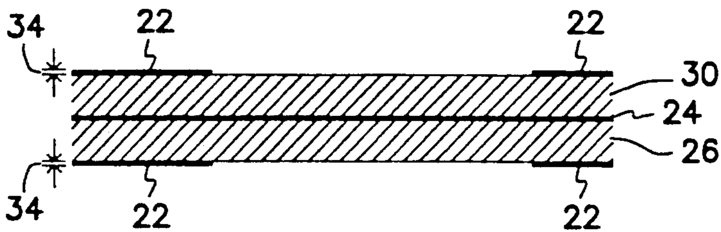
GROW SiO 2 & SiN 3 PATTERN DIELECTRIC FIG. 3C
