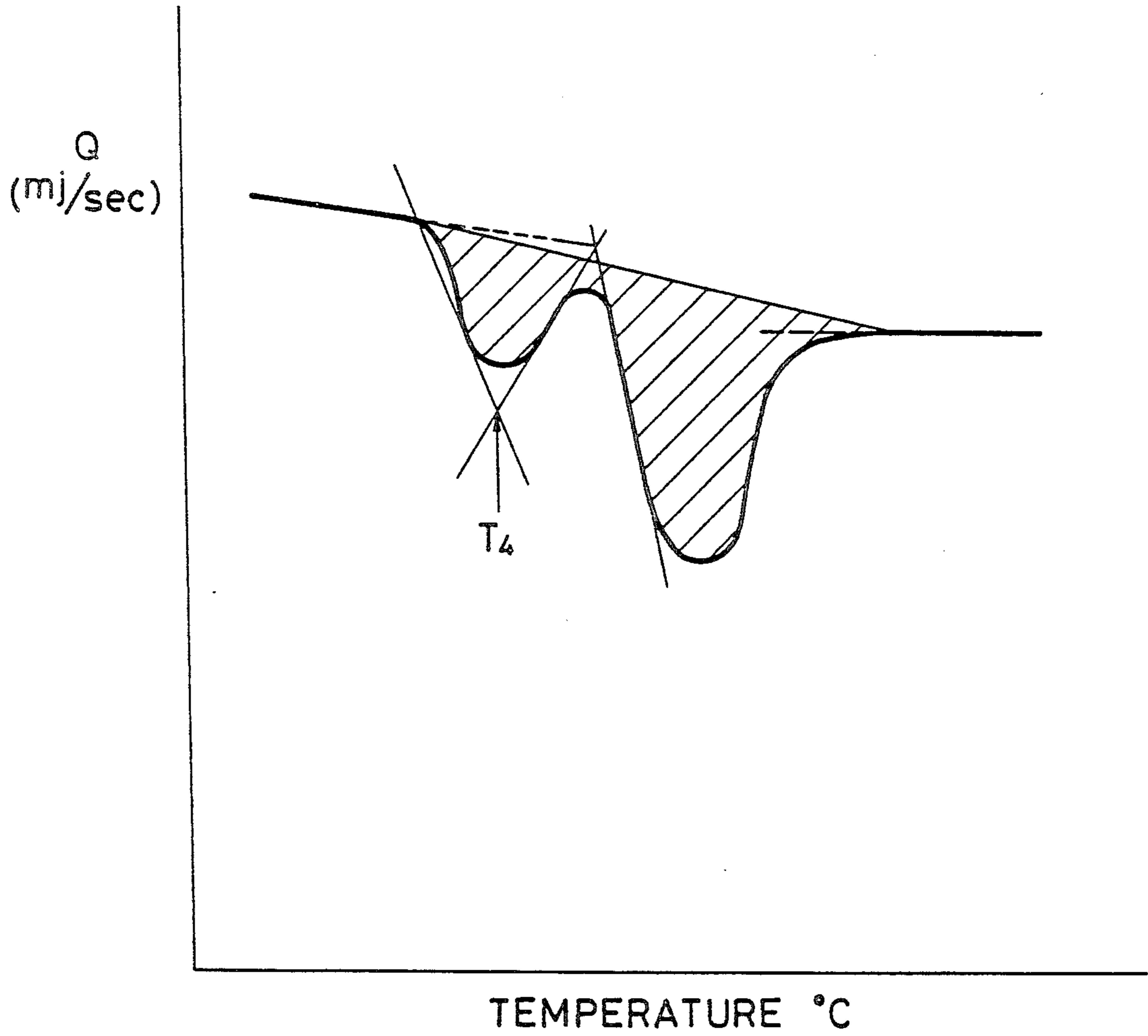
MAXIMUM VALUE ( T_4 ) OF HEAT ABSORPTION PEAK OF TONER BY DSC
