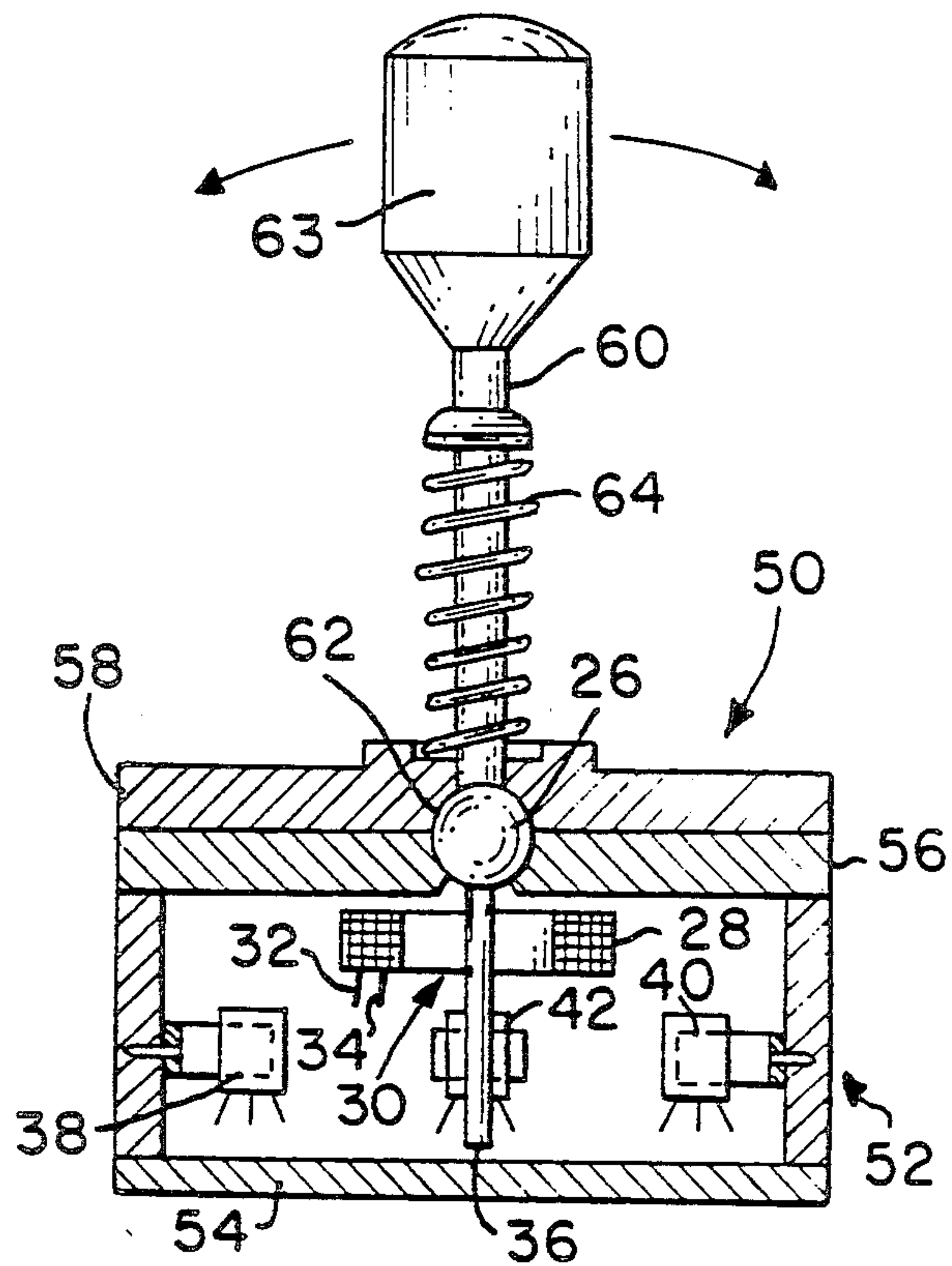
PRIOR ART
