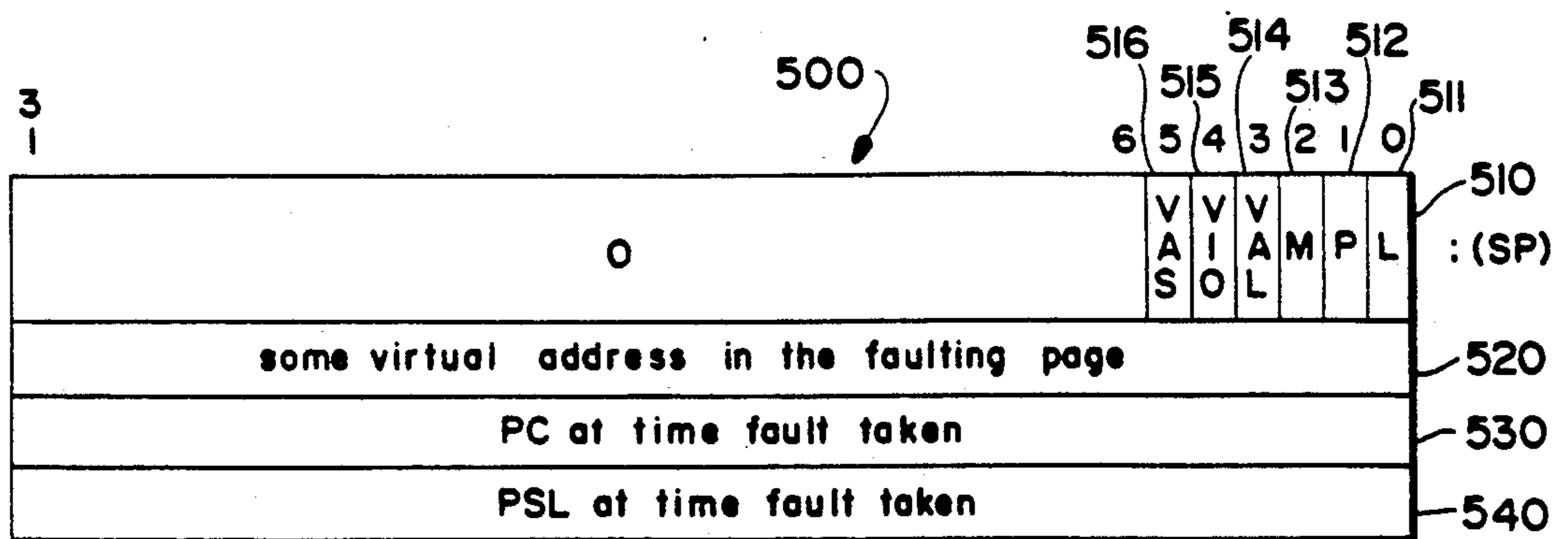
Memory Management Fault Stack Frame
