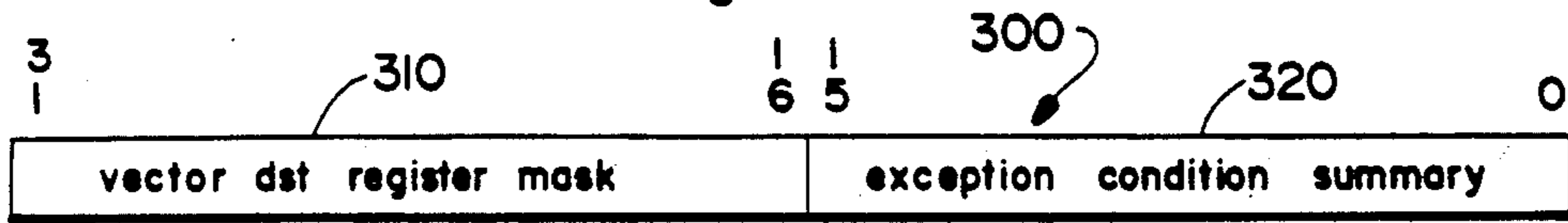
Vector Arithmetic Exception Register (VAER)
