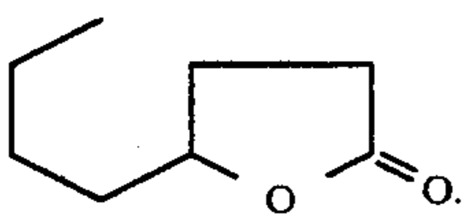
FIG. 26 is the GLC profile for the reaction product of Example VII(c). The peak indicated by reference numeral 292 is the peak for gamma octalactone having the structure:
