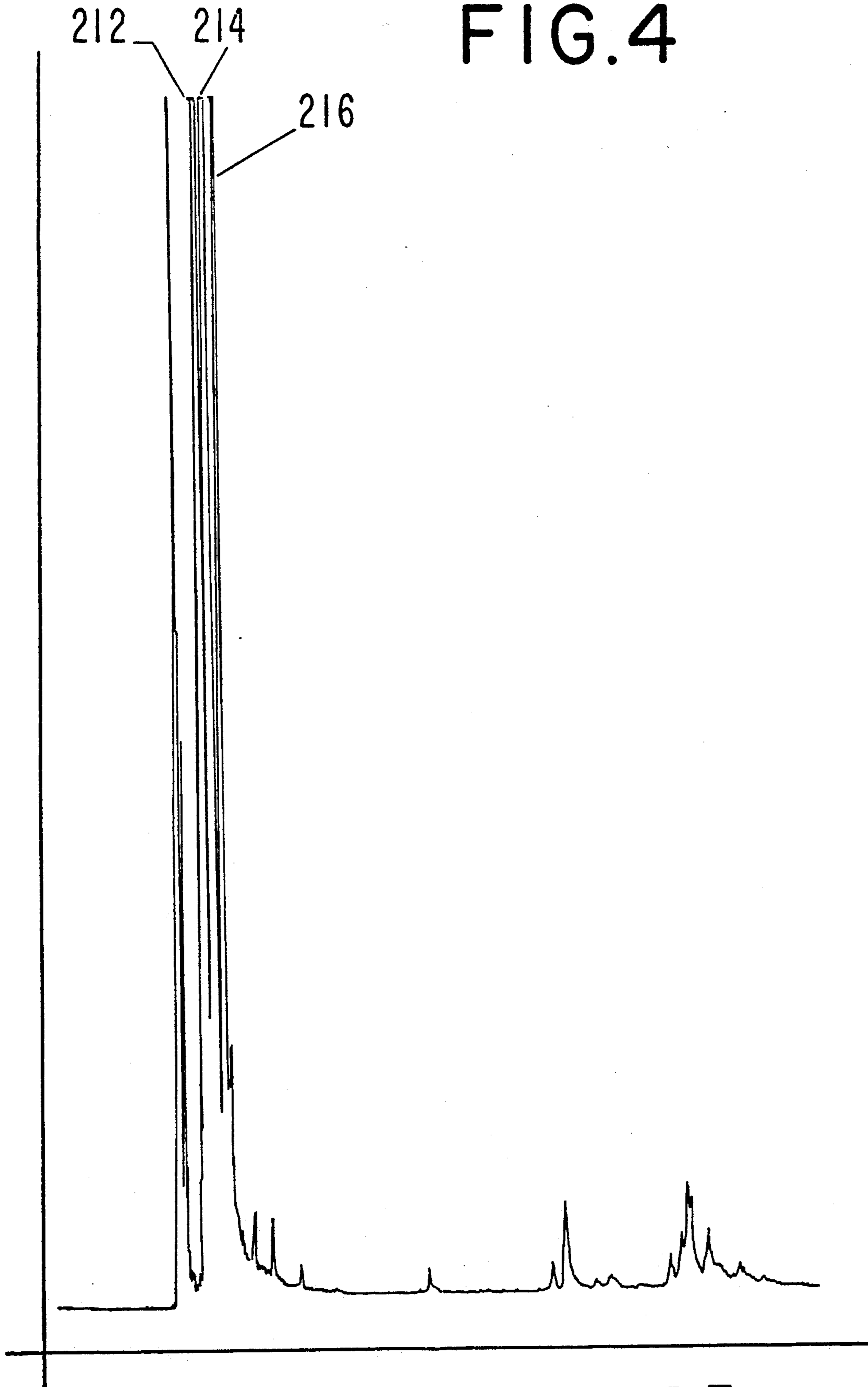
GLC PROFILE FOR EXAMPLE I(c).
