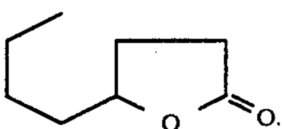
FIG. 26 is the GLC profile for the reaction product of Example VII(c). The peak indicated by reference numeral 292 is the peak for gamma octalactone having the structure:
