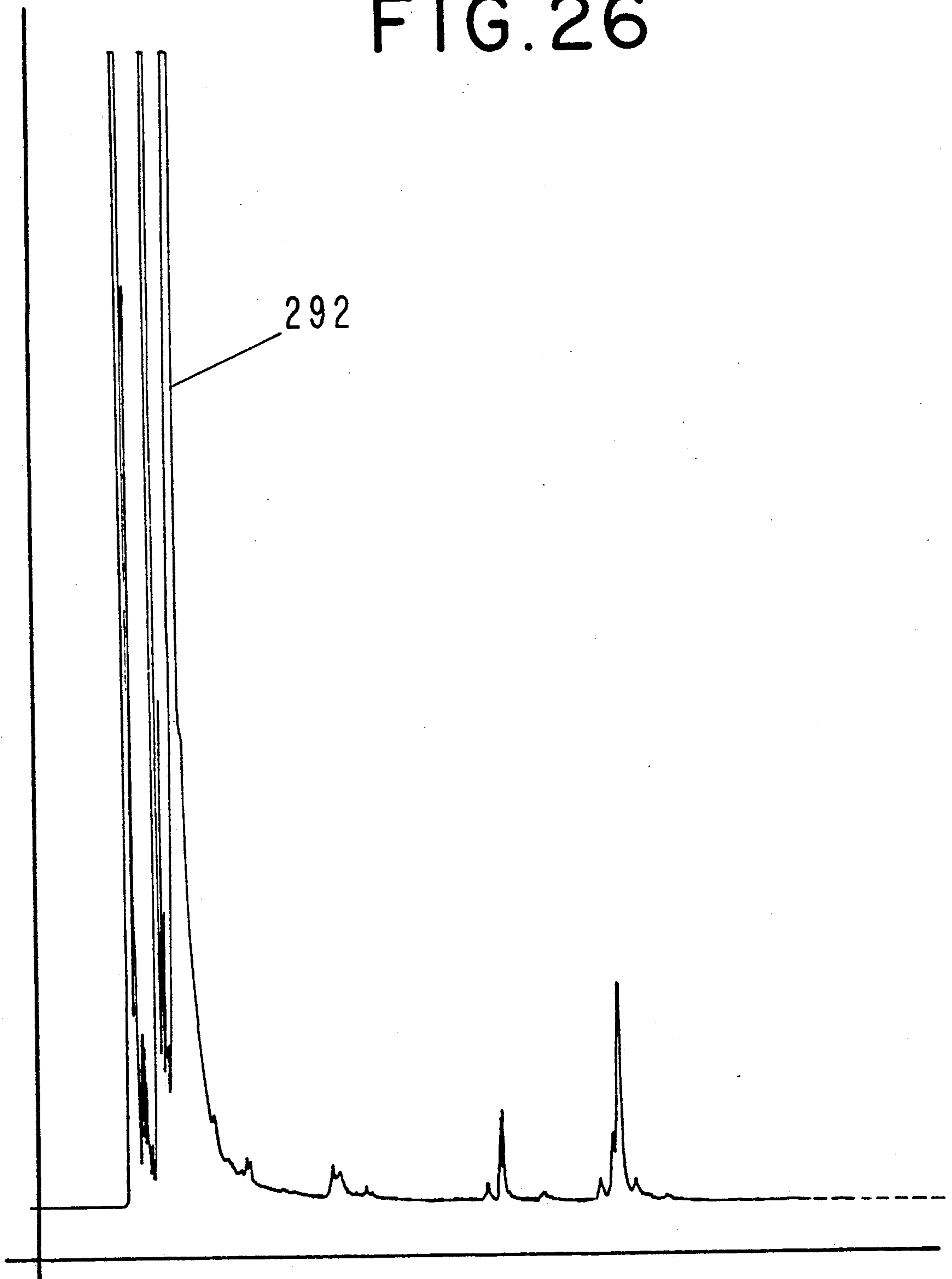
GLC PROFILE FOR EXAMPLE VII (c) .
