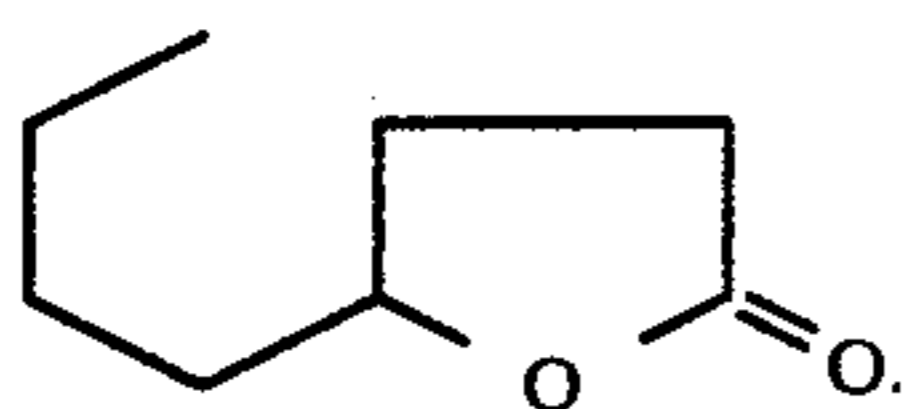
FIG. 24 is the GLC profile for the reaction product of Example VII(a). The peak indicated by reference numeral 288 is the peak for gamma octalactone having the structure:
