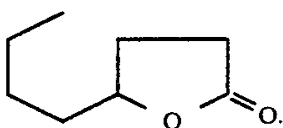
FIG. 25 is the GLC profile for the reaction product of Example VII(b). The peak indicated by reference numeral 290 is the peak for gamma octalactone having the structure:
