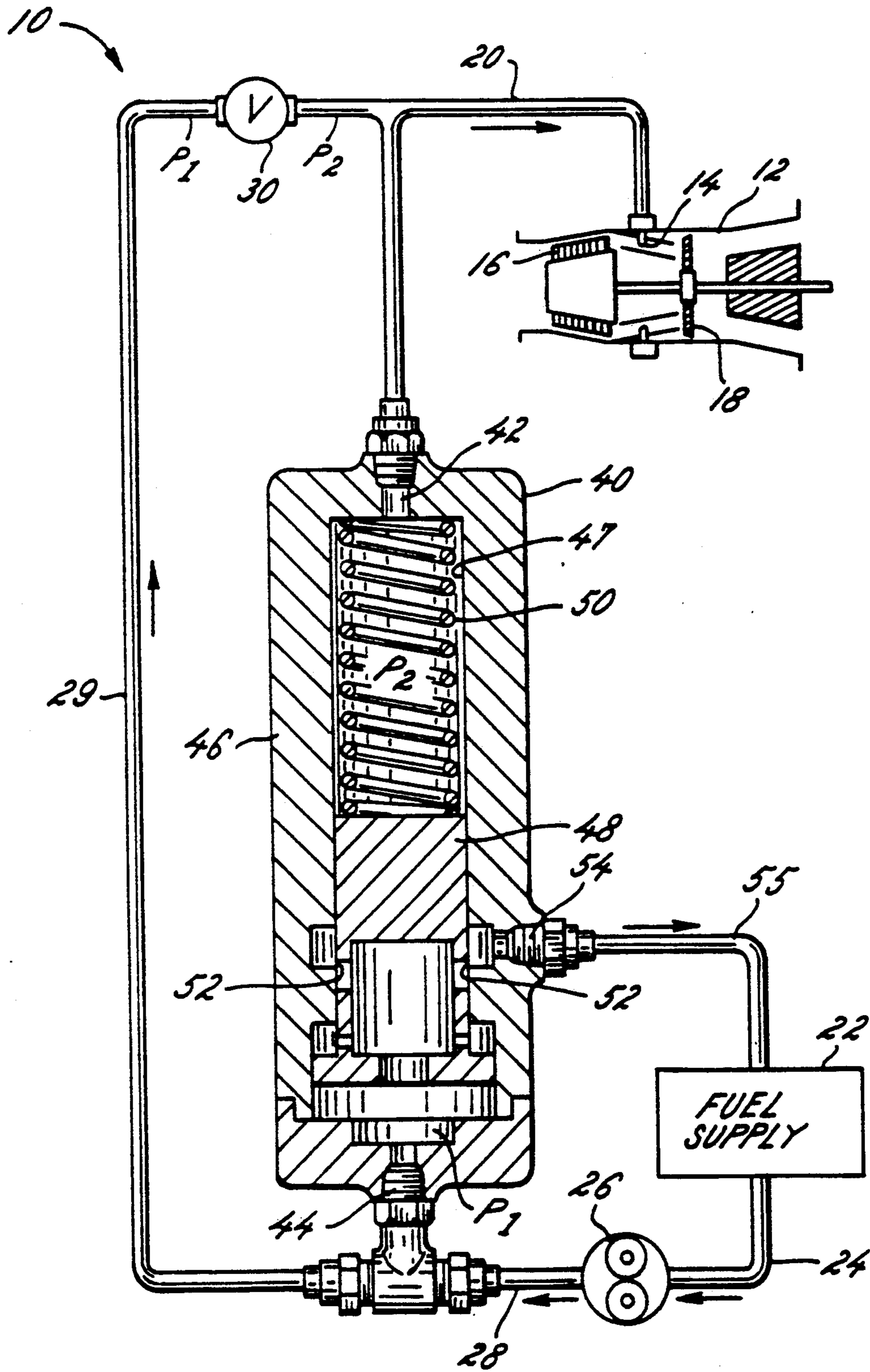
FIG. 1 (PRIOR ART)
