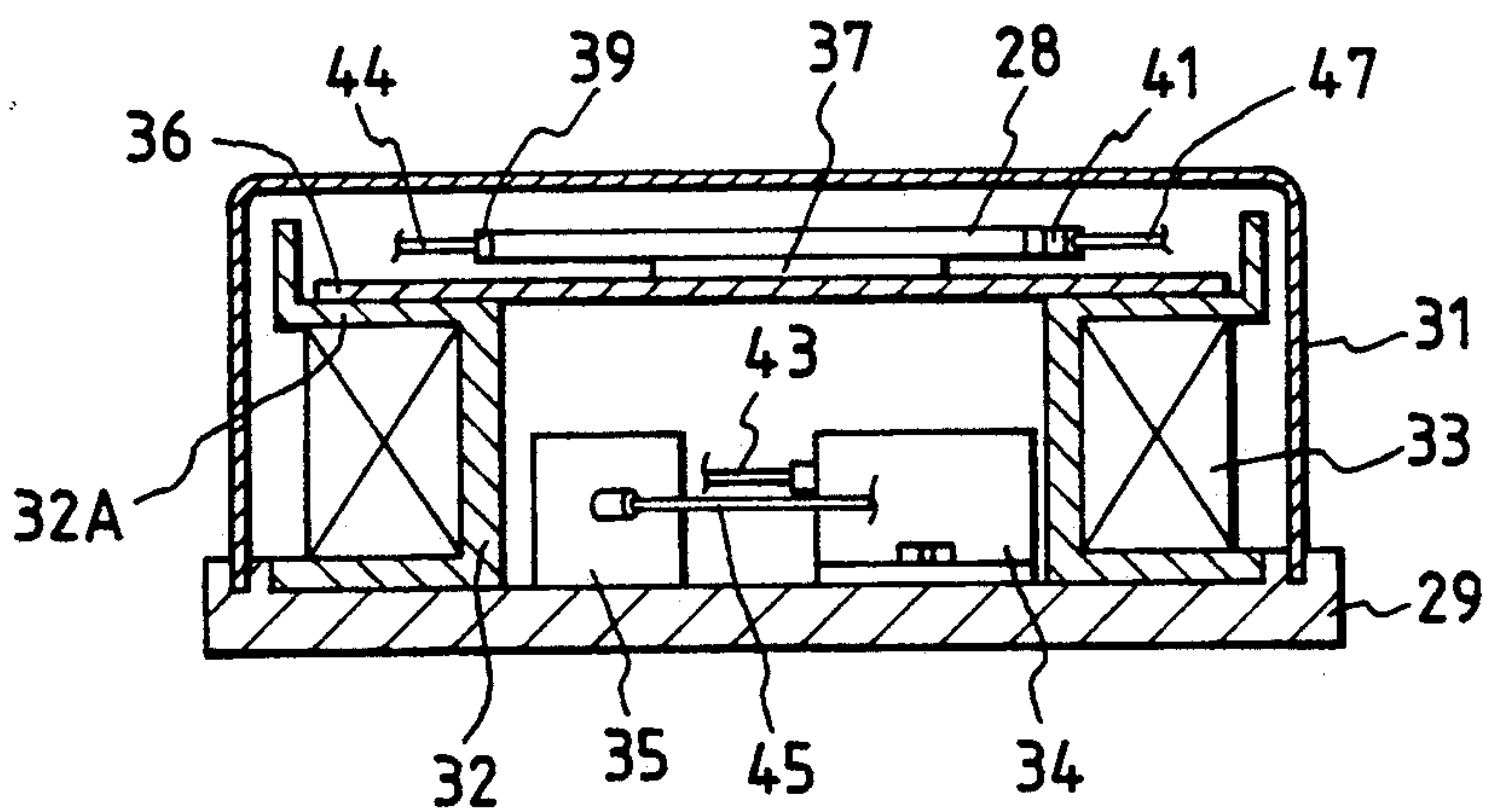
FIG. 4 PRIOR ART
