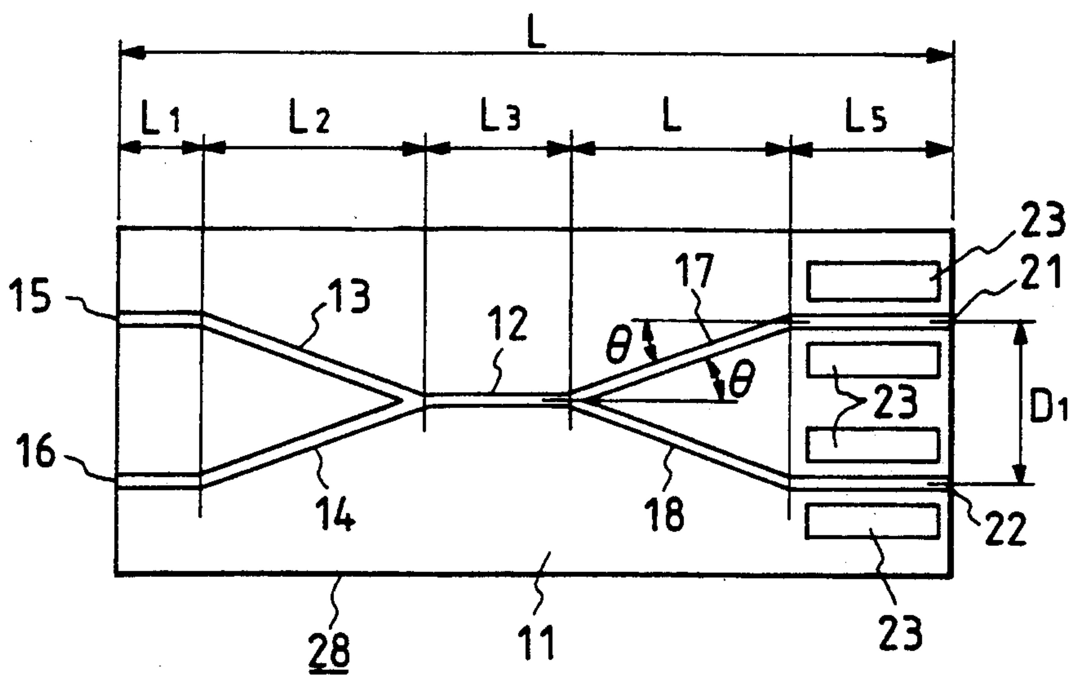
FIG. 1 PRIOR ART
