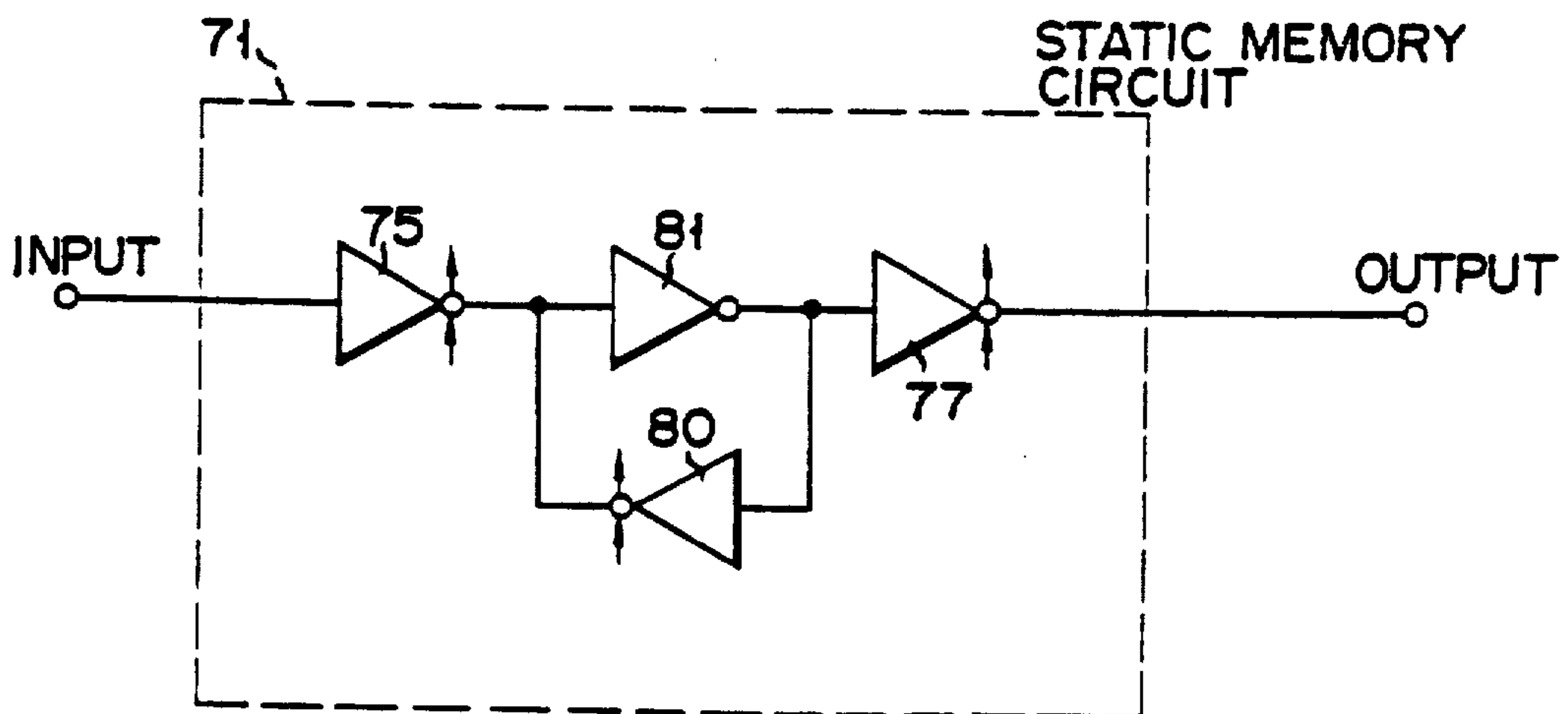
FIG. 9 (PRIOR ART)
