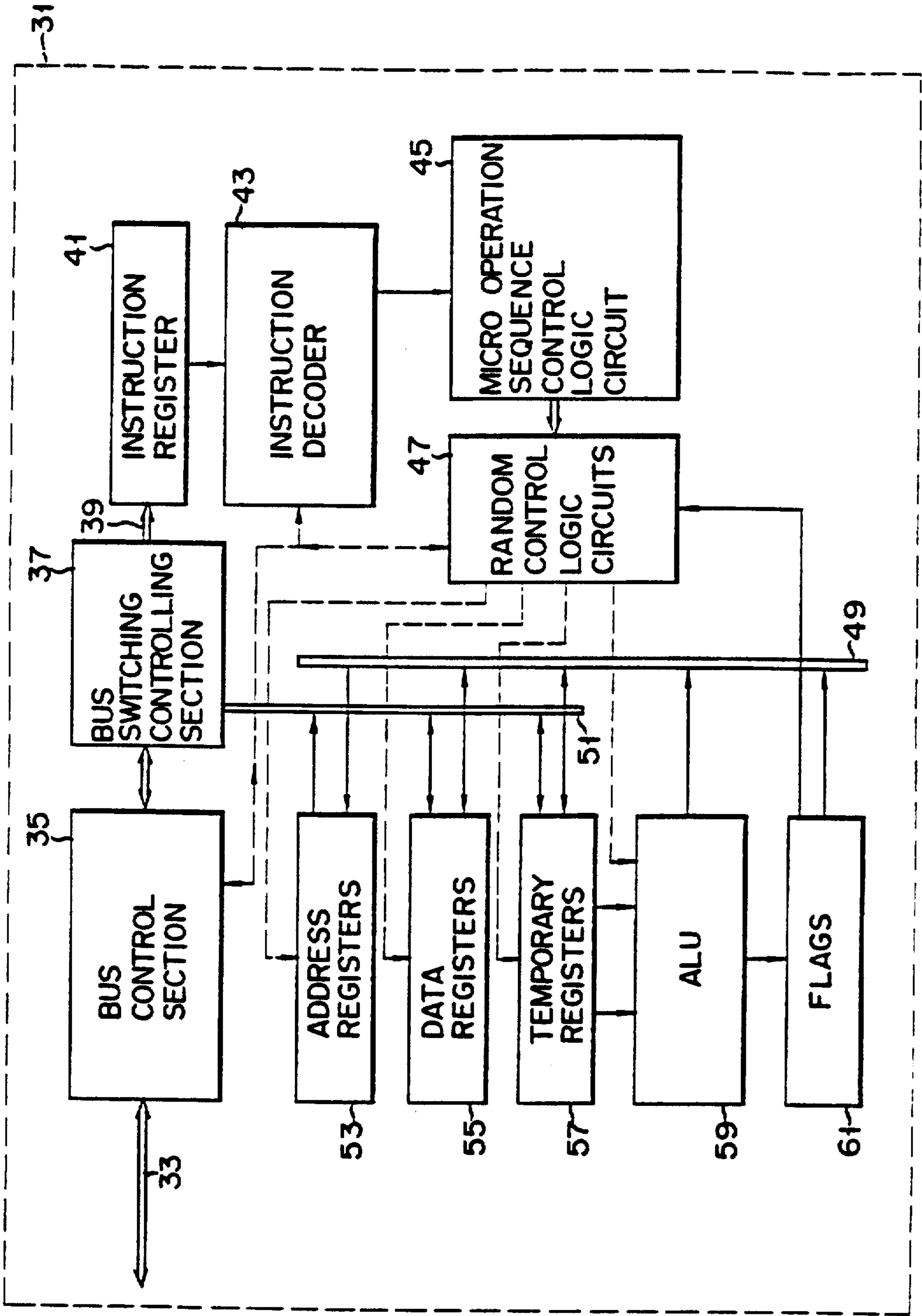
FIG. 3 (PRIOR ART)
