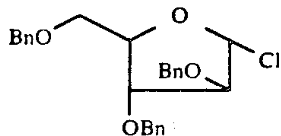
Alpha-chlorosugar III (~100%)
