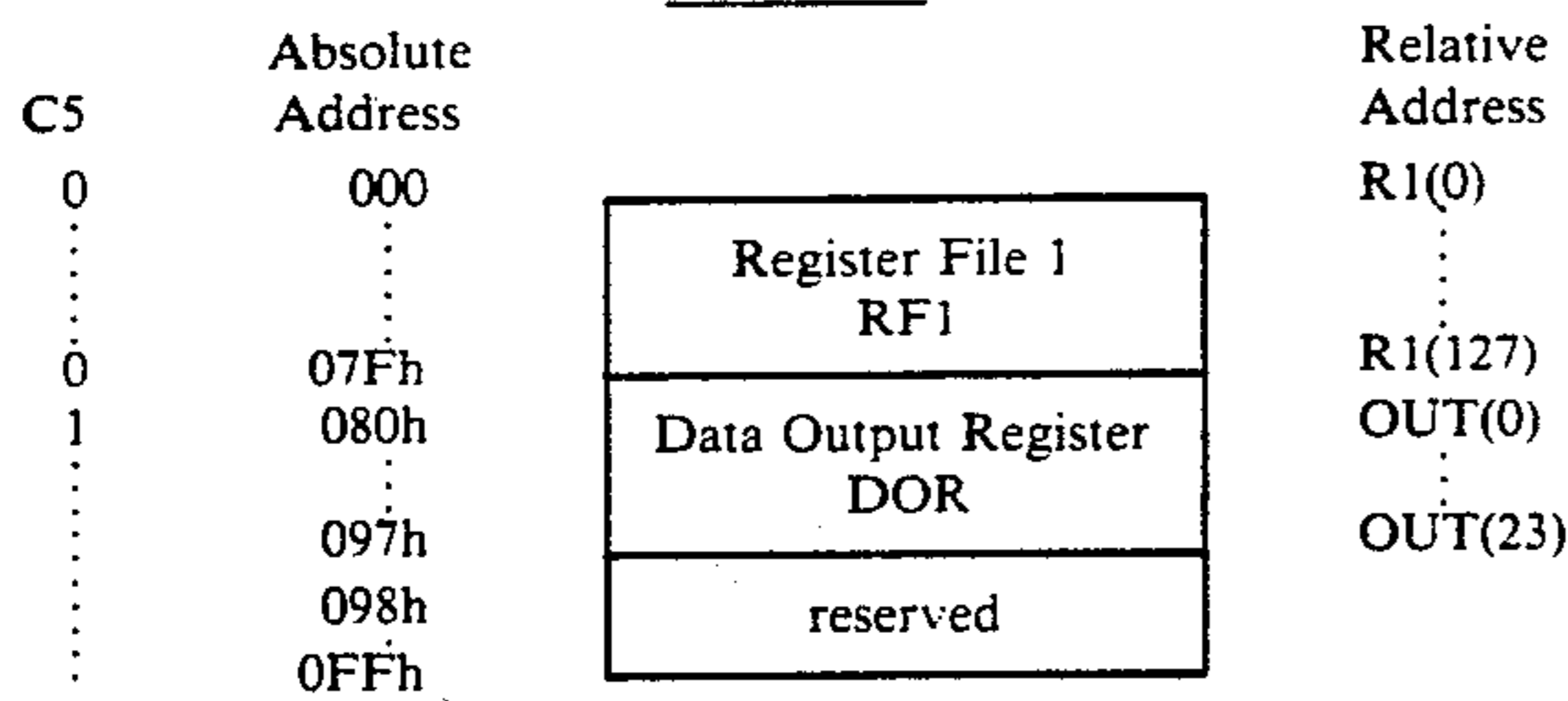
DOR/RF1 Memory Map: h indicates hexadecimal
