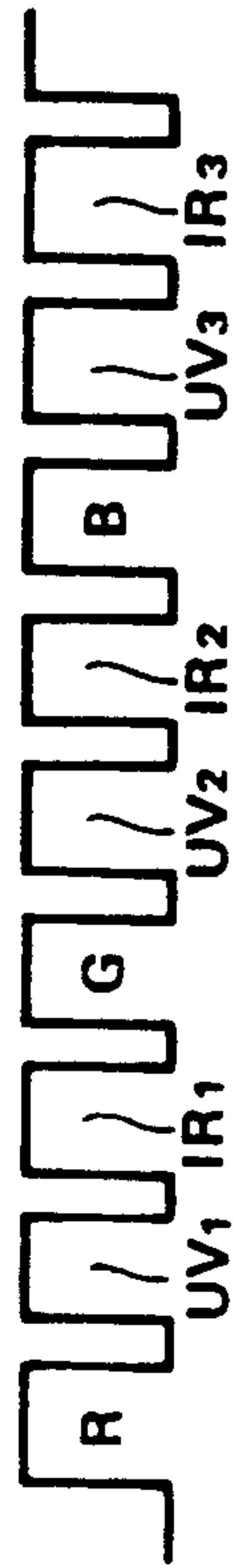
FIG.11(A) ILLUMINATING LIGHT
