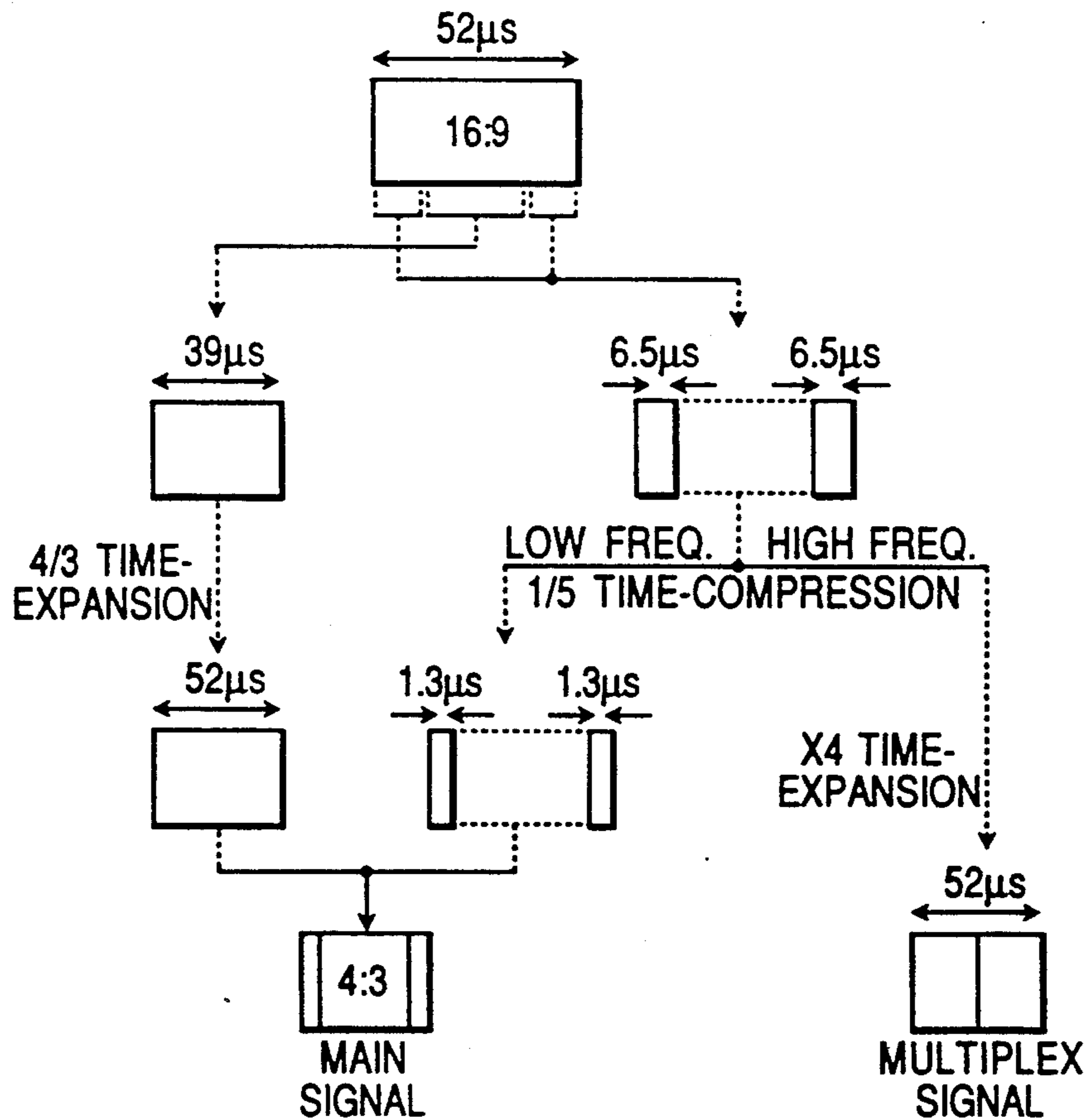
FIG. 10 PRIOR ART
