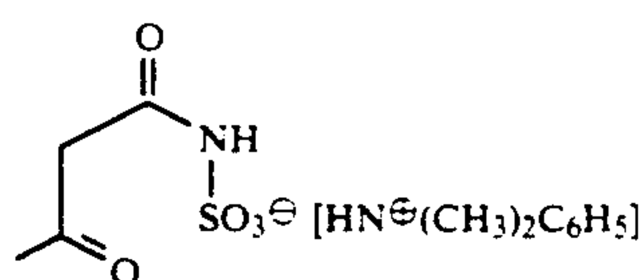
dimethylphenylammonium acetoacetamide-N-sulfonate
