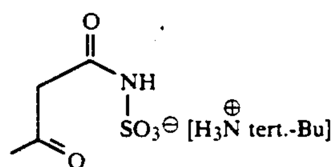
tert.-butylammonium acetoacetamide-N-sulfonate
