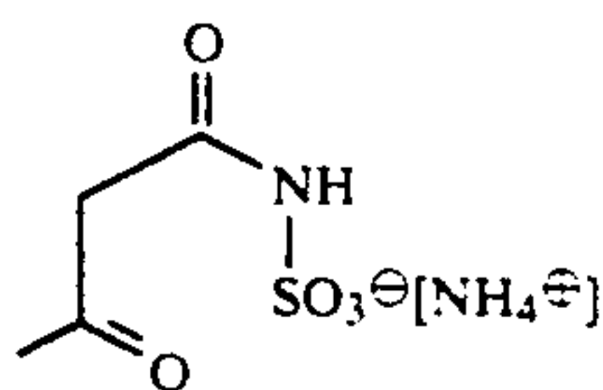
ammonium acetoacetamide-N-sulfonate
