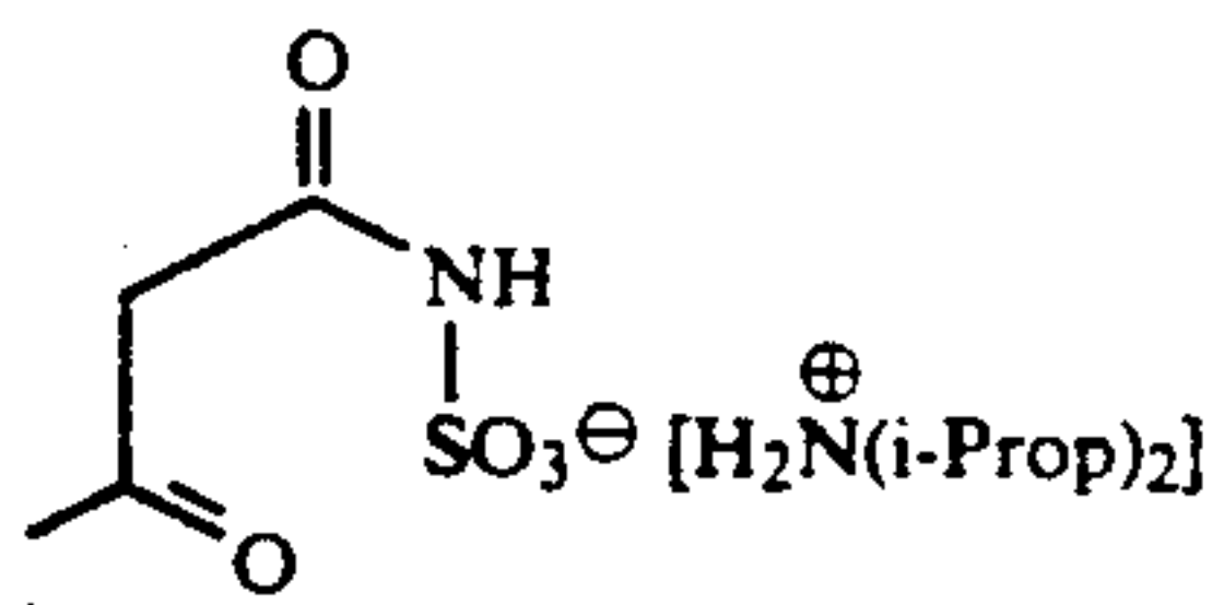
diisopropylammonium acetoacetamide-N-sulfonate
