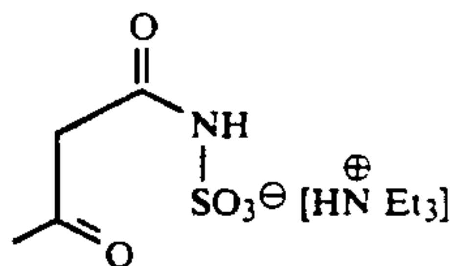
triethylammonium acetoacetamide-N-sulfonate
