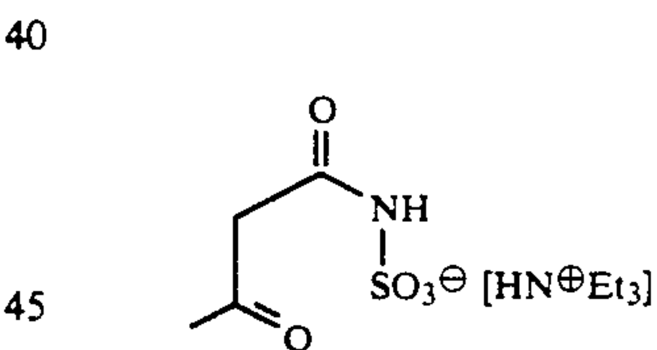
triethylammonium acetoacetamide-N-sulfonate
