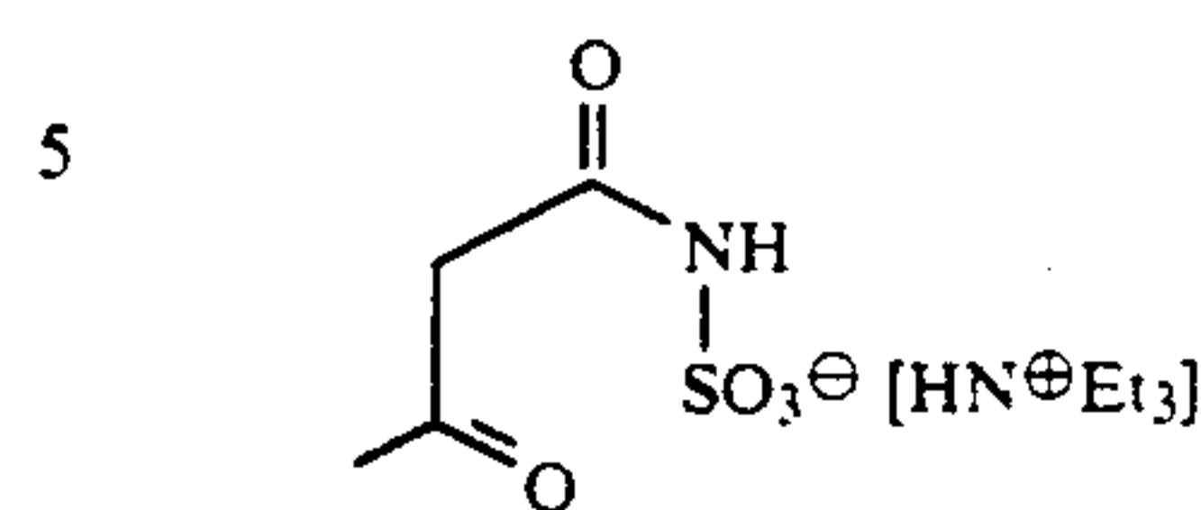
triethylammonium acetoacetamide-N-sulfonate
