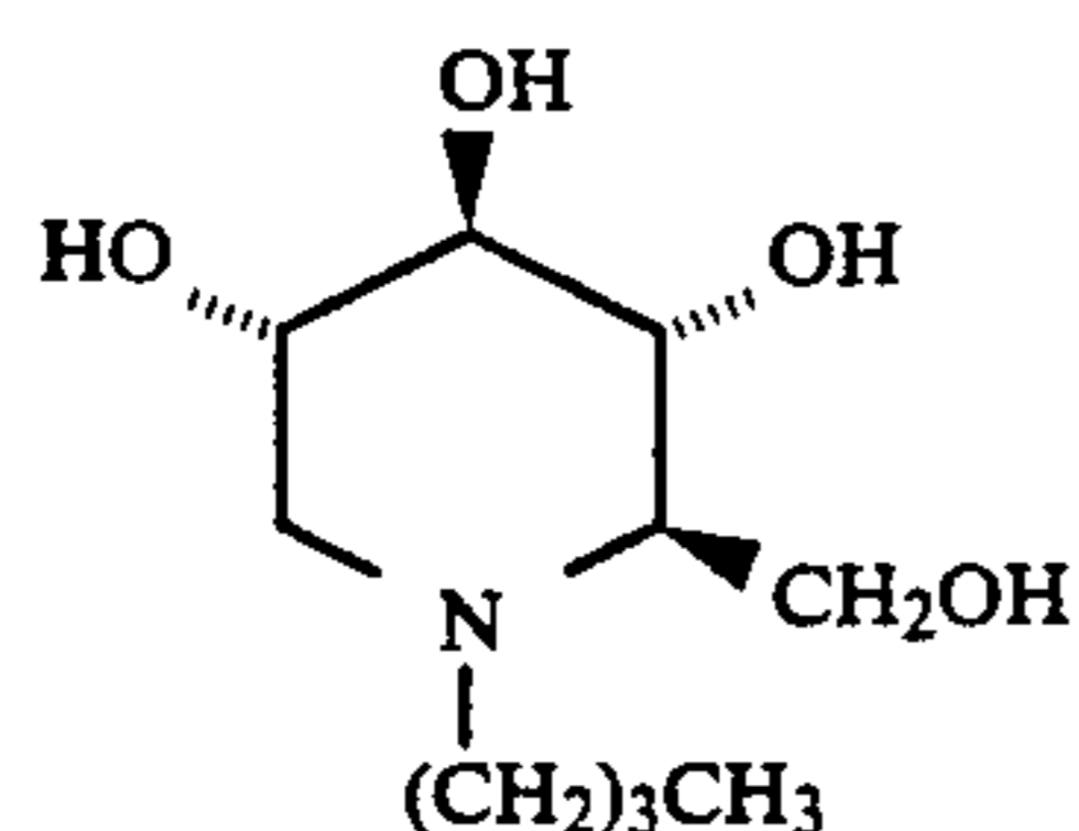
N-Bu-DNJ
