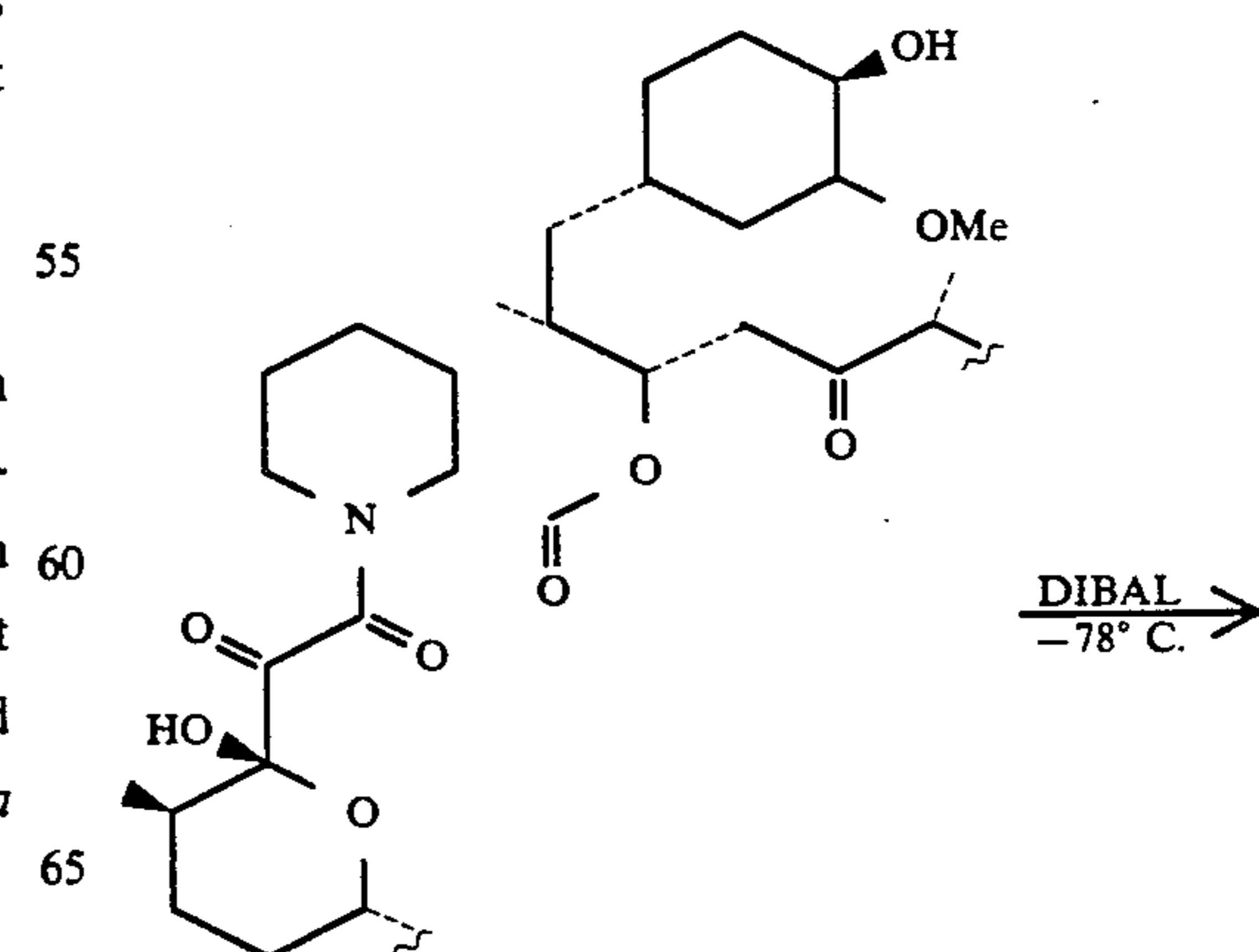
Scheme A. Reduction of rapamycin at position 15
