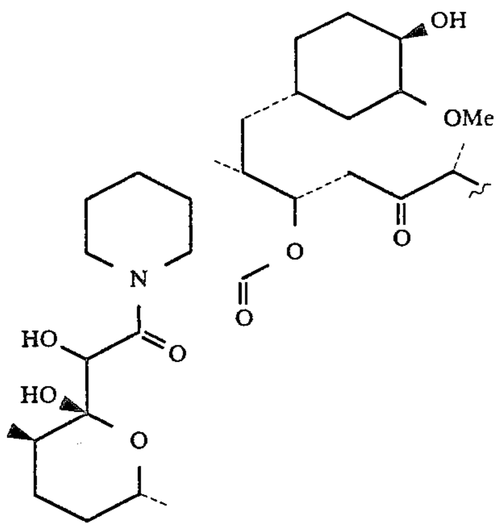
Scheme A. Reduction of rapamycin at position 15
