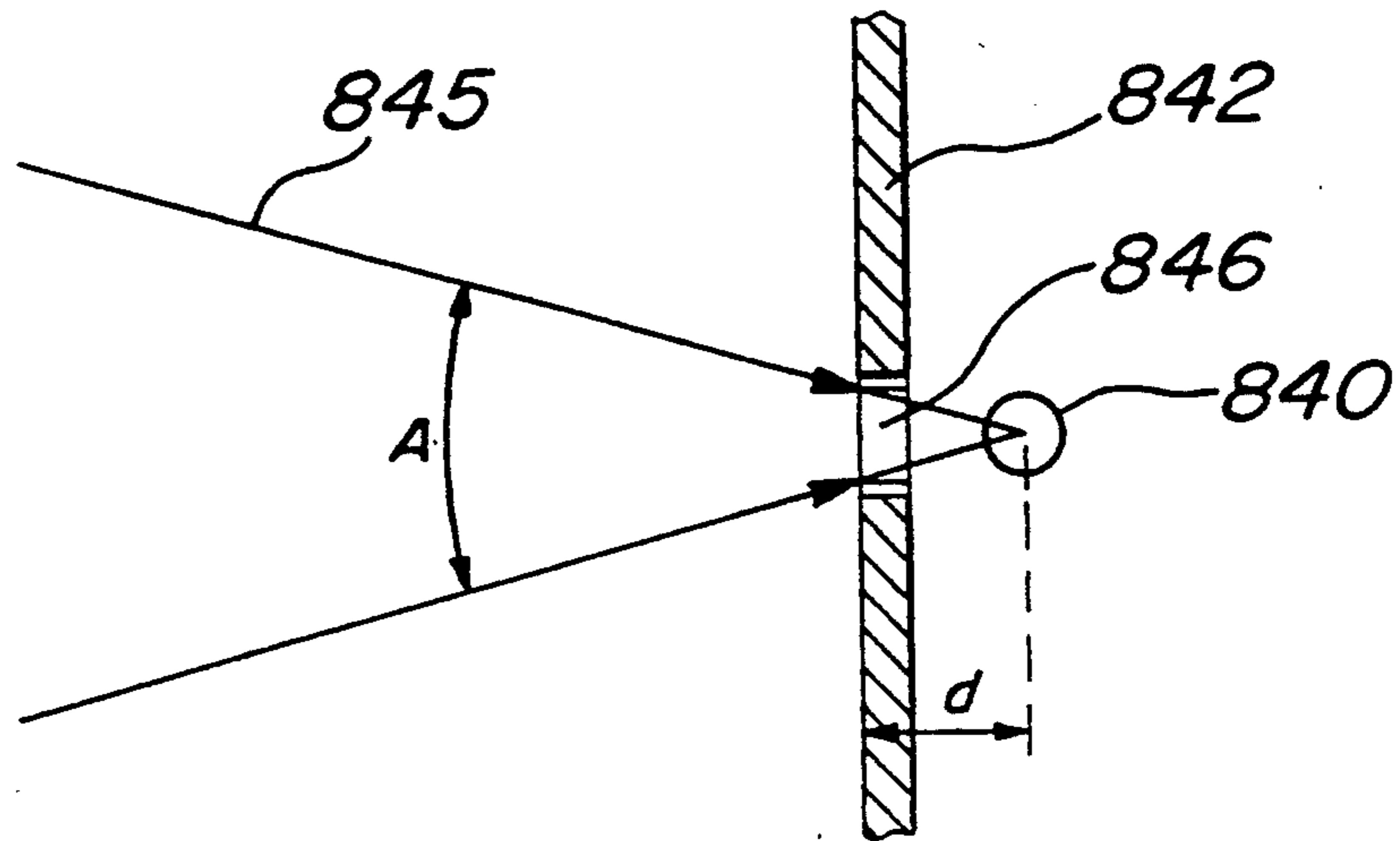
FIG. 16 (PRIOR ART)
