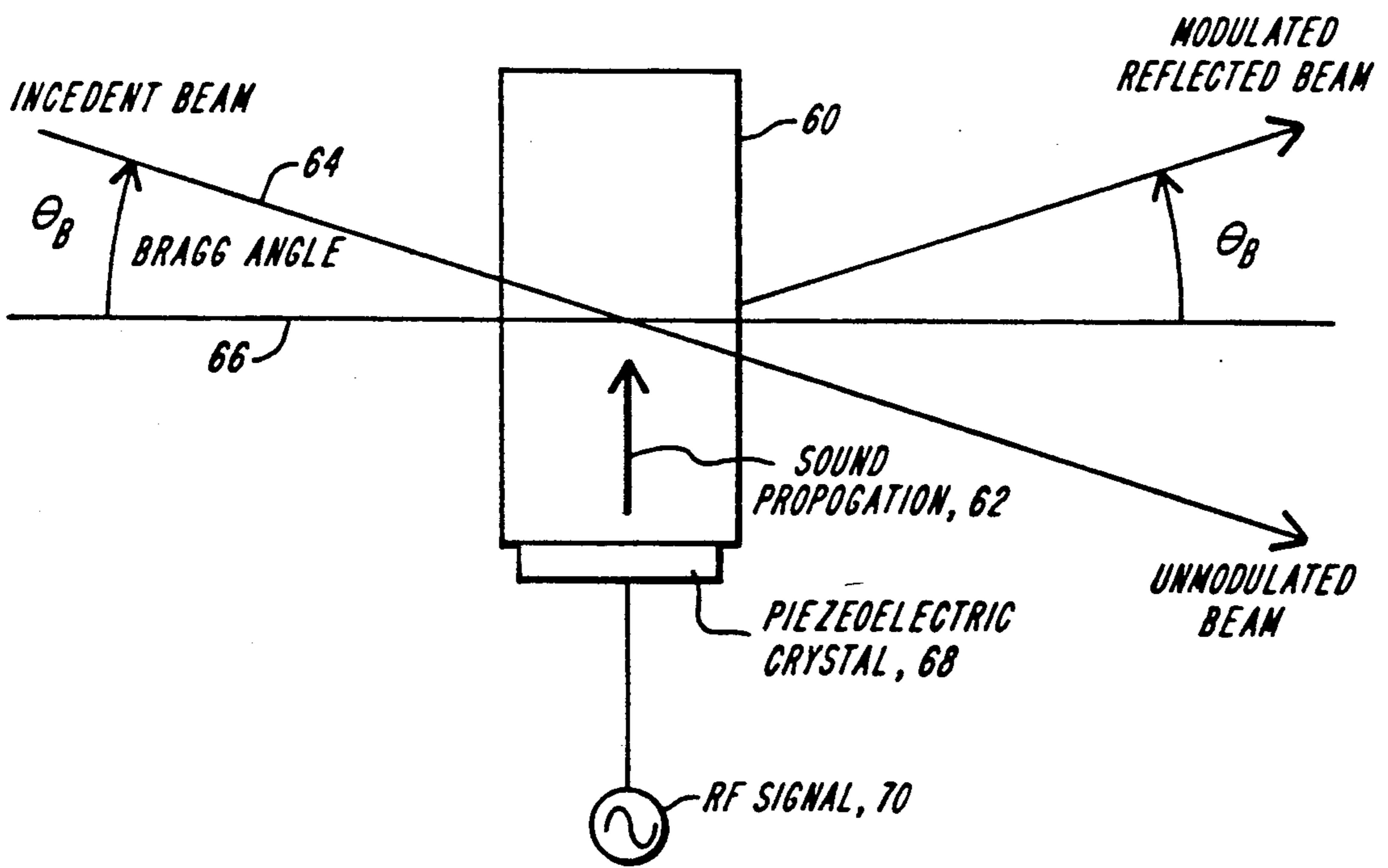
FIG. 2 (PRIOR ART)
