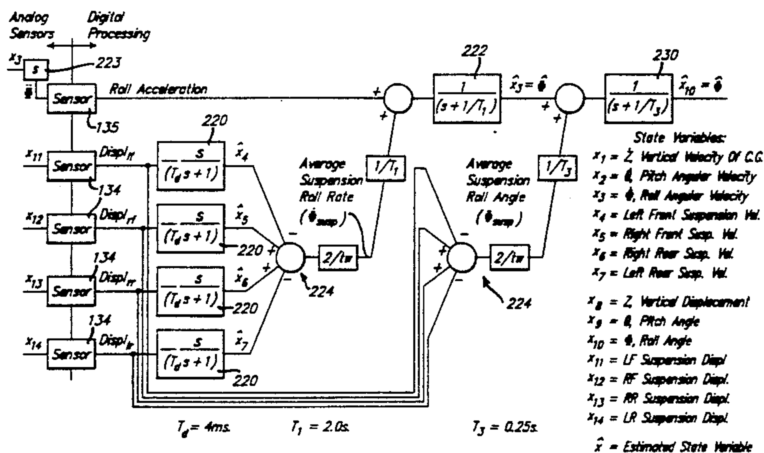
Principle Layout Of The Low Power Active Suspension Hardware
