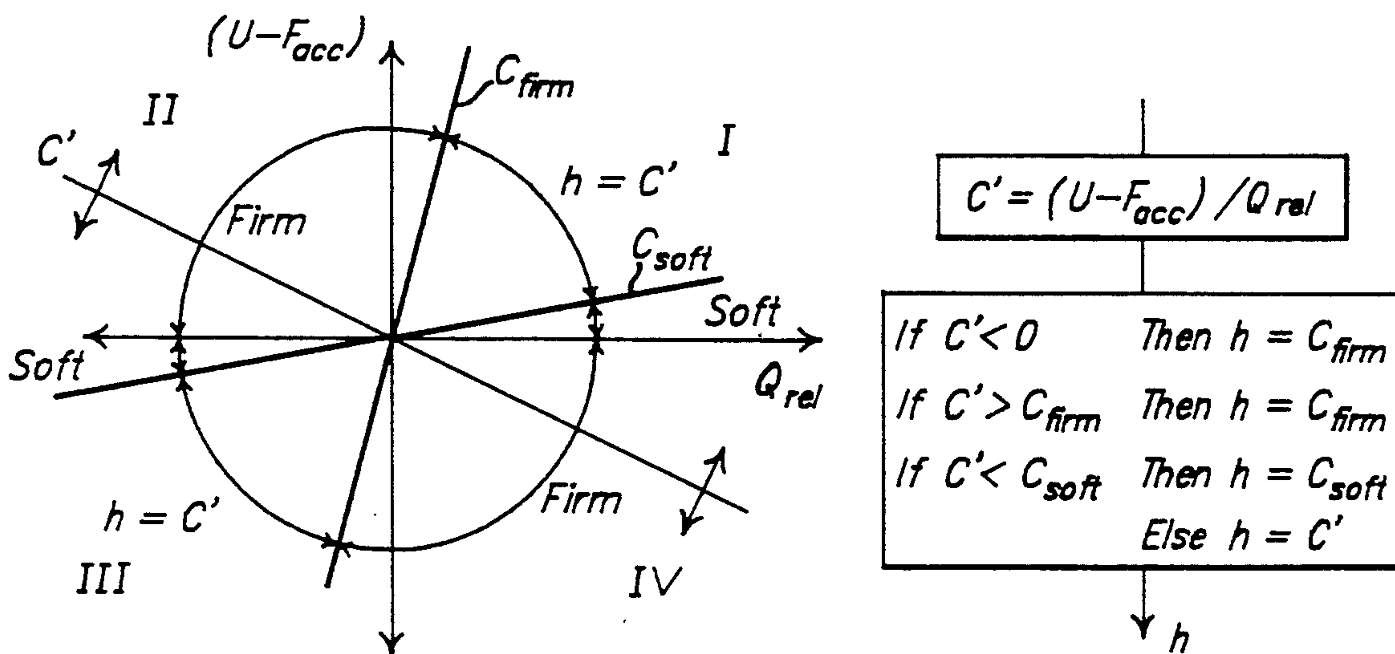
The Gain Adjustment Related To Requirement.
