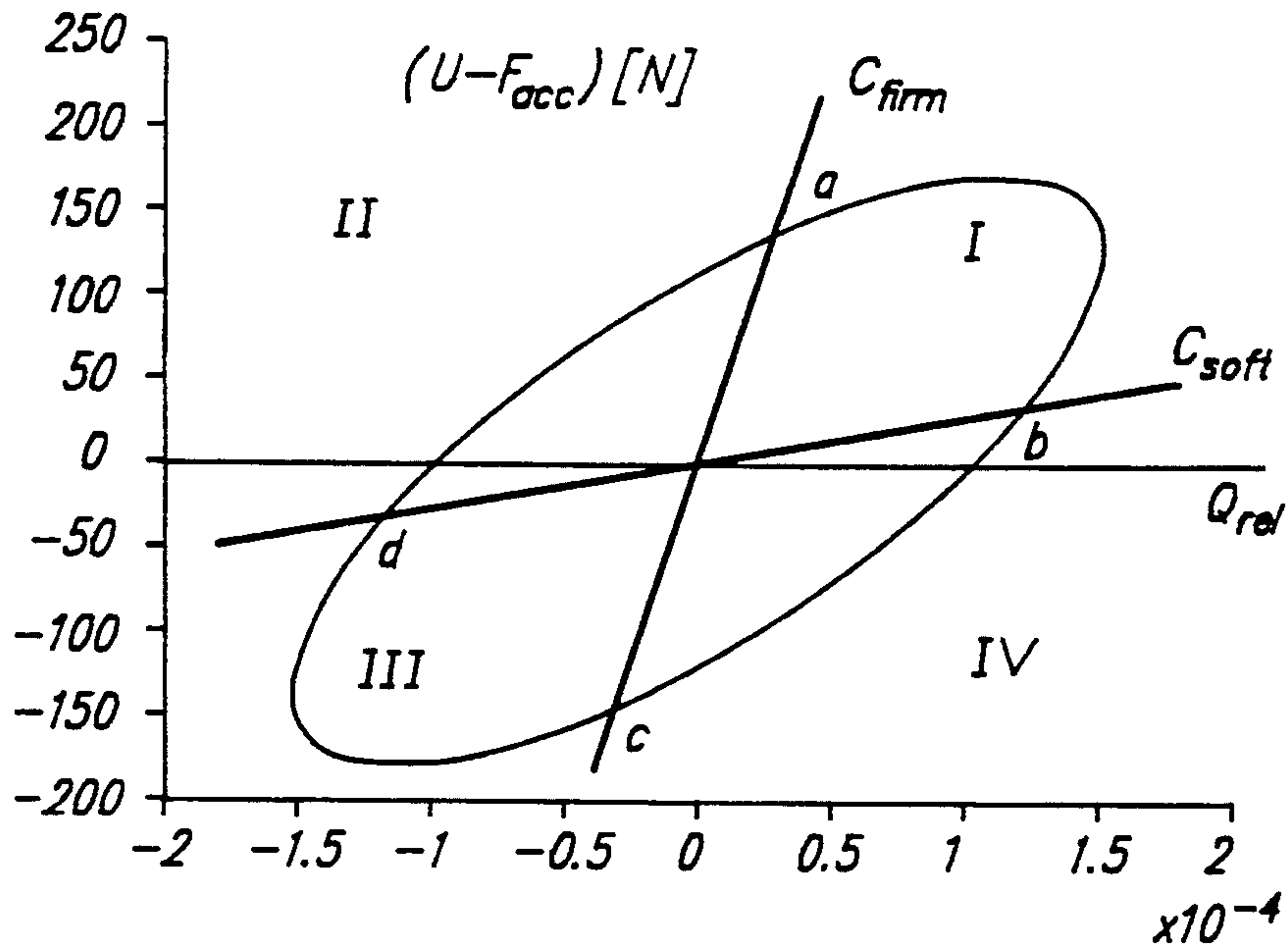
Piston Force (U-F_{acc}) Vs. Relative Flow Q_{rel} [ m^3/s ] At 2Hz Heave Road Input
