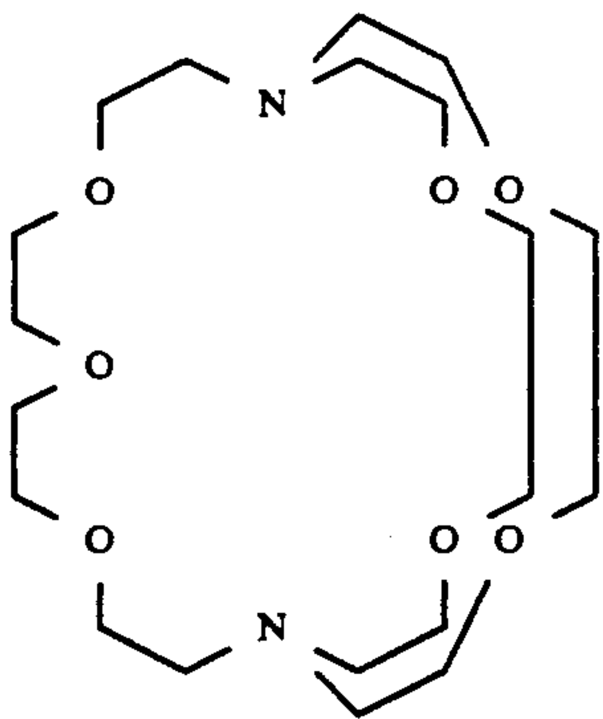
Chromogenic cryptand 3.2.2 is represented by
