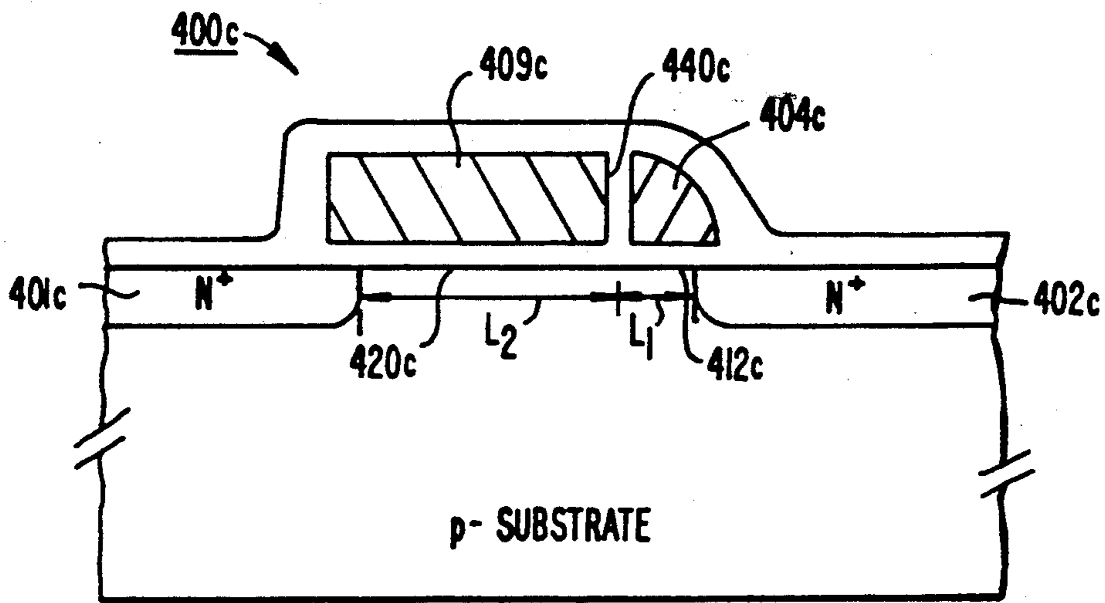
FIG. 4c. PRIOR ART
