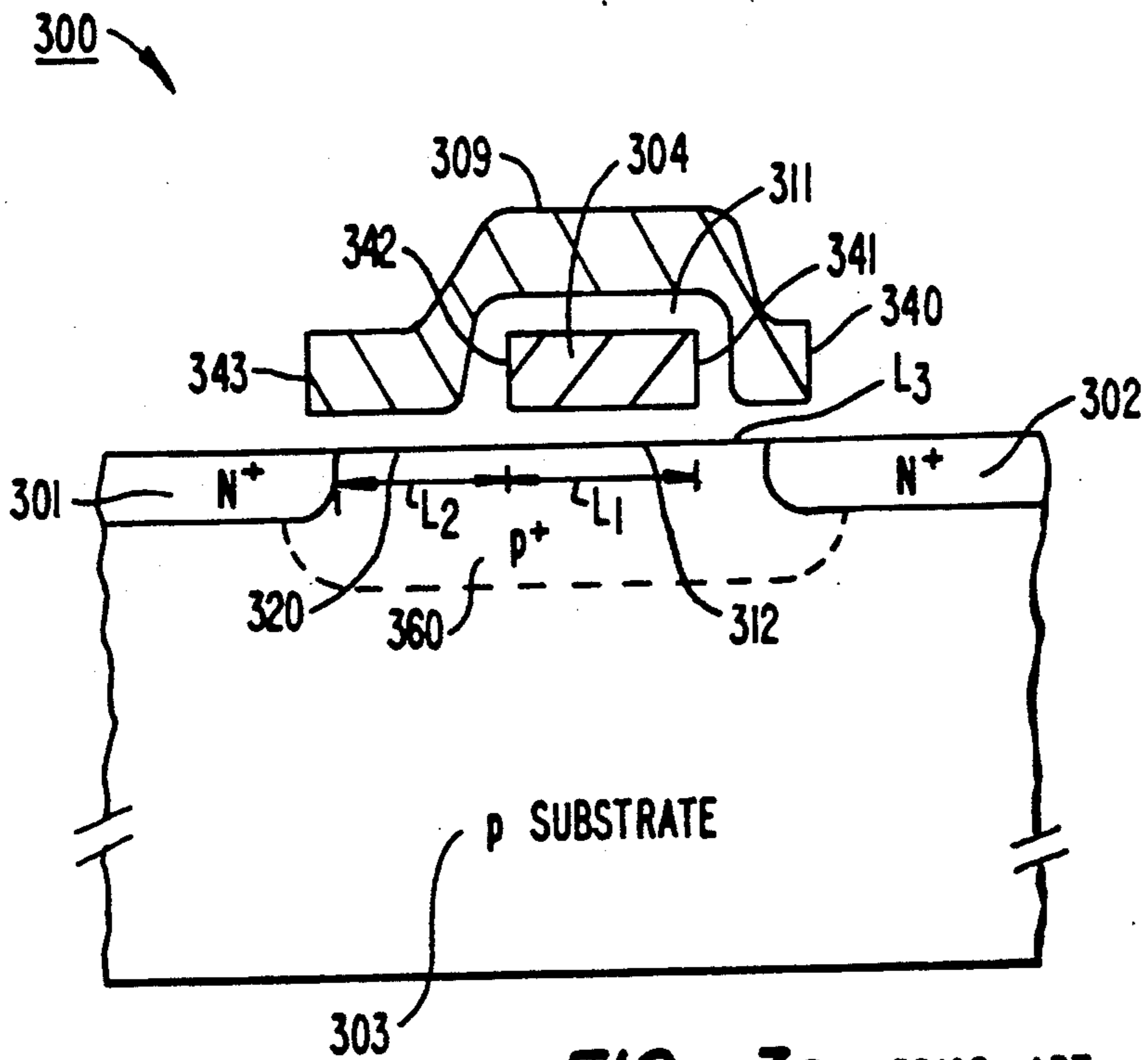
FIG. 3c. PRIOR ART
