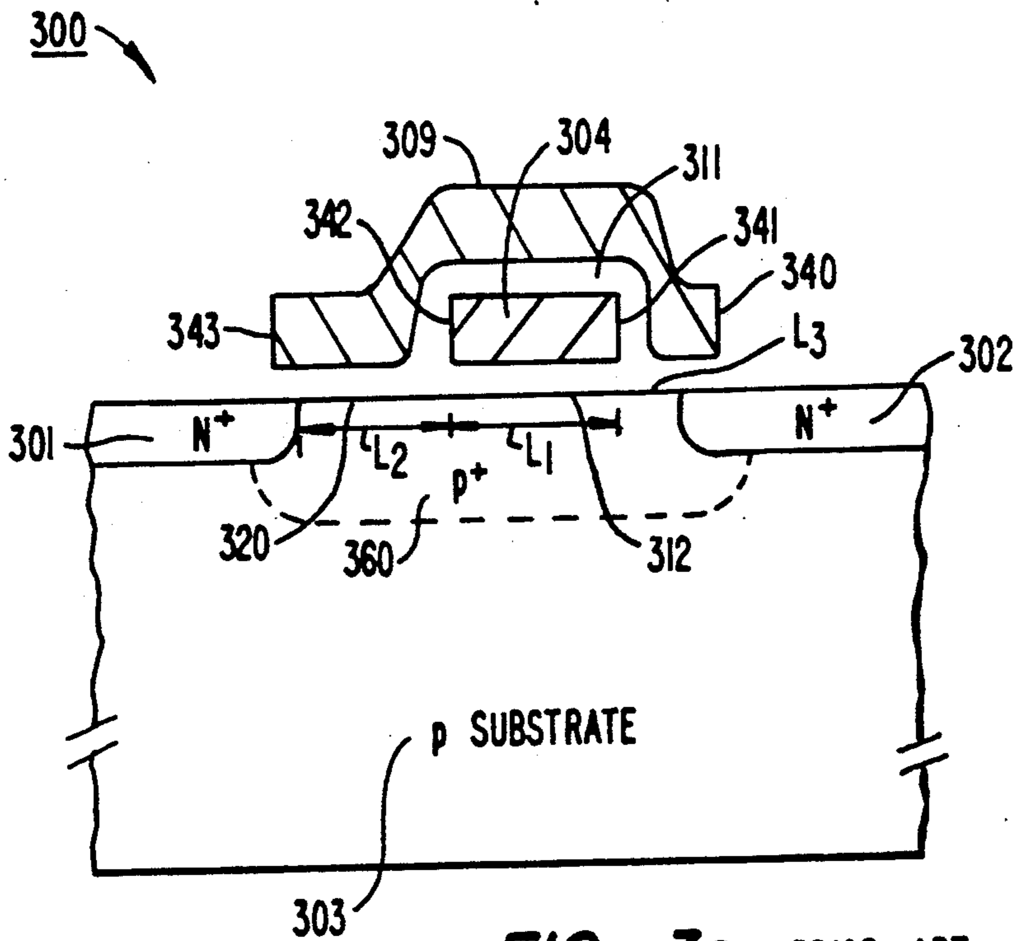
FIG. 3c. PRIOR ART
