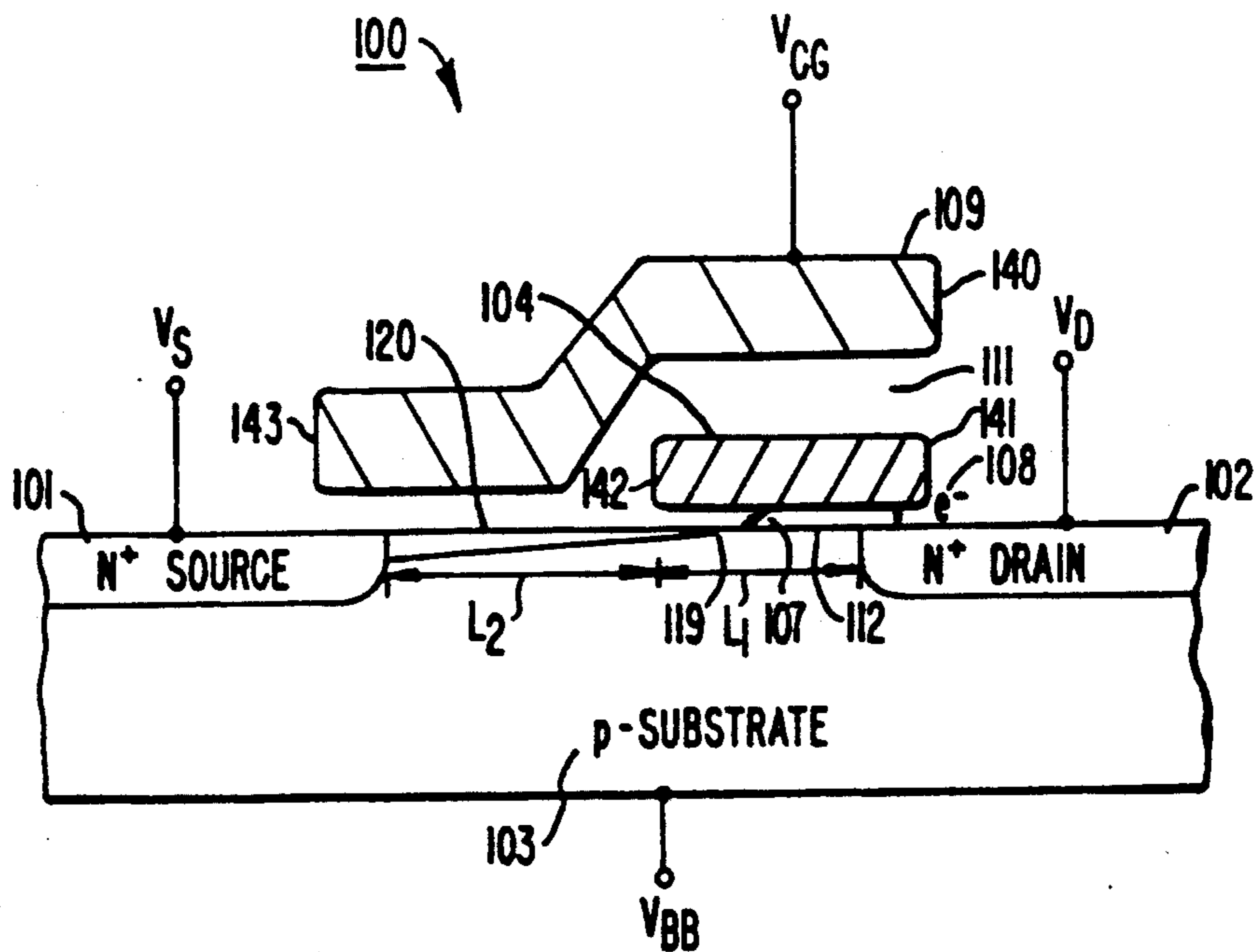
FIG. 1. PRIOR ART
