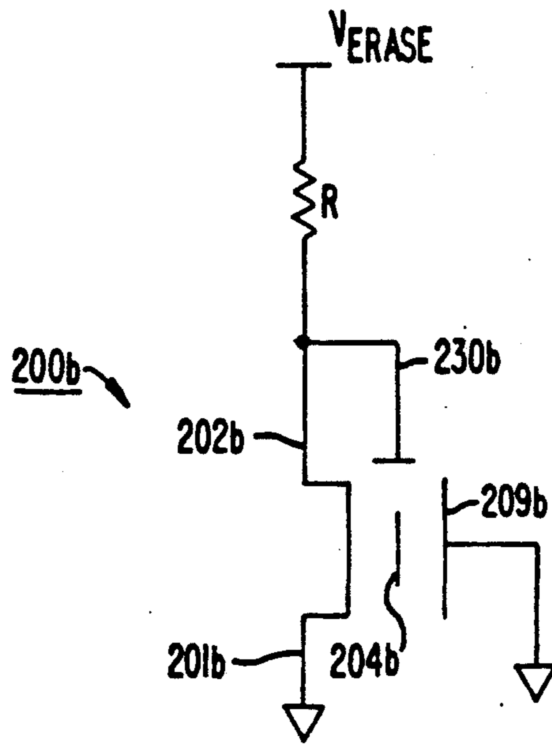
FIG. 2c. PRIOR ART
