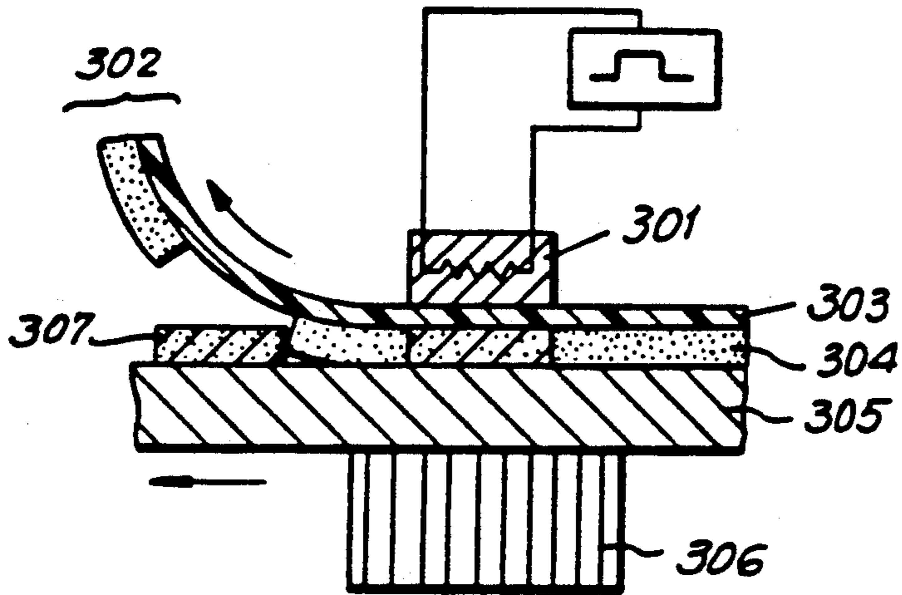
FIG. 1 PRIOR ART
