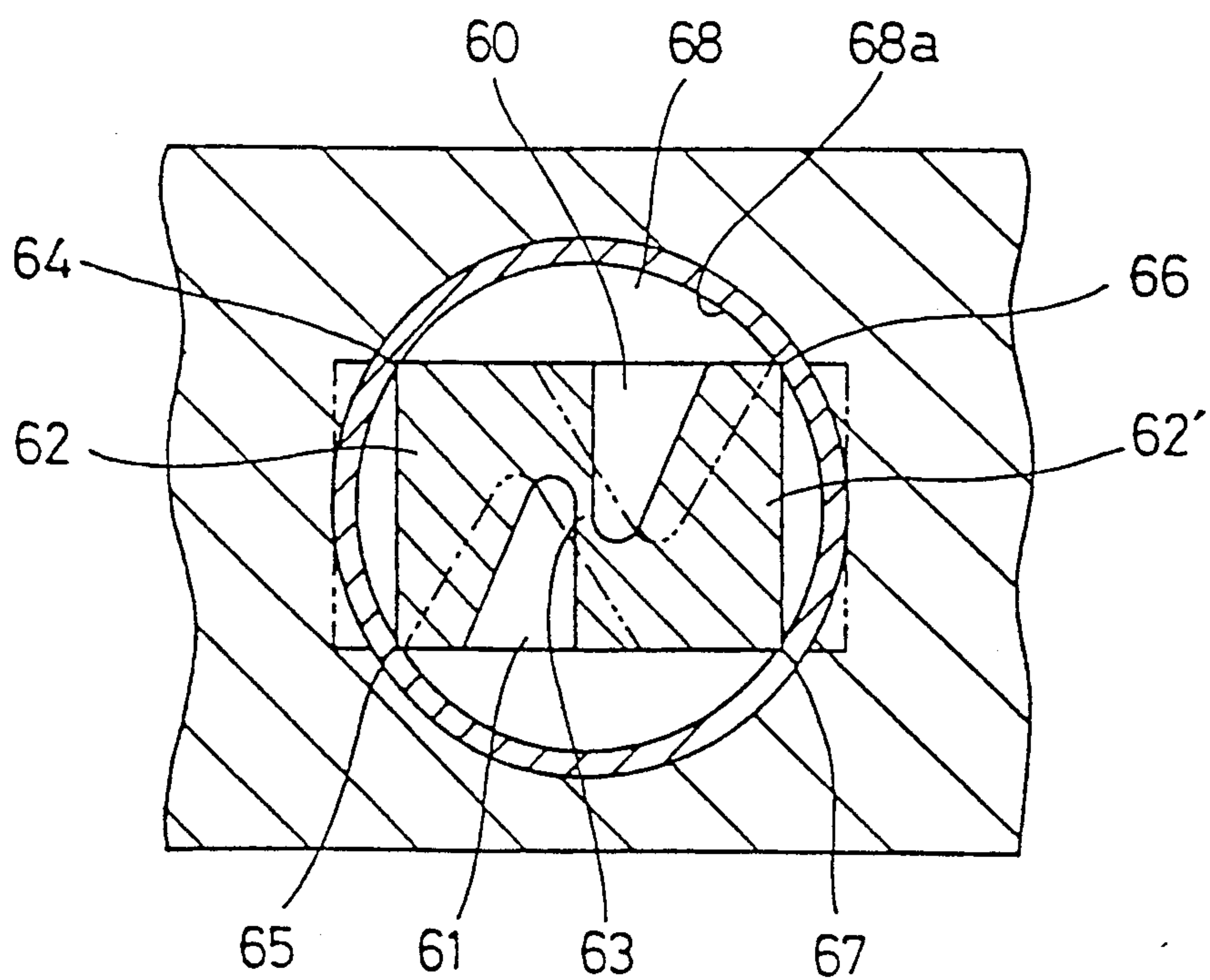
FIG. 19 PRIOR ART
