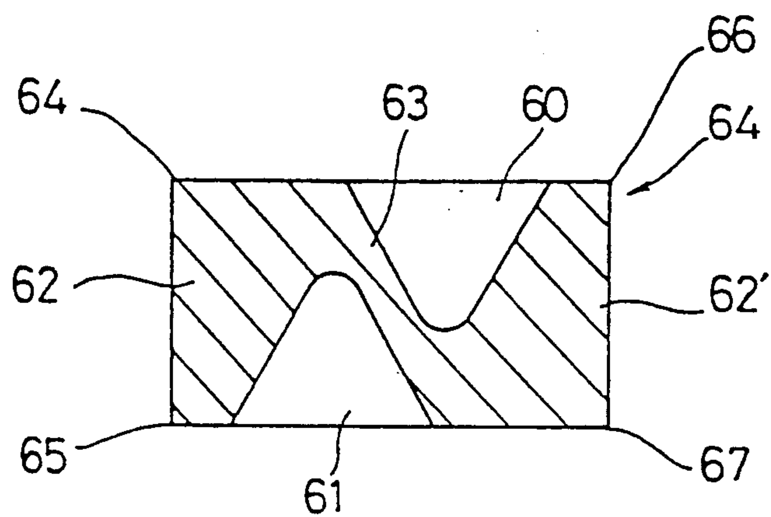
FIG. 18 PRIOR ART
