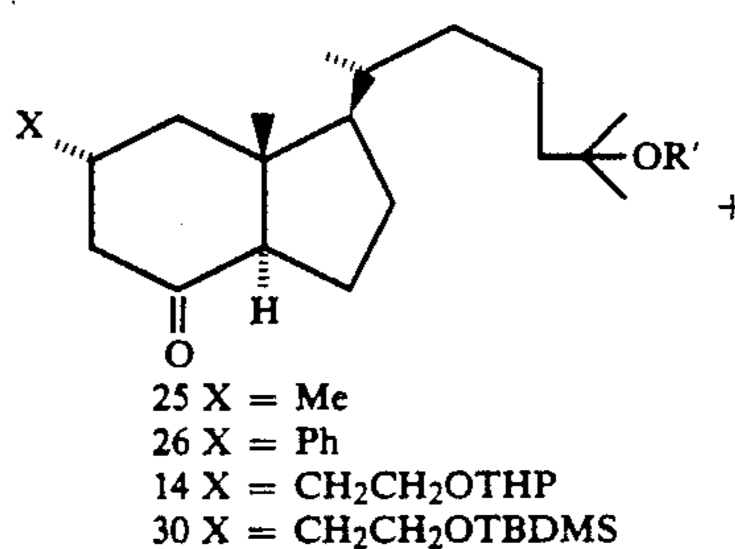
Scheme 4a
