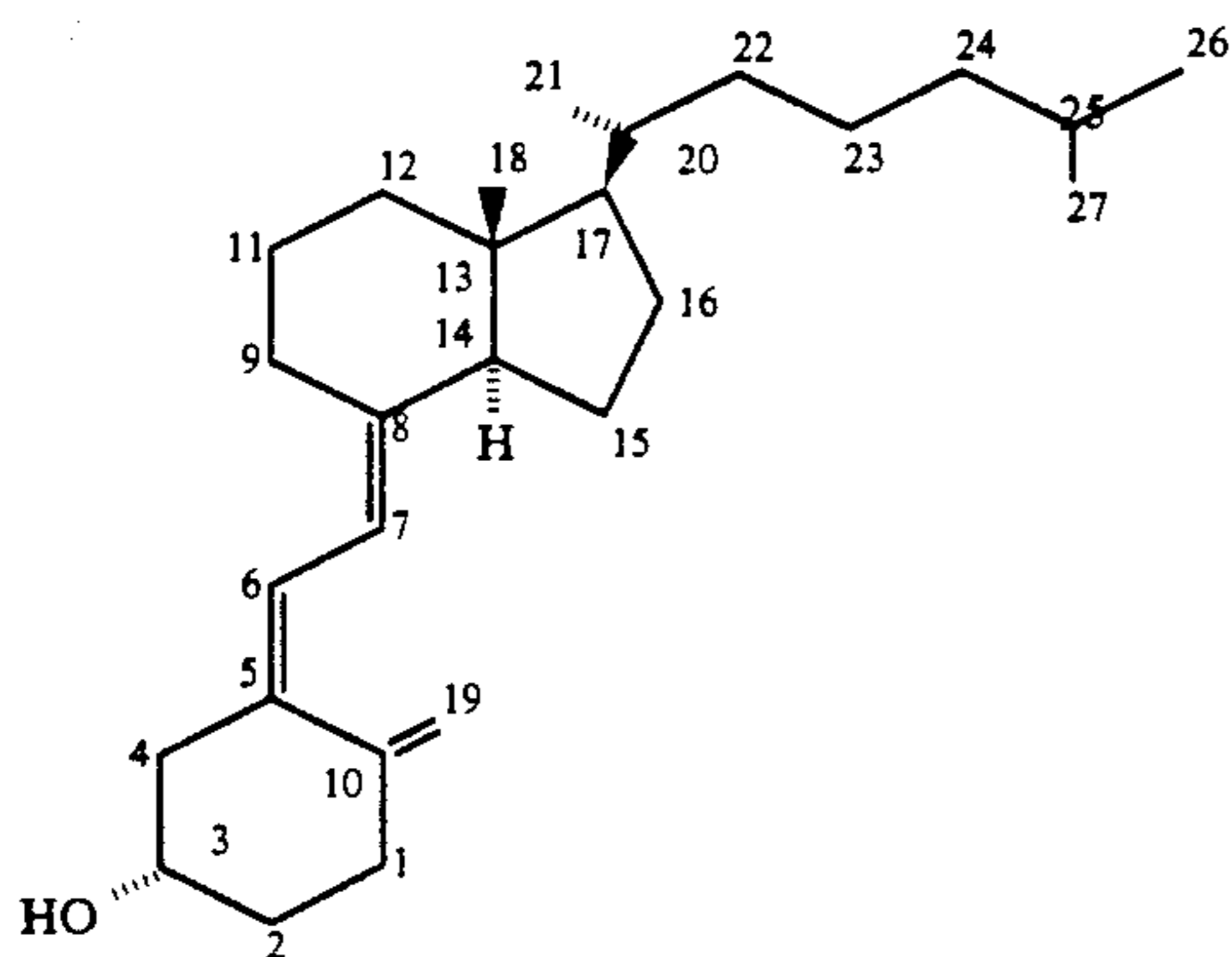
Vitamin D 3 or Cholecalciferol (9,10-seco-5,7,10(19)-cholestatrien-3β-ol)
