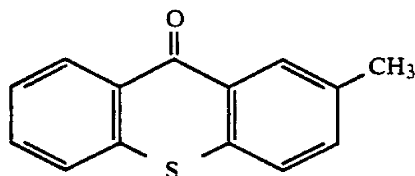
2-methyl thioxanthone
