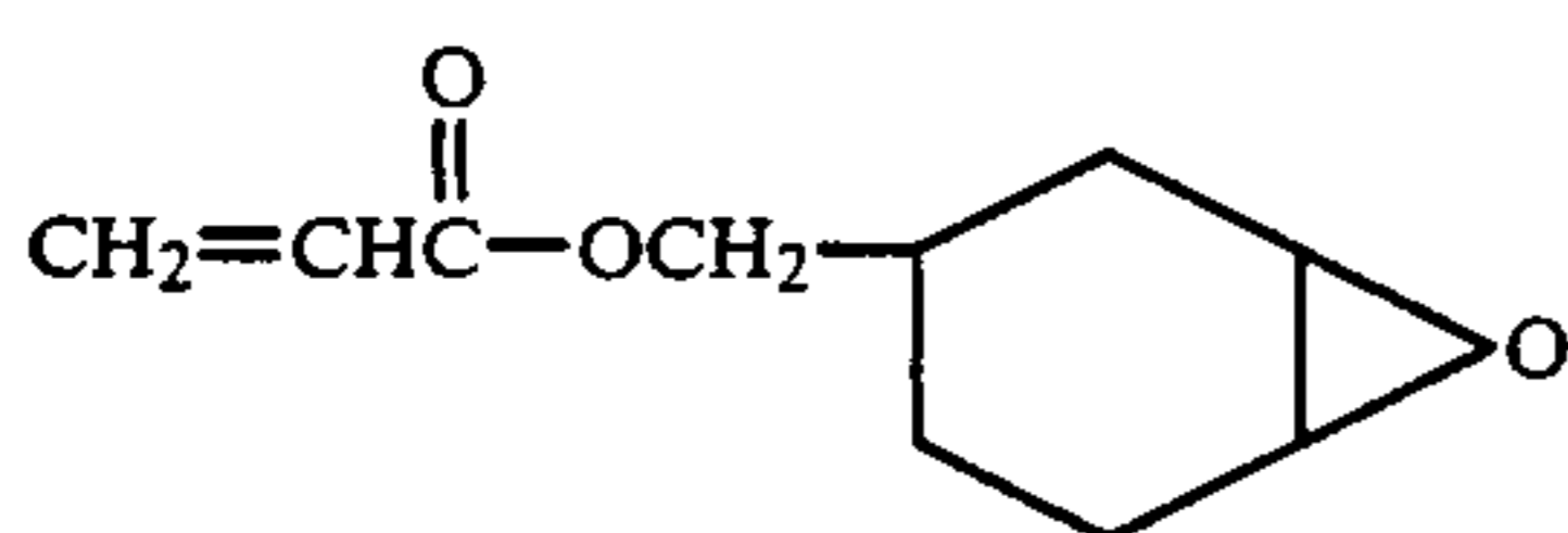
3,4-epoxycyclohexymethyl metacrylate
