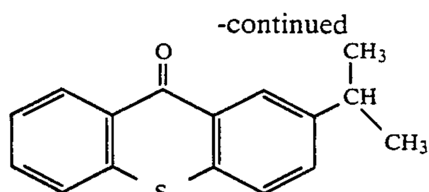
2-Isopropyl thioxanthone
