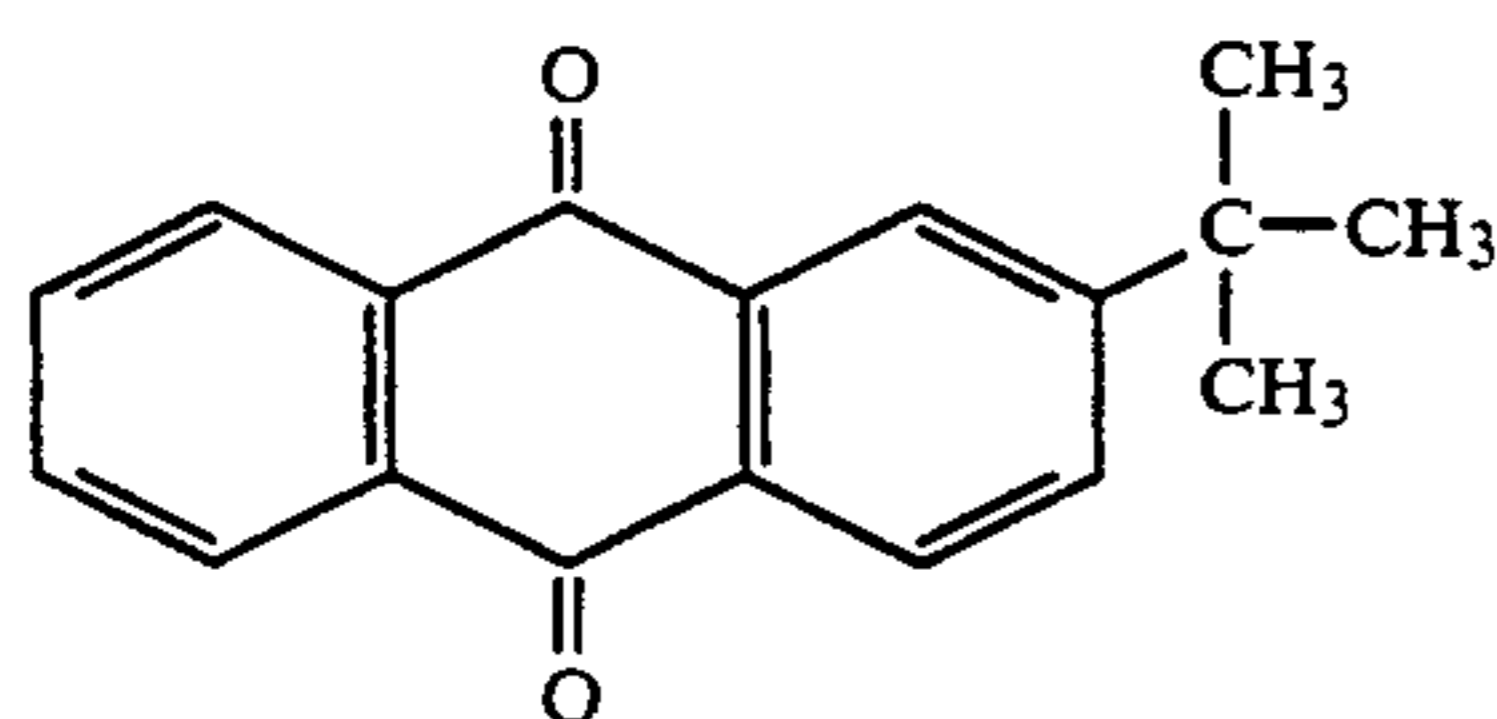
2-t-butyl anthraquinone
