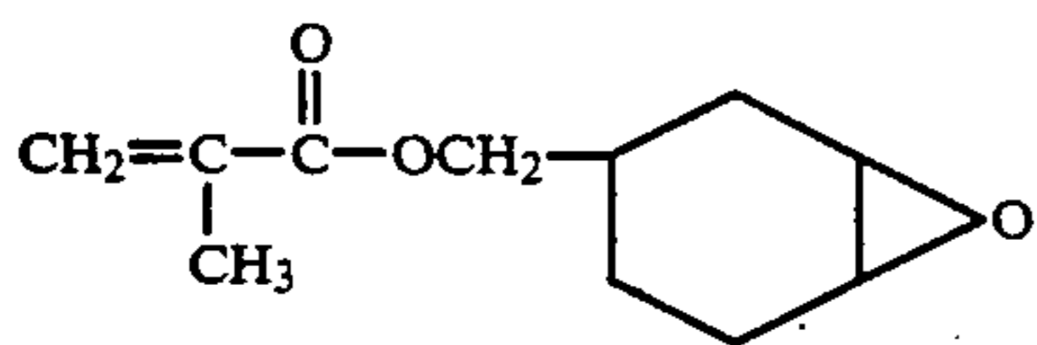
3,4-epoxycyclohexymethyl metacrylate
