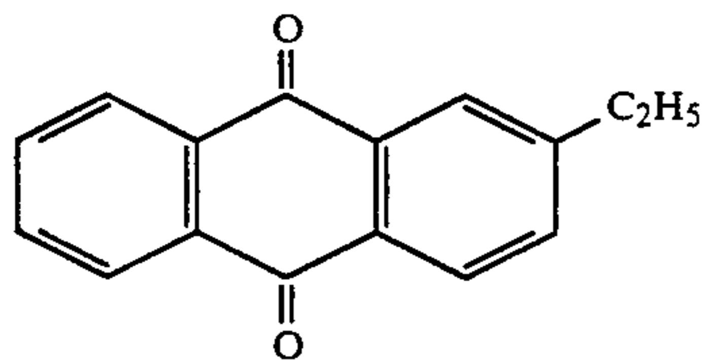
2-ethyl anthraquinone
