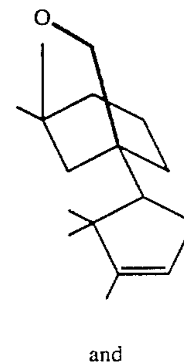
FIG. 9 is the NMR spectrum for the mixture of compounds having the structures:
