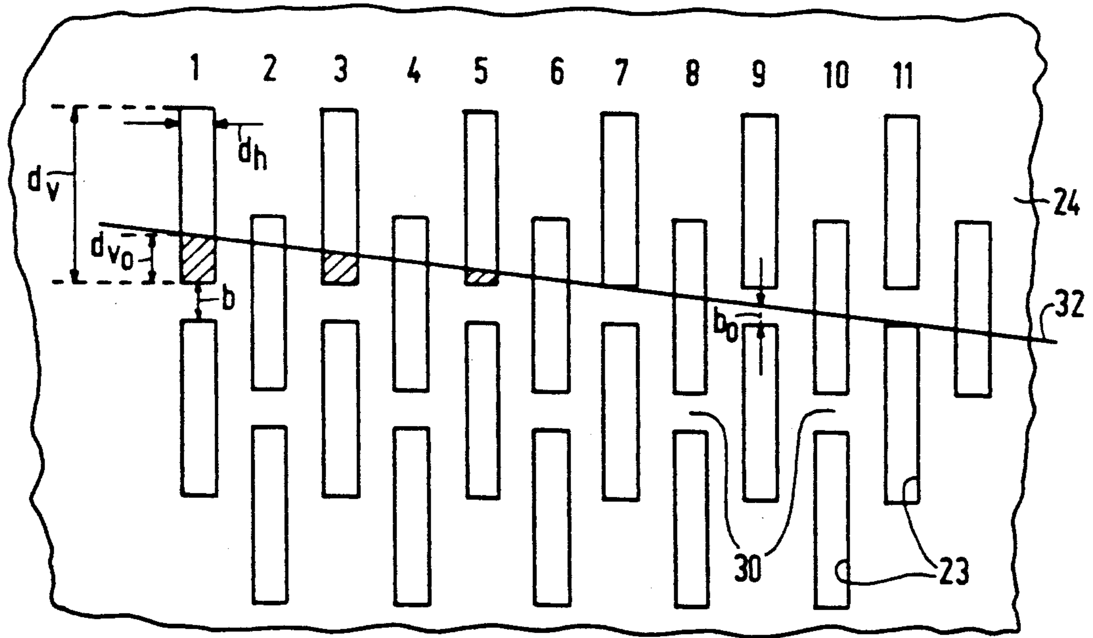
FIG. 2 PRIOR ART
