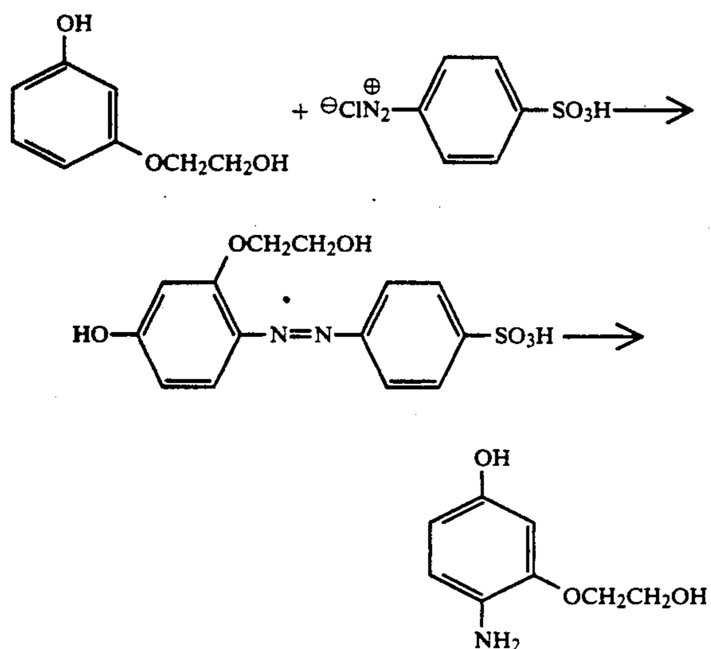
Reaction scheme 3
