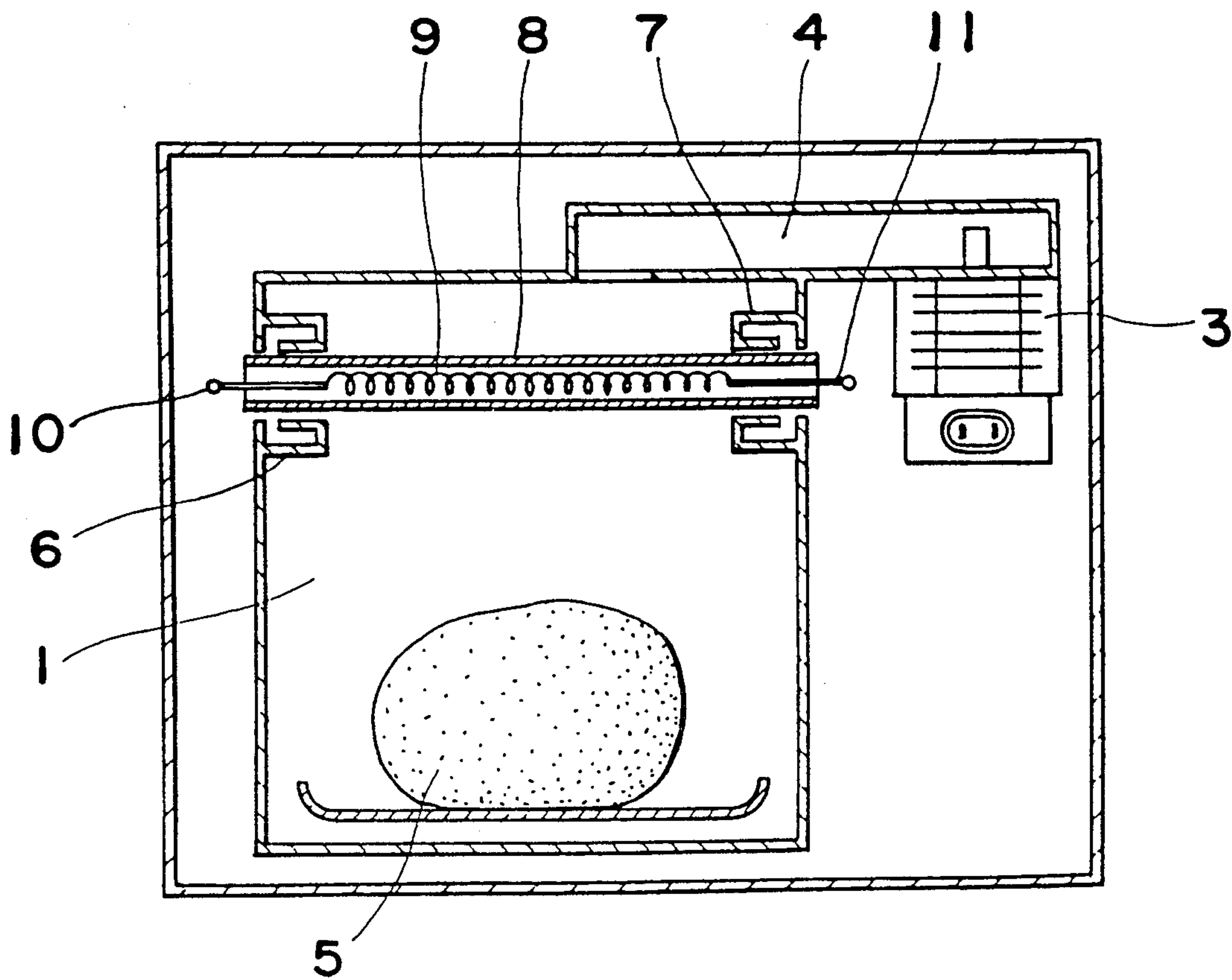
Fig. 2 PRIOR ART
